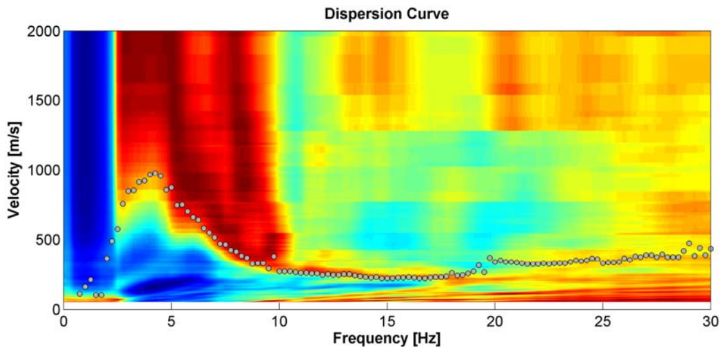
Figure 12: ReMi and ESAC analysis results comparison. ESAC phase velocities (gray dots).
