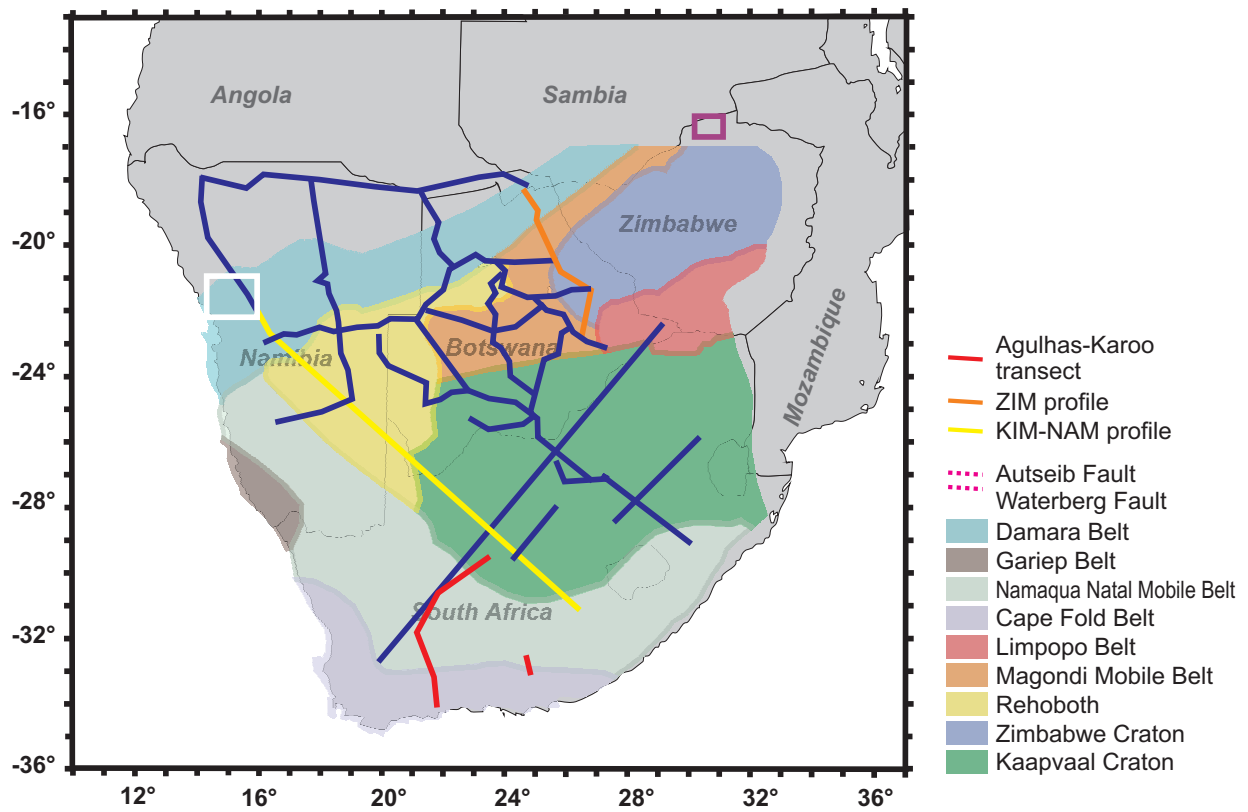
Fig. 3 Regional scale map of southern Africa showing major tectonic units discussed in the text. Black lines indicate MT profiles of the SAMTEX project (Evans et al. , 2011; Jones et al. , 2009; Muller et al. , 2009; Miensopust et al. , 2011) throughout Namibia, Botswana and South Africa. Red lines show high resolution MT profiles of the Inkaba yeAfrica project (de Wit and Horsfield, 2006; Weckmann et al. , 2007a,b). A yellow rectangle outlines the region of MT experiments in the Lower Zambezi valley basins by Bailey et al. (2000b,a); Whaler and Zengeni (1993) and Losecke et al. (1988). A white rectangle shows the area in which a regional (200km) and a local MT experiment (20kmx20km) were conducted by Ritter et al. (2003b) and Weckmann et al. (2003b)
