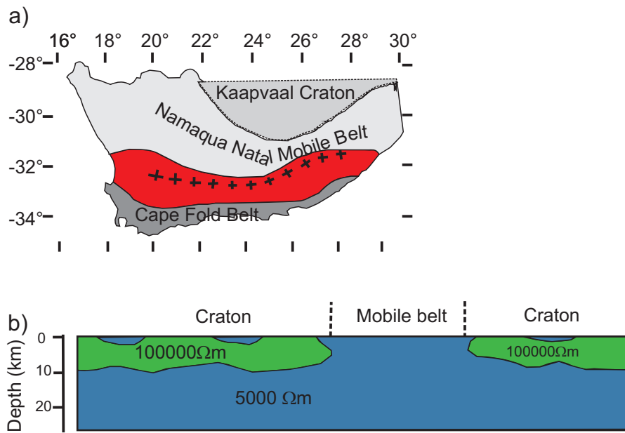
Fig. 2 Summarizing some of the early geo-electric and magnetic results which led to the postulation of the Southern Cape Conductive Belt (SCCB) and a generalized description of the characteristic properties of mobile belts and cratons. a) Map showing prominent tectonic units in Southern Africa together with location of the maximum of the Beattie Magnetic Anomaly (BMA (line of crosses), Beattie , 1909) and the SCCB (red colour) as derived from magnetometer array measurements modified after de Beer and Gough (1980). b) Proposed fundamental properties of cratons and mobile belts as derived from both deep geo-electric and magnetometer array measurements modified after van Zijl (1977a).
