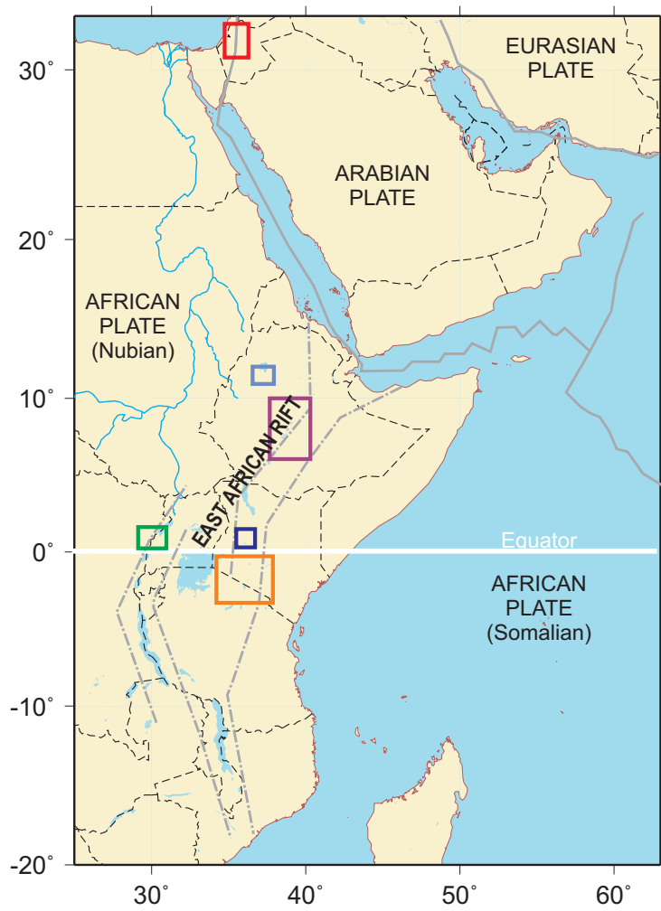
Fig. 7 Tectonic setting of the eastern African plate. Rectangles indicate the location of recent MT studies discussed in detail in the text. Red: DESERT and DESIRE projects across the Dead Sea Transform (Ritter et al. , 2003a; Meqbel et al. , 2008, see also Fig. 9). Dark blue: Baringo Rift basin, Kenya (Hautot et al. , 2000). Light blue: Mesozoic basin structure beneath the Lake Tana area, Ethiopia (Hautot et al. , 2006). Green: Western Branch of the East African Rift, Uganda (Häuserer and Junge, 2011, Riftlink). Lilac: Ethiopia Afar Geoscientific Lithospheric Experiment, Ethiopia (Whaler and Hautot, 2006, EAGLE). Orange: KRISP-94 project, Kenya (Simpson et al. , 1997; Sakkas et al. , 2002)
