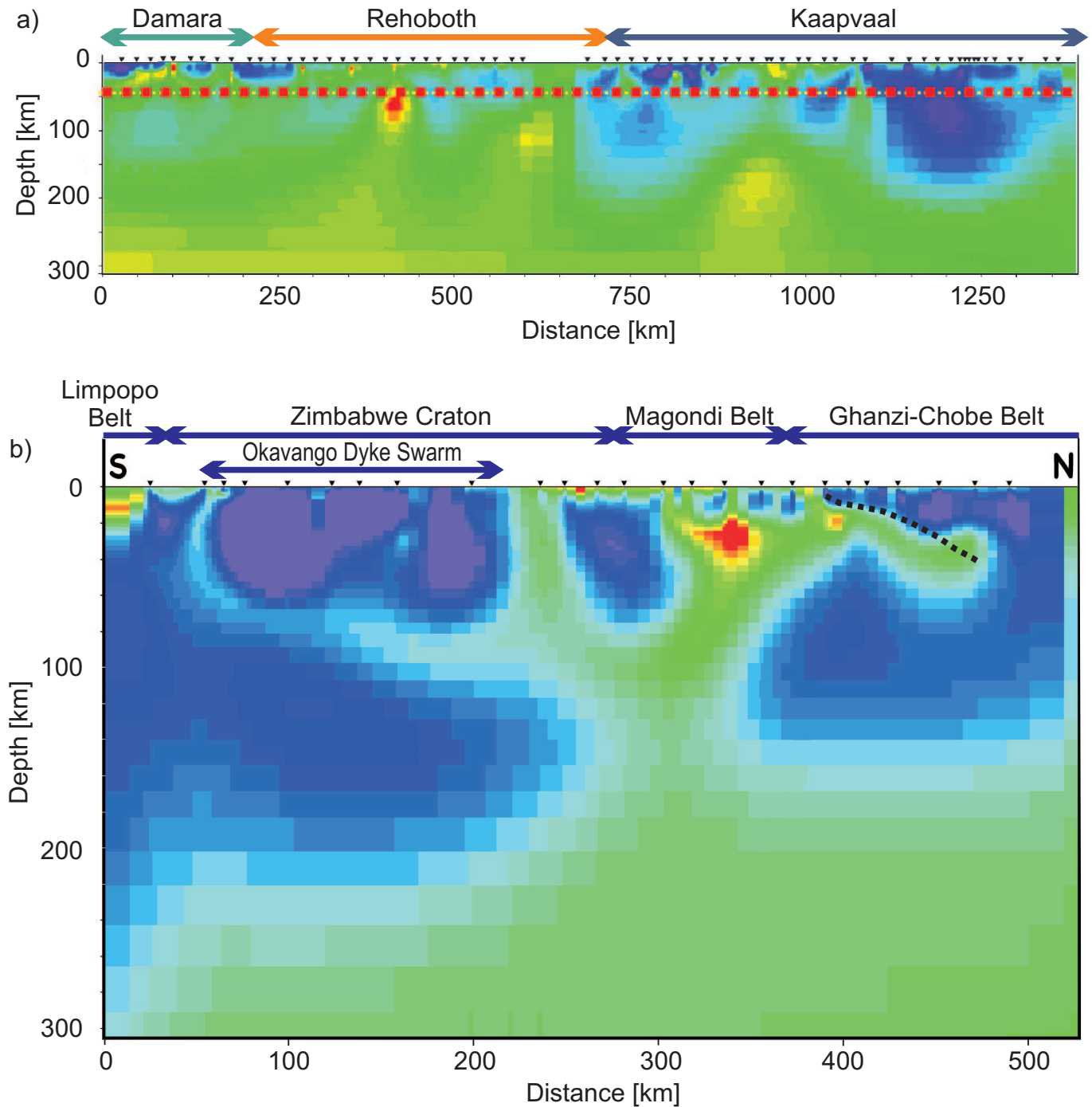
Fig. 4 Two-dimensional electrical resistivity models for a) the KIM-NAM and b) ZIM profiles derived from 2D inversion modified after Muller et al. (2009) and Miensopust et al. (2011) . Zones of low electrical resistivity are shown in red, zones of high resistivity (or low conductivity) in blue colours. The surface extent of the respective geological units is indicated by arrows above the resistivity sections. Both profiles run in southeast-northwest direction, but they are separated by more than 500km. In both models, the cratonic terranes exhibit resistive and thus cool and thick lithospheric root, while the mobile belts seem to be much more conductive correlating with hotter and thinner lithosphere. The red dashed line along the KIM-NAM profile (Fig. a) shows crustal thickness. The black dashed line in figure b) indicates the northward dipping boundary between the resistive Ghanzi-Chobe Belt to the north and the Magondi Belt to the south.
