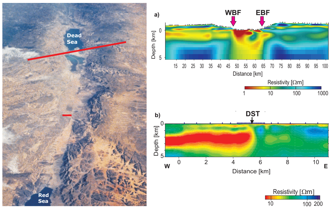
Fig. 9 The locations of the two profiles crossing the Dead Sea Transform are indicated on top of an aerial picture (left side). a) 2D inversion result of the main profile of the DESIRE data set (Meqbel et al. , 2008). In the upper 5 km several shallow conductivity anomalies can be observed which correlate well with sedimentary sequences known from existing boreholes. Beneath the Dead Sea (conductive Dead Sea brines imaged in dark red colours) in the center of the profile a vertical zone of higher conductivities is observed, flanked by higher resistivities (blue colours) beneath the eastern and western shoulders. The vertical boundary of this anomaly coincides with the location of the Eastern and Western boundary faults of the DST (EBF and WBF, respectively). b) 2D inversion result of the inner part of the DESERT profile (Ritter et al. , 2003a). The most prominent feature is the conductive half layer in 2 – 3.5 km depth, which is interpreted as the image of brines in a sedimentary layer. In this simple transform fault setting, the shallow DST appears to be a barrier for cross-fault fluid flow.
