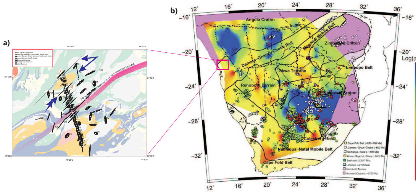
Fig. 5 a) Using current ellipses to image structural details of the MT data set across the Waterberg Fault / Omaruru Lineament (WF/OL) in Namibia (Weckmann et al. , 2003a). The length of an ellipse defines a measure of a nearby conductivity contrast, while the orientation shows the direction of preferred current flow. Parallel and elongated ellipses north of the WF/OL can only be explained by a 10km wide fault zone showing internal electrical anisotropy parallel to the fault. Extremely elongated ellipses (marked with a blue arrow) image a shallow, very conductive ring structure of graphite bearing marbles. b) Application of an imaging method to the SAMTEX data set (Jones et al. , 2009). This approach is based on the maximum resistivity values for a depth of 200km using the Niblett-Bostick transformation (e.g. Niblett and Sayn-Wittgenstein, 1960; Bostick, 1977). Coloured circles on top show kimberlite locations (red \hat{=} diamondiferous, green \hat{=} non-diamondiferous, and white \hat{=} not defined or unknown). Black dots indicate site locations. Zones of high resistivity (blue) correlate with cratonic mantle lithosphere. The occurrence of diamondiferous kimberlites seem to be mostly confined to the craton boundaries.
