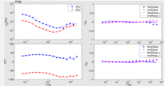
Fig. 5: Apparent resistivity and phase curves for off-diagonal impedances at site P06 and tipper function for Parinacota volcano. The general fit is satisfying, except at longest periods.
