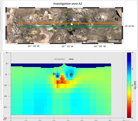
Fig. 4: 3-D inversion model of volcano Parinacota (RMS = 1.43) after 134 iteration with a background resistivity of 100 \Omega m. Well conductive feature (A) with an apparent resistivity of 1 \Omega m beneath volcano Parinacota. Higher resistive structure (B) in the subsurface around the volcano conical. The green array delimits the profile which is illustrated in the image above.
