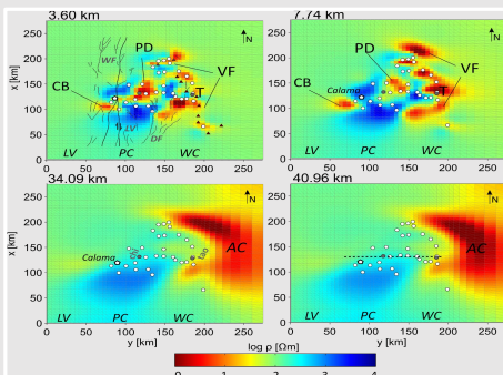
Fig. 7: Preferred 3-D model (RMS=2.09, 132 iterations) of investigation area B in plan view at different depth. The final data set consist of 32 sites located in the Precordillera (PC), the Western Cordillera (WC) and the Preandean Depression (PD). For the 3D inversion with the ModEM 3-D algorithm, the impedance tensor and vertical transfer function elements were smoothed and interpolated using an Akima function. Background resistivity was set to 100 \Omega m. AC-Altiplano Conductivity Anomaly; VF-Conductor that belongs to the volcanic arc; T-conductor correlating with the El Tatio Geysers; CB-conductive sediments of the Calama Basin. Grey dots: Data example. Triangles represent the location of the volcanoes. Upper left: solid lines indicate main faults of the study area (WF-West Fissure; LV-Limon Verde; DF-DF-Domeyko Fault). Lower right: dotted line illustrates cross section of the resistivity distribution with depth.
