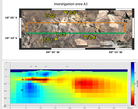
Fig. 2: 3-D inversion model of volcano Taapaca (RMS = 1.043) after 109 iteration with a background resistivity of 100 \Omega m. Important feature (A) may indicate the magma chamber of Taapaca volcano at a depth of 6-8 kilometer, as a possible good conductor is found. The topography of the area is observable, the air is illustrated in dark blue cells and separates from the conductive features of the subsurface. Two resistive feature are resolved at (B) and (C). Feature (D) remains uncertain and requires a sensitivity study to confirm its existence. Satellite image taken from Google Earth shows the area of the profile with stations. The orange line illustrates the array of the inversion model cut. It is a result of the cell size of the initial model. The green line indicates the front-side of the profile shown.
