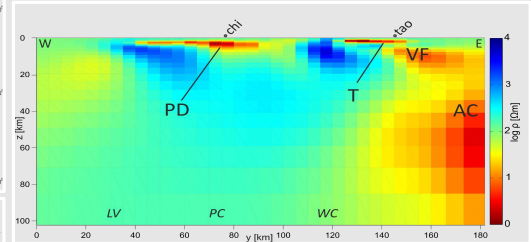
Fig. 6: Resistivity distribution along depth (RMS=2.09) of the preferred model at around 22.5°S in study area A. AC-Altiplano conductor; VF-Conductor that belongs to the Volcanic arc; T-conductor correlating with the El Tatio Geysers. Grey dots: MT Sites closest to the selected section and shown in Fig. 4.
