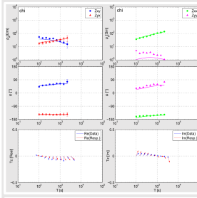
Fig. 6: Apparent resistivity, phase and tipper at sites tao and chi with an RMS= 2.09. Derived from the off-diagonal (left) and the main diagonal (right) elements of the impedance tensor Z and tipper. Solid lines represent the response after the inversion with ModEM. It turned out that the 3-D model with a covariance set to 0.2 and tipper set to an error floor of 0.03 (impedance tensor set to an error floor of 0.05) fits the data best.
