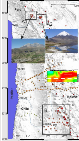
Fig. 1: Map of the investigation areas in Northern Chile. Stars mark the magnetotelluric (MT) sites in this area. Rectangles A1 and A2 (at ~18°S) and B (at ~22.5°S) are areas for which 3-D modeling with the ModEM 3D inversion algorithm was performed. The dotted lines indicates the location of the MT profiles Pica (north) and ANCORP (south). The electrical resistivity distribution of the Altiplano-Puna Magma Body (APMB) are shown in the middle part of the map. The 2-D inversion model at 21°S along the ANCORP line is by Brasse (2011). The image represent the most prominent conductor in this part Andes. CC-Coastal Cordillera; LV-Longitudinal Valley; PC-Precordillera; PD-Preandean Depression; WC-Western Cordillera; triangles show the location of the volcanoes.
