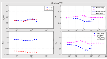
Fig. 3: Apparent resistivity and phase curves for off-diagonal impedances at site T01 and tipper function for Taapaca volcano. The AMT site shows fitting problems at longest periods. Apparent resistivity and vertical transfer function are fitted quite well, beside some small poor fits at longer periods. This may be a result of a topography effect or the cell distribution and dimension.
