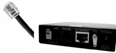
Figure 6 Example of a VDSL Ethernet Extender.
