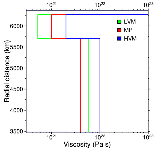
Figure 3.2: Radial viscosity distribution for the viscoelastic earth models LVM, MP and HVM.
