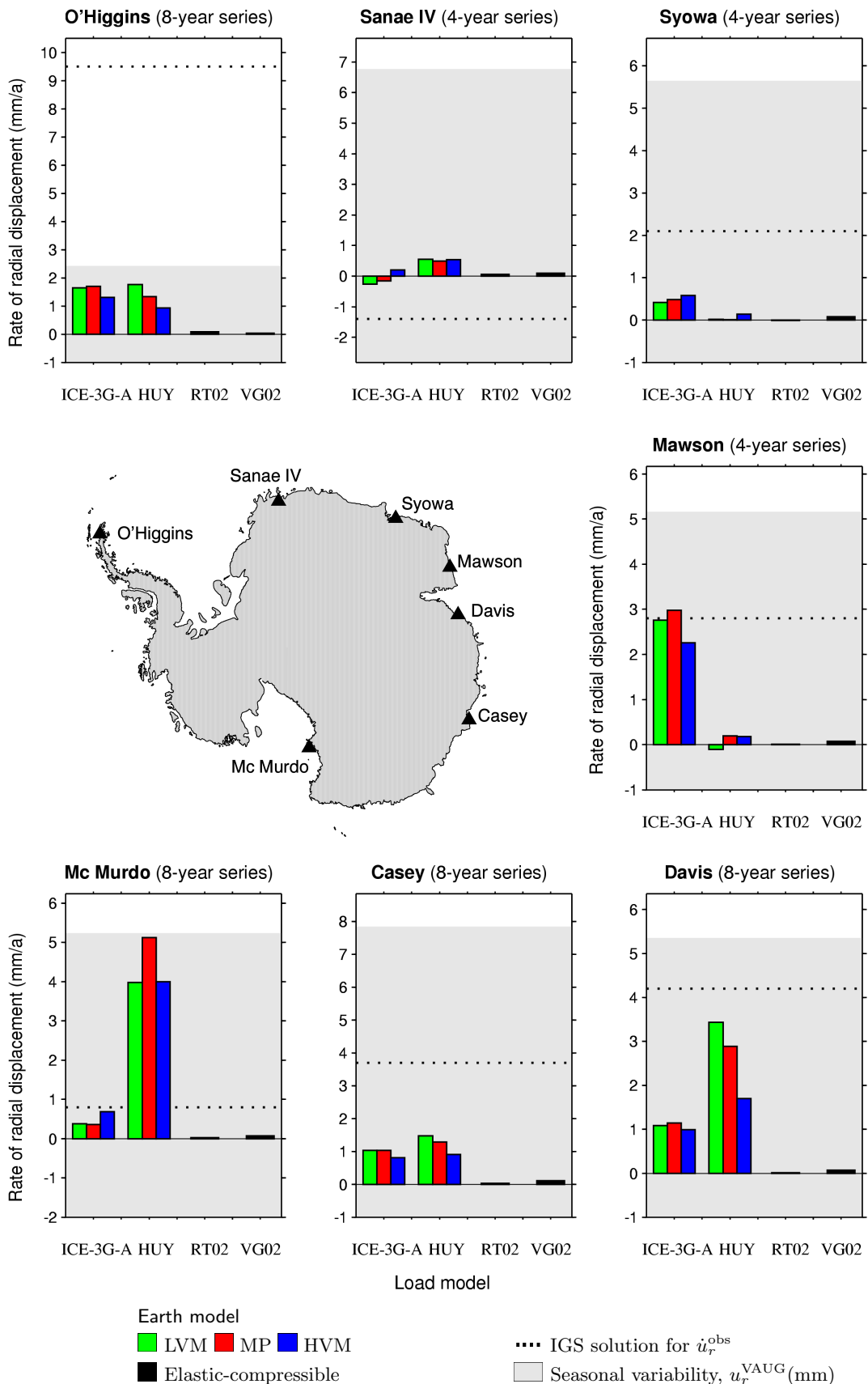
Figure 6.4: Precision and observations of \dot{u}_r for the IGS GPS stations. The GPS solutions for \dot{u}_r^{\text{obs}} are taken from the International GPS Service (2003 [online]).
