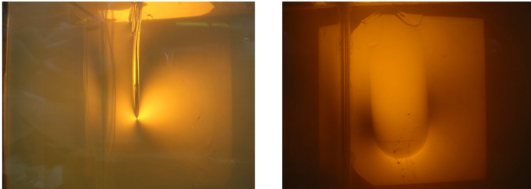
Figure 6: Stress field around a downward-propagating glycerin-filled crack in gelatin as evidenced by illuminating the tank through a polariser (left: cross-sectional view, right: frontal view).
