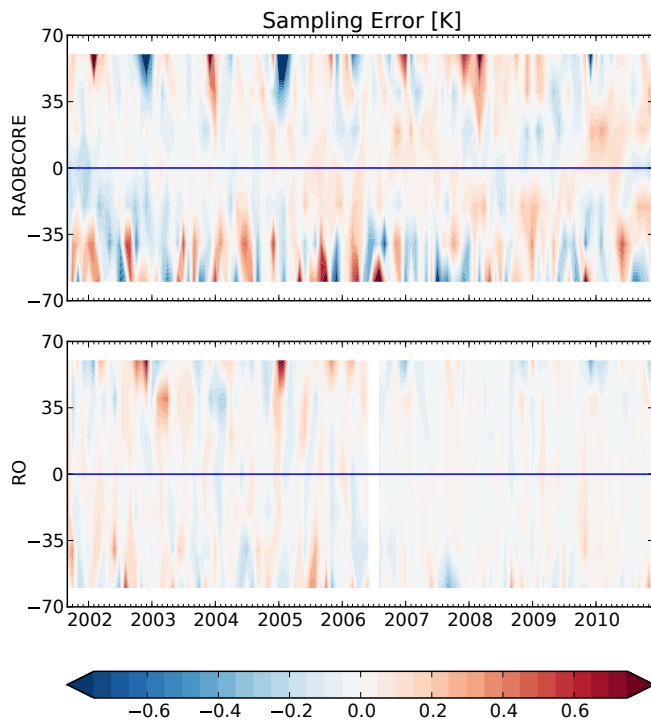
Fig. 5. Sampling error of (top) radiosondes and (bottom) RO. Shown are latitudinal bands at 20^\circ resolution.
