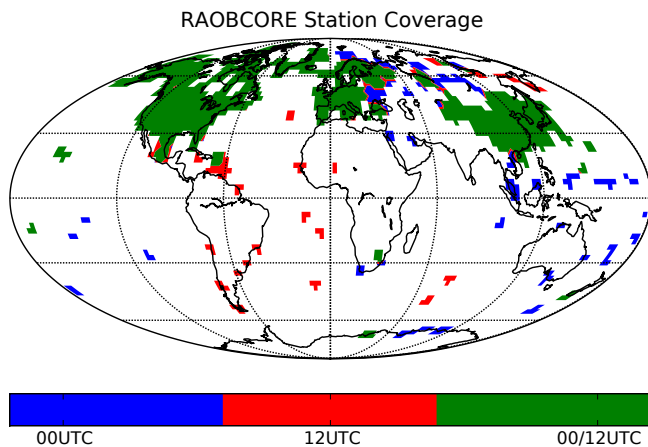
Fig. 3. Global coverage of radiosonde launches used in the RAOBCORE and RICH datasets. The color code shows whether there are launches at 00UTC (blue), 12:00 UTC (red), or at both times (green), in the corresponding 2.5^\circ \times 2.5^\circ bin.
