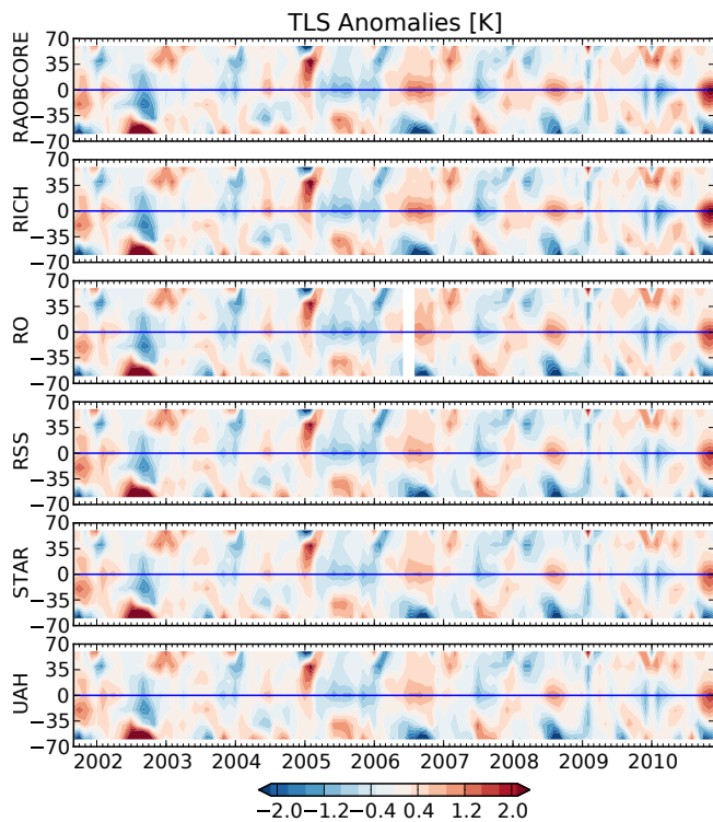
Fig. 7. Evolution of TLS anomalies for radiosondes (RAOB CORE, RICH), RO, and (A)MSU (RSS, STAR, UAH) (top to bottom), shown at 20^\circ resolution.
