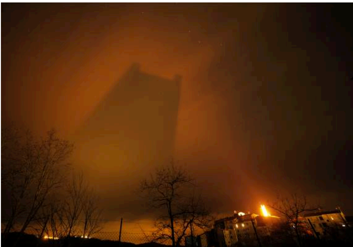
Figure 23: Shadow of the church tower illuminated by a single upward directed floodlight. Photo by Zoltan Kollath. More images are available at http://lossofthenight.blogspot.de/2015/03/effect-of-single-floodlamp-in-natural.html .
