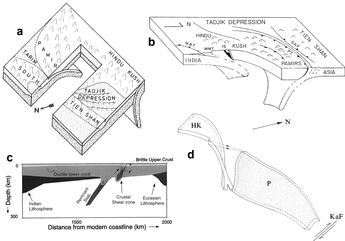
Figure 2.6.: Conceptual sketches of a selection of proposed models for the Pamir-Hindu Kush: Two-plate model, featuring intracontinental southward subduction of Eurasia in the Pamir and northward subduction of Indian material in the Hindu Kush (Figure from Burtman and Molnar, 1993 ) Model of southward subduction of Eurasia in the Pamir, steepened by the impingement of underthrusting India (Figure from Fan et al., 1994 ) A single, remnant slab of Indian provenance floating in the mantle due to neutral buoyancy, deformed as a consequence of mantle flow (Figure from Pavlis and Das, 2000 ) Single, contorted slab of Indian provenance, contortion due to relative northward translation along the Karakorum Fault (Figure from Pegler and Das, 1998 )
