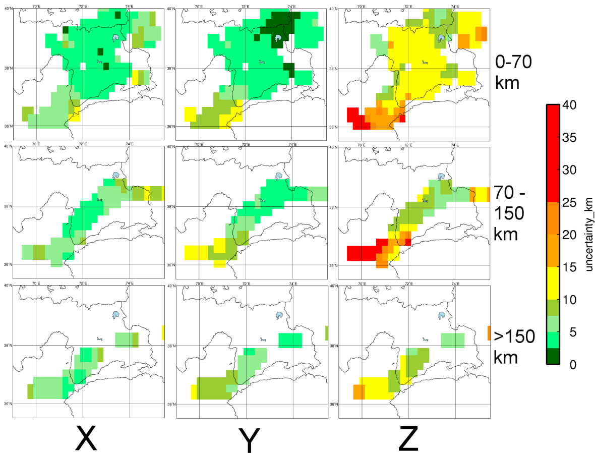
Figure 4.9.: Mean location uncertainty, i.e. extent of the error ellipsoid, in longitudinal, latitudinal and vertical direction calculated for 0.25^\circ \times 0.25^\circ bins in three depth layers, indicated at the right of the images. Bins containing less than five earthquakes are left blank.
