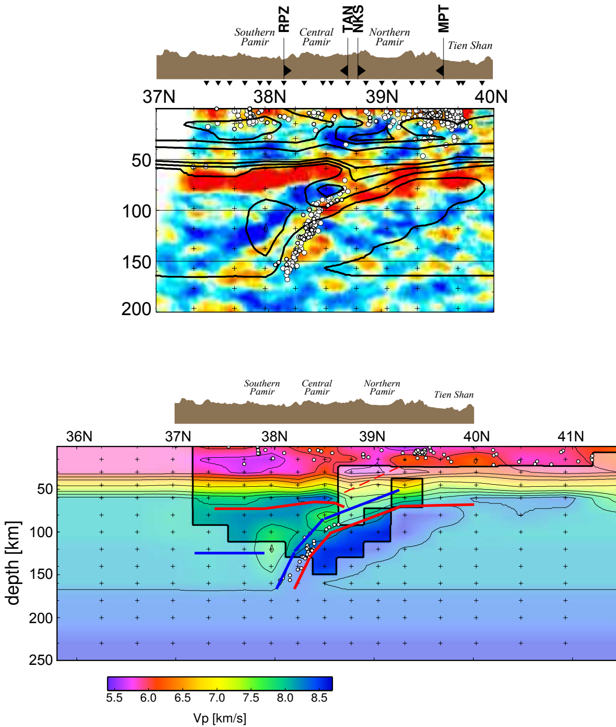
Figure 6.22.: ( upper subplot: ) Overlay of v_p contour lines from the tomographic study presented herein onto P-to-S receiver function results of Schneider et al. (2012). Their dipping converter in red clearly corresponds to the upper boundary of the Pamir slab. ( lower subplot: ) Interpreted converters (red lines indicate upward decrease of velocity, e.g. at the Moho, blue lines upward velocity increase) of Schneider et al. (2012) overlain onto tomographic cross section. The low-velocity channel discovered in this study is situated right on top of the Pamir slab and might be imaged as a much broader zone of lowered v_p
