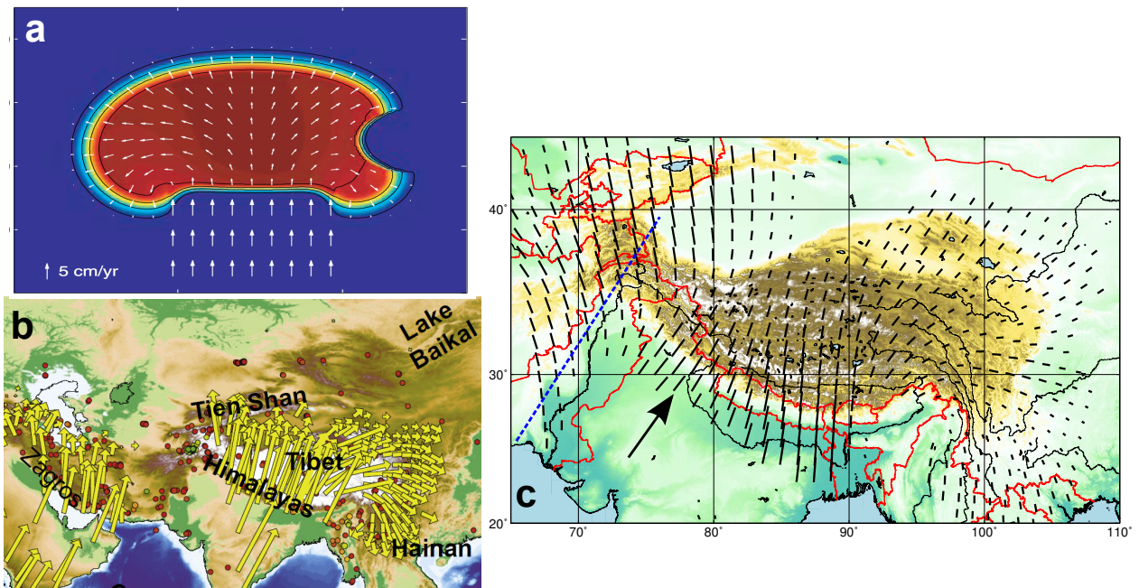
Figure 6.26.: a: Numerical simulation result of the indentation of a rigid India into plastic Eurasia (red), effecting a rotation of displacement vectors away from the indenter on the Eurasian side near the syntaxes (Figure taken from Cook and Royden, 2008 ) b: Compilation of GPS displacement vectors, showing India's NNE motion relative to Eurasia. Figure modified from Becker and Faccenna (2011) . Plotted datasets from Zhang et al. (2004) , Gan et al. (2007) and ArRajehi et al. (2010) . c: Orientation of principal compressive axes for the Himalaya-Tibet region, computed on a regular grid with the code SSPX ( Allmendinger et al., 2007; Cardozo and Allmendinger, 2009 ). Computations carried out by M. Moreno (pers. comm., 2012) , using GPS data of Zhang et al. (2004) , Mohadjer et al. (2010) and Zubovich et al. (2010) . Results show that the pure northward compression that constitutes the background deformation in the Pamir-Hindu Kush is likely an edge effect of the NNE-ward indentation of India into Eurasia. Dashed blue line traces the approximate western outline of the Indian indenter. Together with the principal direction of indentation (black arrow), this could lead to a constellation where underthrust India has its westward termination around the western edge of the Tarim Basin.
