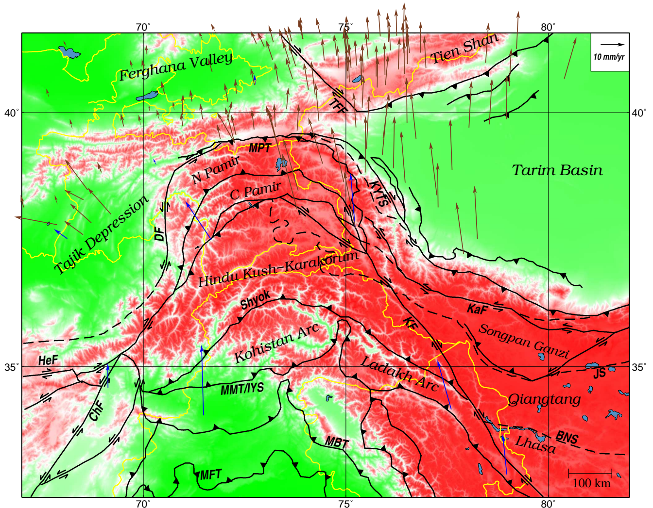
Figure 2.3.: Topographic map of the study region, showing GPS velocities relative to stable Eurasia (brown arrows from Zubovich et al. (2010), blue arrows from Mohadjer et al. (2010)) and tectonic features (faults and sutures), taken from Robinson et al. (2004) and Mechie et al. (2012). HeF = Herat Fault, ChF = Chaman Fault, MFT = Main Frontal Thrust, MBT = Main Boundary Thrust, MMT/IYS = Main Mantle Thrust/Indus-Yarlung Suture, DF = Darvaz Fault, MPT = Main Pamir Thrust, TFF = Talas-Ferghana Fault, KYTS = Kashgar-Yecheng Transfer System, KF = Karakorum Fault, KaF = Karakax Fault, BNS = Bangong-Nujiang Suture, JS = Jinsha Suture
