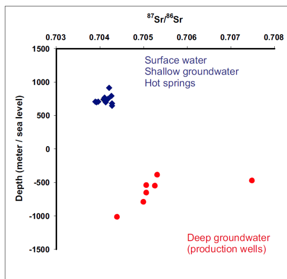
Figure 2: Sr isotope distribution in water samples collected at Lahendong.
