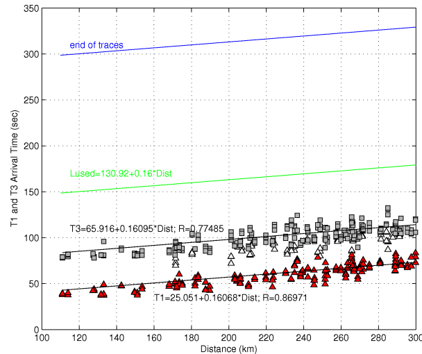
Figure 4.17: Time saved using empirical relation of T1 and T3 as functions of hypocenter distance, or using Chao et al. (2009) with the T1 and T3 at 25% and 65% of “relatively total energy” recorded at stations. Symbol remarks same as 4.13.
