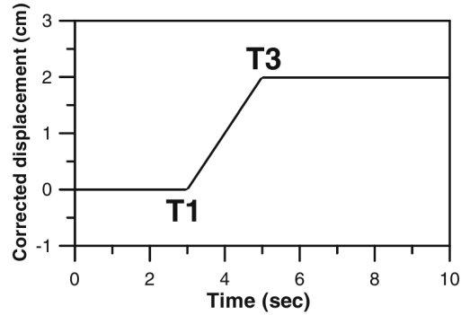
Figure 2.12: The ramp function of displacement trace proposed by Wu & Wu (2007). The flatness of displacement trace is observed to determine corrected displacement. T1 is time point when the ground displacement starts to move from zero position. T3 is time point when the ground displacement has just reached the permanent position.
