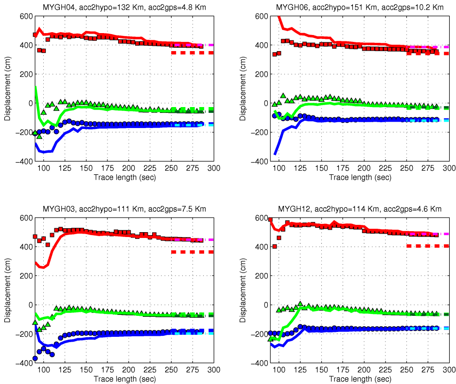
Figure 4.16: Demonstration of static displacements calculated at four stations using different length of waveforms. Red squares, blue circles and green triangles represent displacements calculated following Eqs. 4.7 and 4.8 for east-west, north-south and vertical components, respectively. Solid lines colored in red, blue and green represent displacements calculated using Chao et al. (2009) with T1 and T3 at 25% and 65% of “relatively total energy” recorded at stations. Dashed lines colored in red, blue and green represent nearby GPS data. Dashed-dot lines colored in magenta, cyan and dark green represent displacements obtained from Chao et al. (2009) method using complete 100% of energy.
