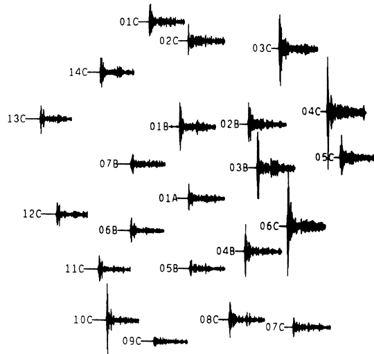
Fig. 4.36 Records of a Semipalatinsk event at stations of the NORSAR seismic array (diameter about 90 km). The event is about 37\text{-}38^\circ away. Note the remarkable variations of signal amplitudes by a factor up to 10 (the standard deviation is about a factor of 2) (from Tronrud, 1983a).
