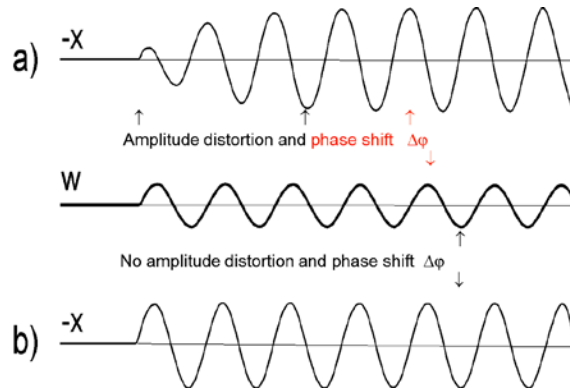
Fig. 4.19 Simulation of displacement signal output x(t) (= relative displacement of the seismometer mass) of a spring-mass pendulum seismometer responding to a monochromatic harmonic ground motion w(t) of period T = 1 s (thick line in the middle). a) Displacement output of a seismometer with low damping ( D_s = 0.2 ) and eigenperiod T_s = 1 s (i.e., resonance); b) Displacement output of a long-period and normally damped seismometer ( T_s = 20 s; D_s = 0.707 ). For discussion see text.
