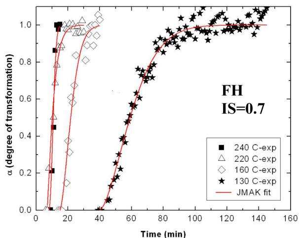
Figure 6. Degree of transformation of pure ferrihydrite to hematite as a function of temperature in the in situ EDXRD experiments.
