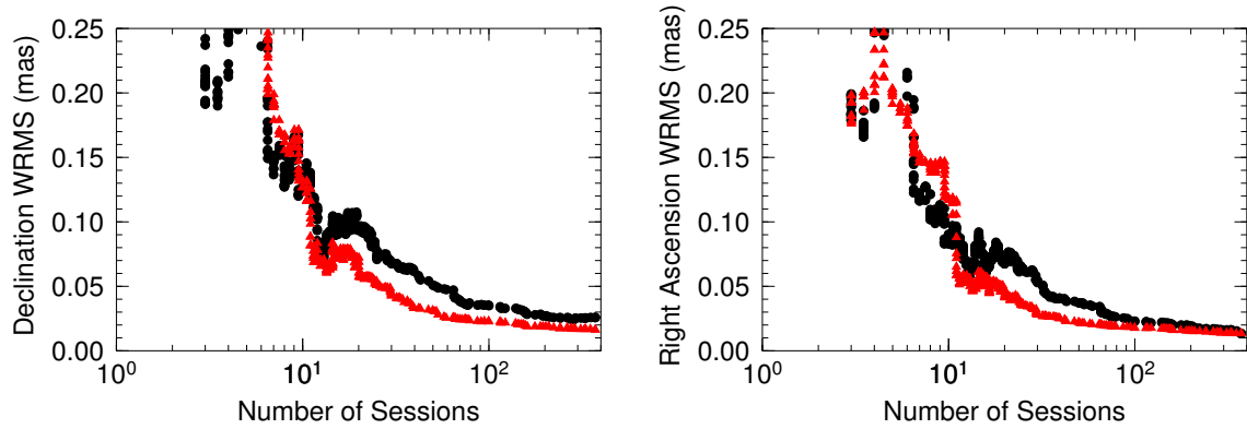
Fig. 1.— Wrms noise (solid circles) for subsets of 50 sources in each decimation solution as a function of the minimum number of sessions in which a source was observed. The median formal uncertainty (red triangles) in each subset is shown for comparison. These values were derived from differences between positions in the two decimation solutions discussed in §7.3.
