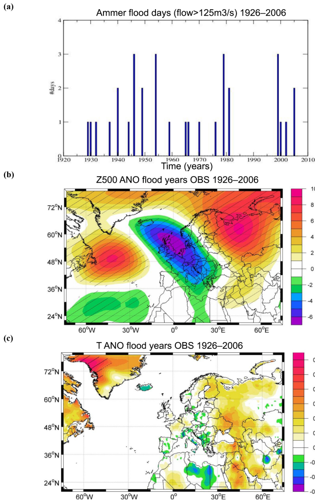
Figure 5. (a) Observed River Ammer flood frequency (daily discharge higher than 125 \text{ m}^3 \text{ s}^{-1} ) and (b) composite map of Z500 and (c) air temperature anomalies for flood years. Hatched regions: anomalies significantly different from zero (90 % level). Units: Z500 (m) and T ( ^{\circ}\text{C} ).
