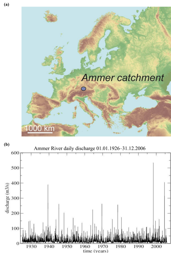
Figure 1. (a) Geographical location of the Ammer catchment and (b) time series of the observed mean daily River Ammer runoff during the period 1926–2006.
