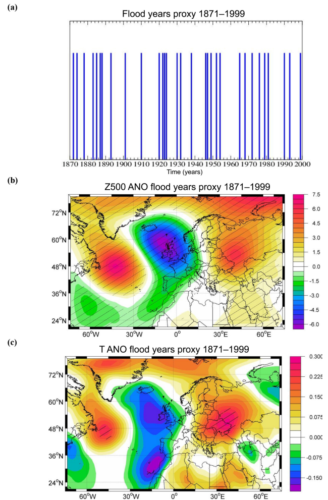
Figure 6. (a) River Ammer flood layer record for the period 1871–1999 (see text for details). Vertical bars depict years with flood layer. Composite map of (b) Z500 and (c) T anomalies for years with flood layer as shown in (a). Hatched regions: anomalies significantly different from zero (90 % level). Units: Z500 (m) and T ( ^{\circ}\text{C} ).
