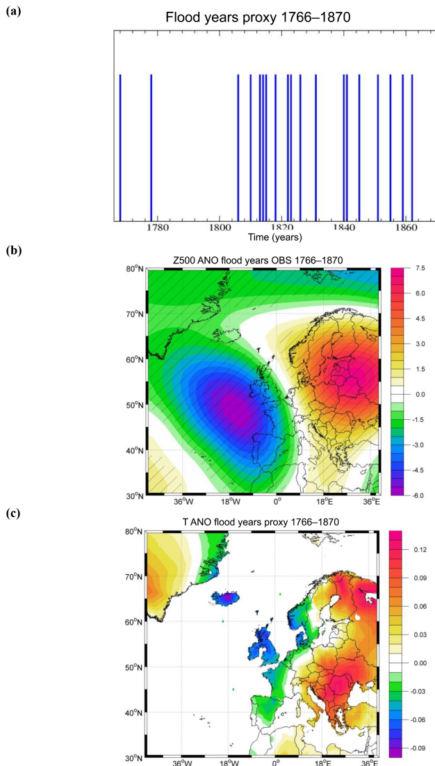
Figure 7. Same as in Fig. 6 but for the period 1766–1870.
