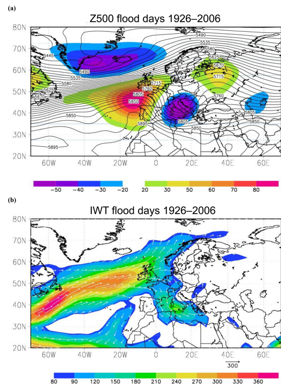
Figure 2. (a) Composite map of daily 500 hPa geopotential height (contour) and anomalies (shaded) corresponding to River Ammer floods (discharge higher than 125 \text{ m}^3 \text{ s}^{-1} ) for the period 1926–2006 and (b) composite map of IWT for flood days (vector) and its magnitude (color). Units: Z500 (m) and IWT ( \text{kg m}^{-1} \text{ s}^{-1} ).
