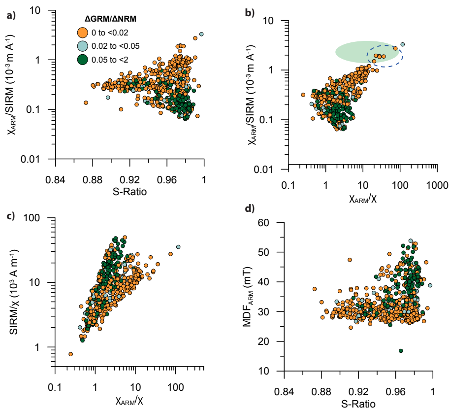
Figure 4. Selected cross plots of magnetic proxy evaluation. Samples that acquire GRM (color code) cluster in different regions of the diagrams. (a) GRM samples are characterized by high S ratios. A linear relationship between \chi_{\text{ARM}} / \text{SIRM} and S ratio relates to co-varying ferrimagnetic grain-size fining and increasing low- vs. high-coercivity magnetic mineral content. (b) GRM samples plot at \chi_{\text{ARM}} / \text{SIRM} levels typical of authigenic, inorganically precipitated greigite. A few samples from the uppermost part of the core plot in the field of bacterial magnetite (dashed circle; Snowball, 1994) and greigite (green shaded area; Reinholdsson et al., 2013). (c) GRM samples have a distinctively different gradient compared to non-GRM samples in the \text{SIRM} / \chi vs. \chi_{\text{ARM}} / \chi plot. (d) GRM samples are characterized by high S ratios and high \text{MDF}_{\text{ARM}} . Non-GRM samples show no relationship between the two parameters.
