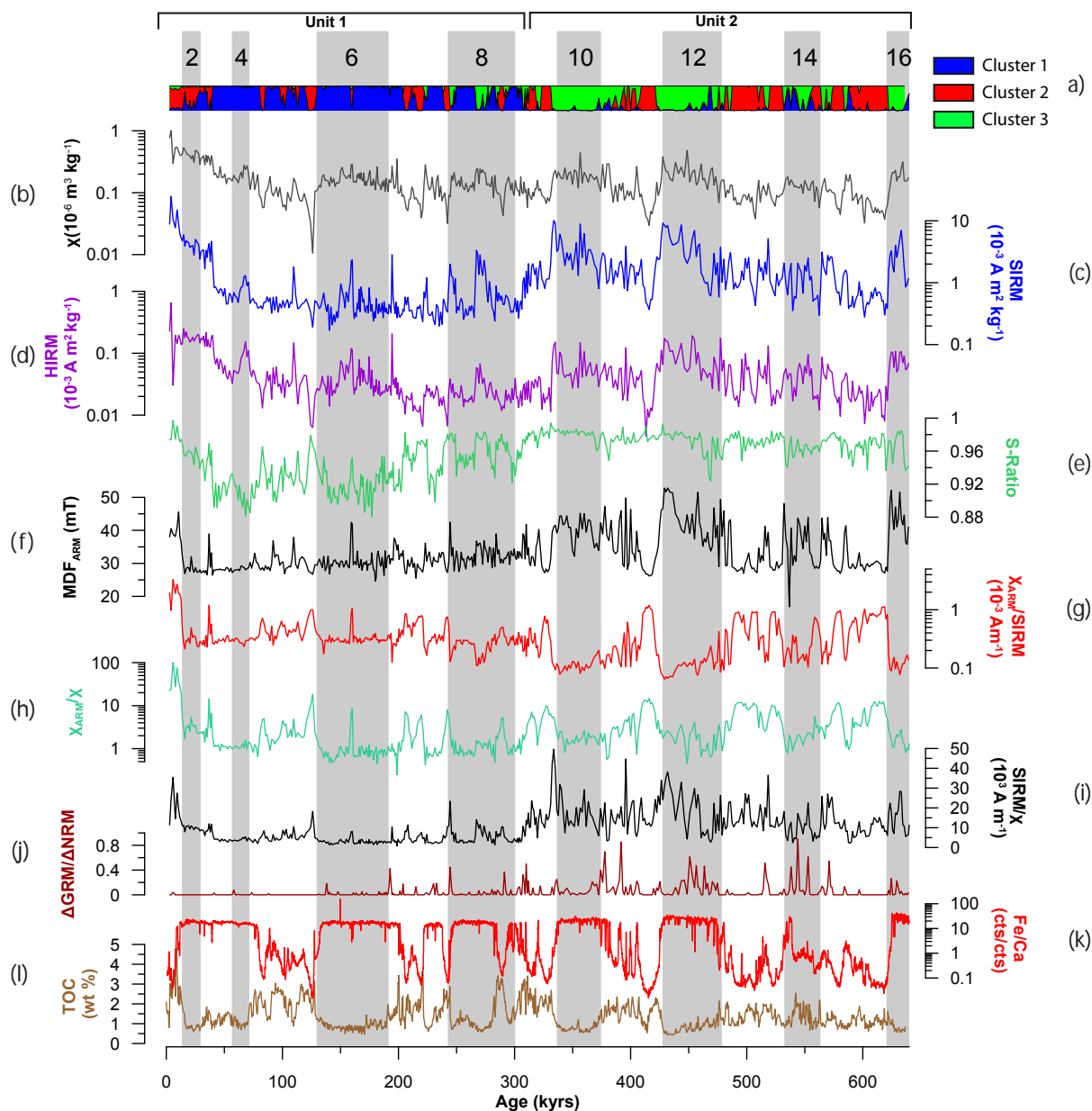
Figure 2. Compilation of magnetic and geochemical parameters measured on samples from the DEEP site. (a) Color bar indicates cluster-membership coefficients for each sample corresponding clusters in Table 2. (d–j) Rock-magnetic proxies; for abbreviations see text. (k) XRF scanning Fe/Ca counts. TOC concentrations (l) are from Francke et al. (2015). Gray bars represent marine oxygen isotope stages after Lisiecki and Raymo (2005).
