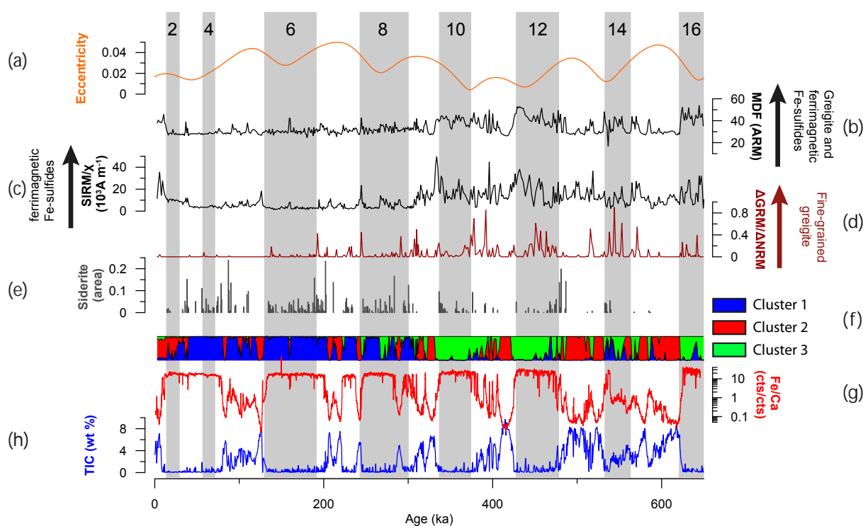
Figure 5. Compilation of parameters indicative of early diagenetic Fe-mineral formation, compared to (a) eccentricity (after Laskar et al., 2004). MDF_{(ARM)} (b), SIRM/\chi (c) and \Delta GRM/\Delta NRM (d) are elevated in the lower part, while siderite abundances (e) are higher in the upper part of the core. Cluster-membership coefficients (f) imply a glacial–interglacial pattern for iron sulfides (green). Iron sulfides and siderites occur also at elevated Fe/Ca (g) ratios during interglacials. Geochemical differences between the upper and lower unit are also visible for TIC (h) concentrations during interglacials.
