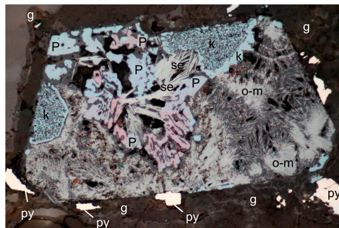
Figure 4. Petřičekite (P), end-member krot'aitite (k), native selenium (se), and olsacherite-molybdomenite (o-m) pseudomorph after clausthalite, surrounded by pyrite (py) and goethite (g). Width = 200 \mu\text{m} , without polarizers. Sample from El Dragón.
