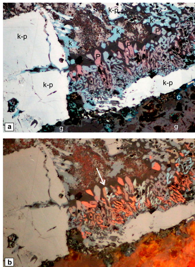
Figure 3. Fragments of krot'aitite-penroseite (k-p) cemented by skeletal palisades of subhedral petřičekite crystals (P), end-member krot'aitite (k), goethite (g), and covellite (c). The arrow marks a twinned petřičekite grain. (a) Without polarizers; (b) with partly crossed polarizers. Image width = 200 \mu\text{m} . Sample from El Dragón.
