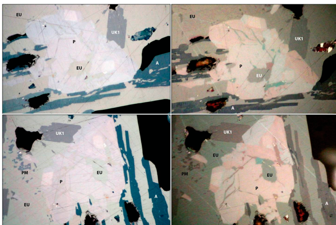
Figure 2. Reflected light images of petříčekite from Předbořice, all images have 200 \mu\text{m} width. Right hand side with partly crossed polarizers, left hand side without. Top and bottom row correspond to different extinction rotations. P = petříčekite, EU = eucairite, PM = permingeatite, A = athabascaite, UK1 corresponds to an unknown selenide currently under investigation. In plane-polarized incident light, petříčekite is pale blue grey to pale pinkish in color, weakly bireflectant and weakly pleochroic from slightly blue-grey to slightly pinkish-grey. With crossed polars, petříčekite is weakly anisotropic with light grey-blue to light pink rotation tints.
