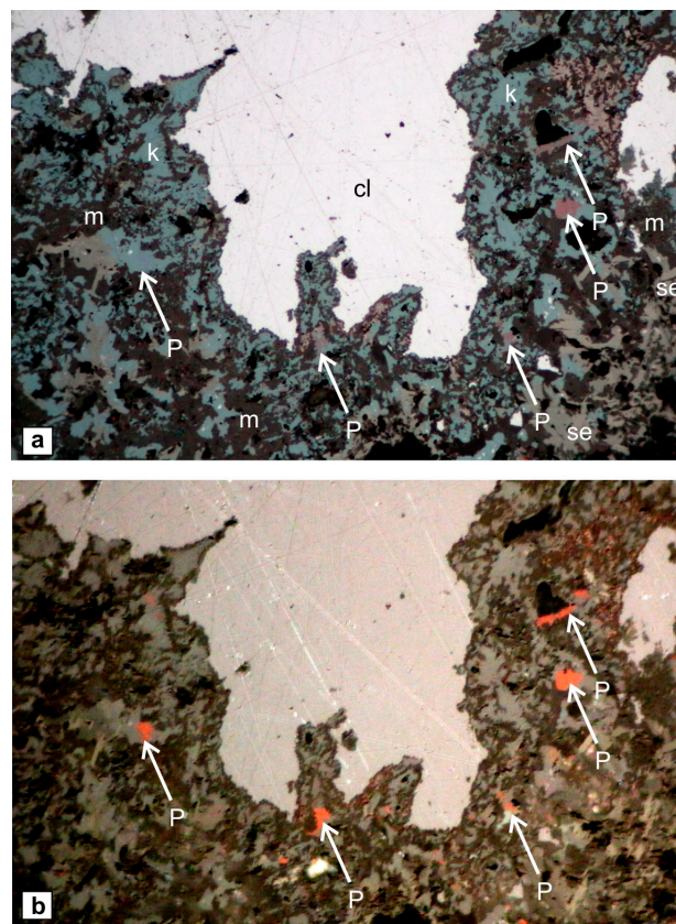
Figure 6. Sample from Sierra de Cacheuta, Argentina: Clausthalite (cl) partly replaced by krut'aite of ideal composition (blue, k), end-member petřičekite (blue-light violet, P), molybdomenite (dark grey, m) and native selenium (light grey, se). (a) Without polarizers; (b) with partly crossed polarizers. Image width = 200 \mu\text{m} .
