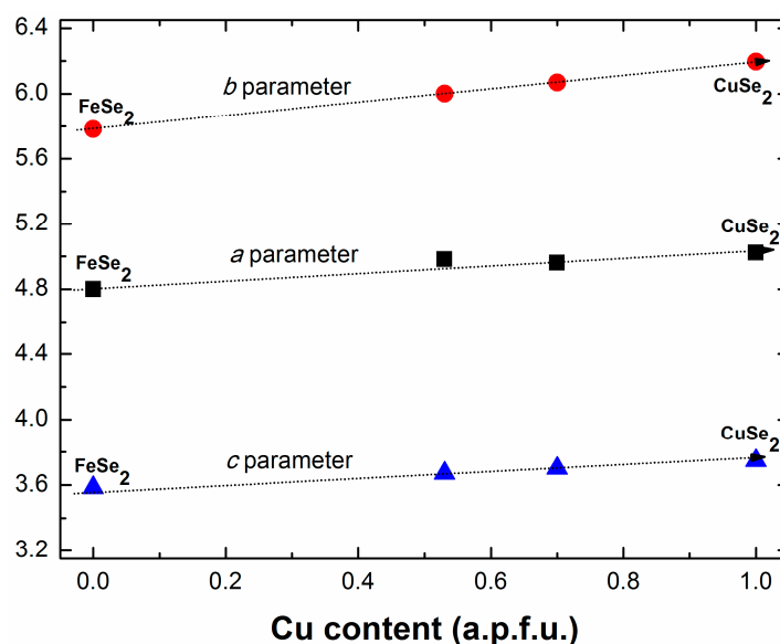
Figure 8. Unit-cell parameters (values in Å) of the two petříčekite crystals from Předbořice, plotted together with the two synthetic end-members FeSe 2 and CuSe 2 [4], as a function of the Cu content (a.p.f.u.).
