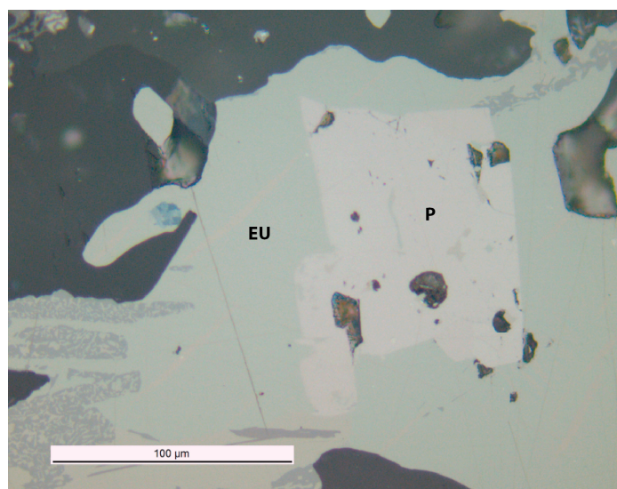
Figure 1. Reflected light photograph of the holotype grain of petříčekite (P, included in EU = eucairite) that was used for structure determination. The chemical composition of this grain is (\text{Cu}_{0.53}\text{Fe}_{0.48})_{\Sigma 1.01}(\text{Se}_{1.98}\text{S}_{0.01})_{\Sigma 1.99} .
