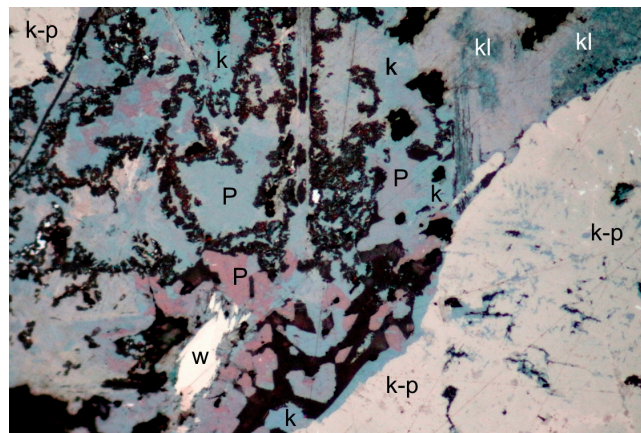
Figure 5. Petřičekite (P), krut'aite (k), watkinsonite (w), and klockmannite (kl) filling a small crack in krut'aite-penroseite (k-p). Note the fine-scale intergrowth of P and k and the partial replacement of k-p, P and w by krut'aite. Width = 200 \mu\text{m} , without polarizers. Sample from El Dragón.
