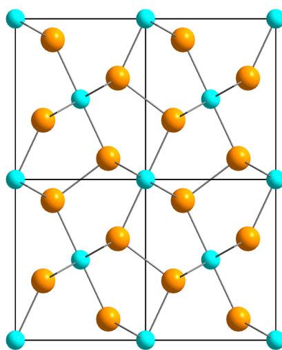
Figure 7. The crystal structure of petřičekite down the c -axis. Light-blue and golden circles indicate (Cu,Fe) and Se, respectively. Four unit-cells are depicted.
