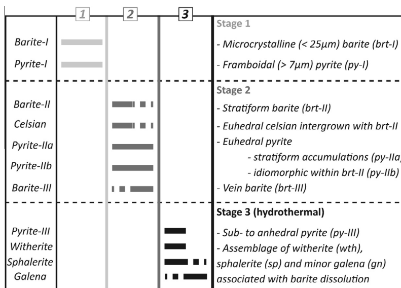
Fig. 4. Mineralogical paragenesis for mineralised samples at Tom and Jason. Stages 1 and 2 predate the hydrothermal mineralisation (Stage 3). Dashed lines reflect uncertainty in the timing relationships.
