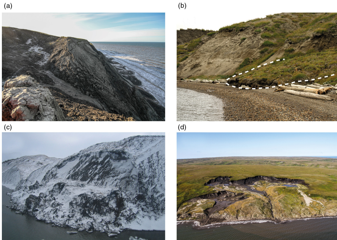
Fig. 5 Coasts of Herschel Island can undergo a series of mass wasting and accumulation processes. Material is transported as mudflows, landslides and block failures before reaching the shore. (a) Slumping, mudflows and shore accumulations on Bell Bluff; (b) active-layer detachment on the east coast (marked with a white dashed line); (c) block failure on the north coast; and (d) retrogressive thaw slump on the east coast.
