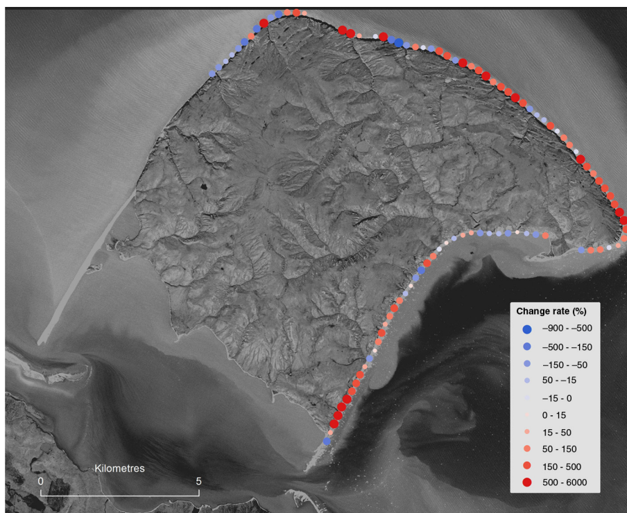
Fig. 6 Rate of change in coastline movement between 1970–2000 and 2000–2011. Coastline movement rates for 1970–2000 were estimated by Lantuit & Pollard (2008).
