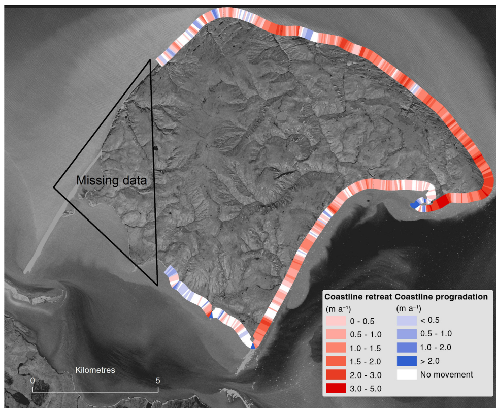
Fig. 2 Map of planimetric erosion inside belt transects on Herschel Island. Net rates of coastline movement in 2000–2011 were calculated from digitized coastlines.
