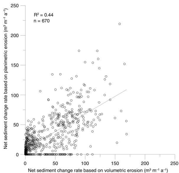
Fig. 4 Scatterplot with linear best fit showing sediment release rates based on DEM elevation change compared to sediment release calculated from coastline retreat and cliff height.
