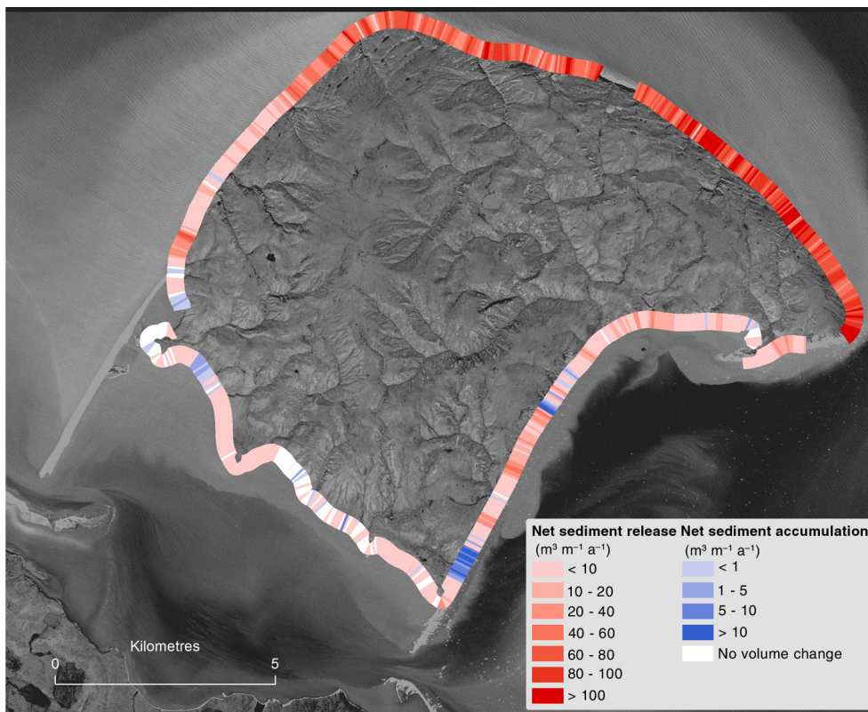
Fig. 3 Map of volumetric erosion inside belt transects on Herschel Island. Net sediment release rates in 2000–2011 are based on DEM elevation changes.
