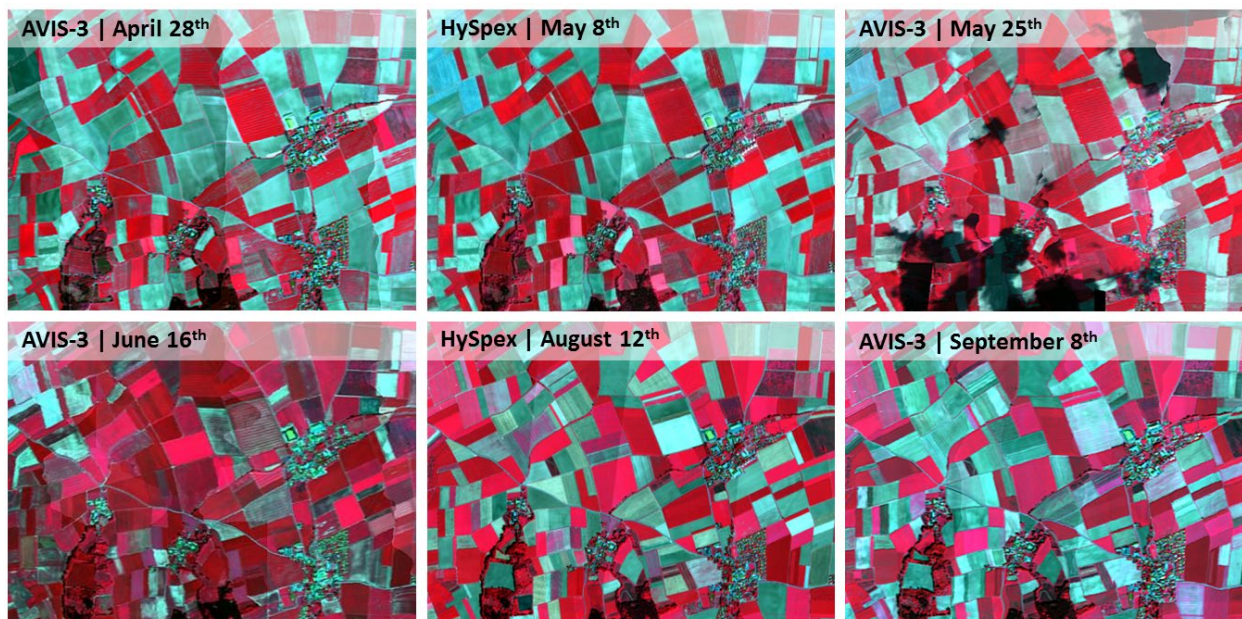
Figure 1.01: Quicklooks (false color infrared) of the multisensoral data acquired during the 2012 growing season over the 'Neusling' test area, Southern Germany.
