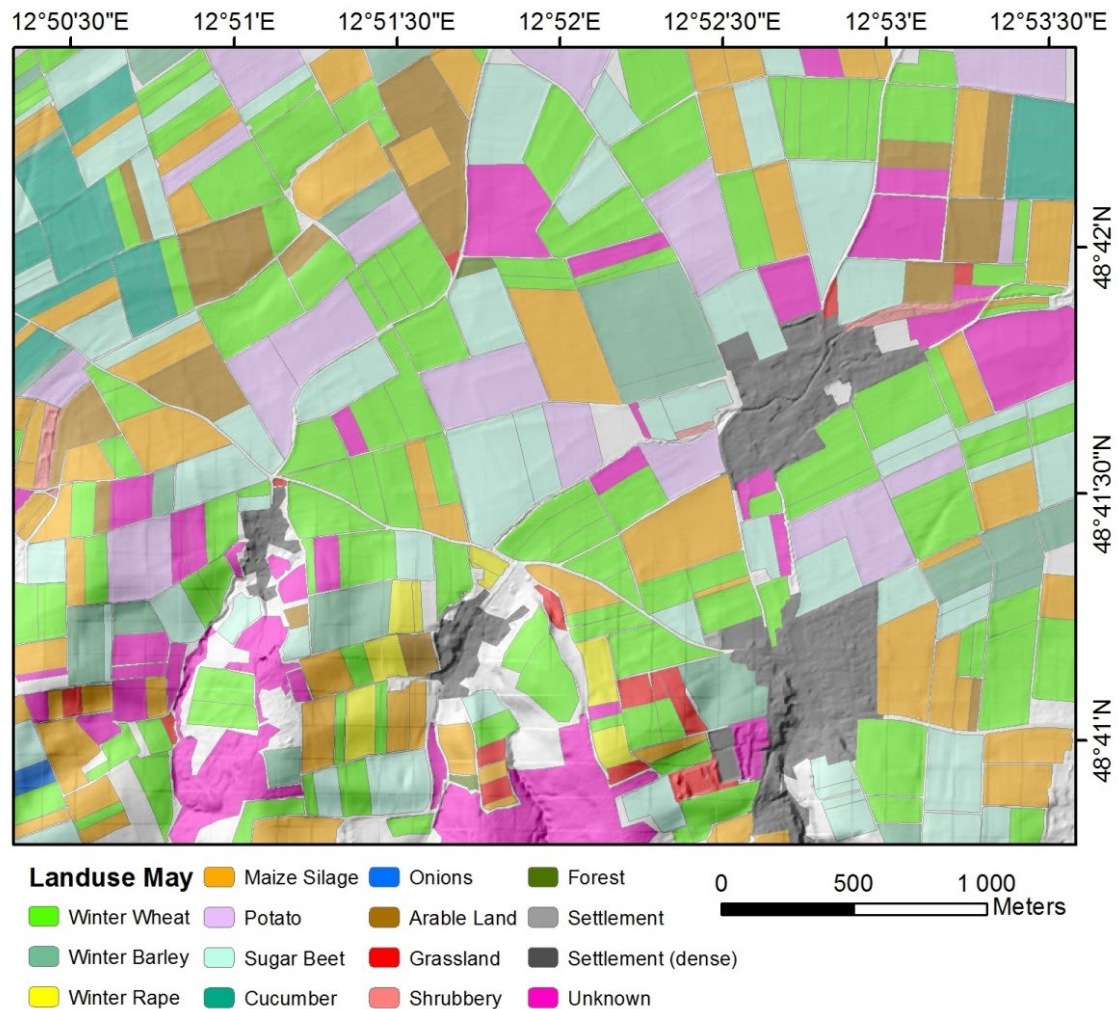
Figure 6.02: Land cover map of the Neusling test area based on in-situ observations during the month of May 2012.
