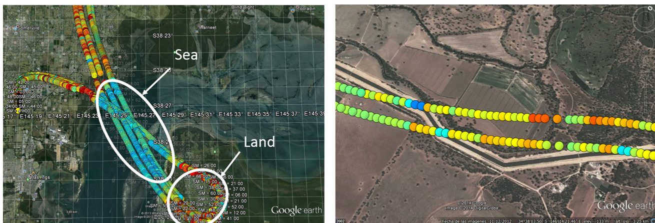
Fig. 28. Left: Sample ground-tracks of up to 4 simultaneous GNSS-R reflections after take-off Melbourne (Australia) collected with the LARGO instrument, and Right: sample ground-tracks showing the variability of the scattering coefficient over terrain and water bodies. The color scale represents the forward scattering coefficient (blue: high, red: low). The largest scattering is produced over water bodies, either the ocean (left image) or over water channels (right image). Over the ocean there is also variability due to different sea states (left). Over land (right plot), lower/higher scattering (red/blue) is associated with lower/higher soil moisture conditions (dry/moist soil). Surface roughness, vegetation, and topography effects also play a role in the magnitude of the scattering coefficient.
