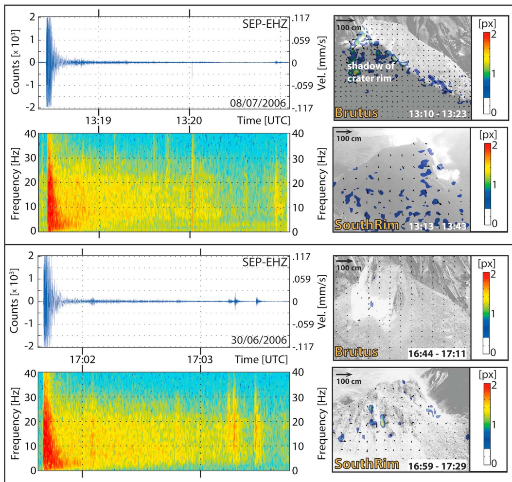
Figure 7. Trace, spectrogram, and DIC results from events lacking displacements (Events No. 25 and 14 in Table 1). Similarly to Figure 5, the signal of the leading earthquake may clip. The events lacking displacements only show weak tremor and no clear concentration of low-frequency content at the event onset when compared to the events with displacements (Figure 5).
