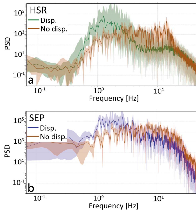
Figure 4. Power spectral densities of earthquakes associated and not associated with displacements for the seismic stations (a) HSR and (b) SEP. The solid lines show the median PSD; the shaded envelopes correspond to the minimum and maximum values. In order to reduce the contribution of the tremor following the leading earthquake, we only include the first 20 s after the onset of the event into the calculation. We used events No. 2, 8, 14, and 25 in Table 1 (no displacements) and No. 1, 3, 6, and 9 (with displacements). The corresponding waveforms are displayed in supporting information Figure S2.
