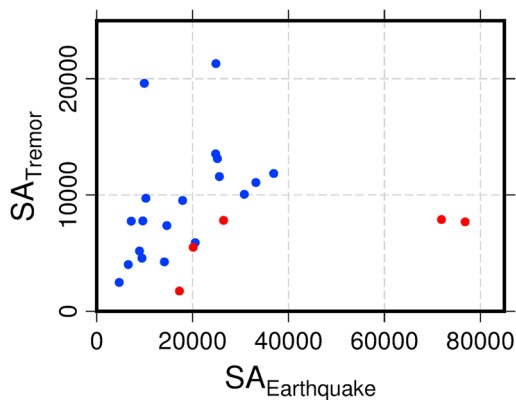
Figure 8. Average spectral values of leading earthquake spectral amplitudes ( SA_{Earthquake} ) plotted against the tremor spectral amplitudes ( SA_{Tremor} ). Values associated with deformation in the L region are plotted in red.
