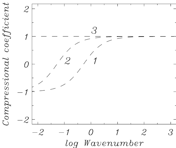
Figure 1. Compressional coefficient, \epsilon , as a function of the normalized Hankel wavenumber, n . Results apply to \kappa^* = 1 \times 10^{11} Pa (curve 1), \kappa^* = 1 \times 10^{12} Pa (curve 2) and \kappa^* \rightarrow \infty (curve 3); the other parameter values are given in Table 1.
