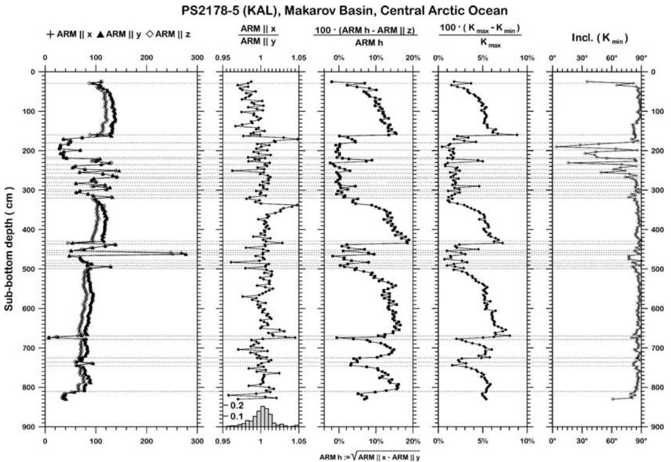
Figure 11. Results from simple experiments of anisotropy of anhysteretic remanent magnetization compared with AMS obtained from Kastenlot core PS2178-5. ARM ||x , ARM ||y , ARM ||z —ARM along the x -, y - and z -axes of the samples, respectively. For further explanation see Fig. 3.
