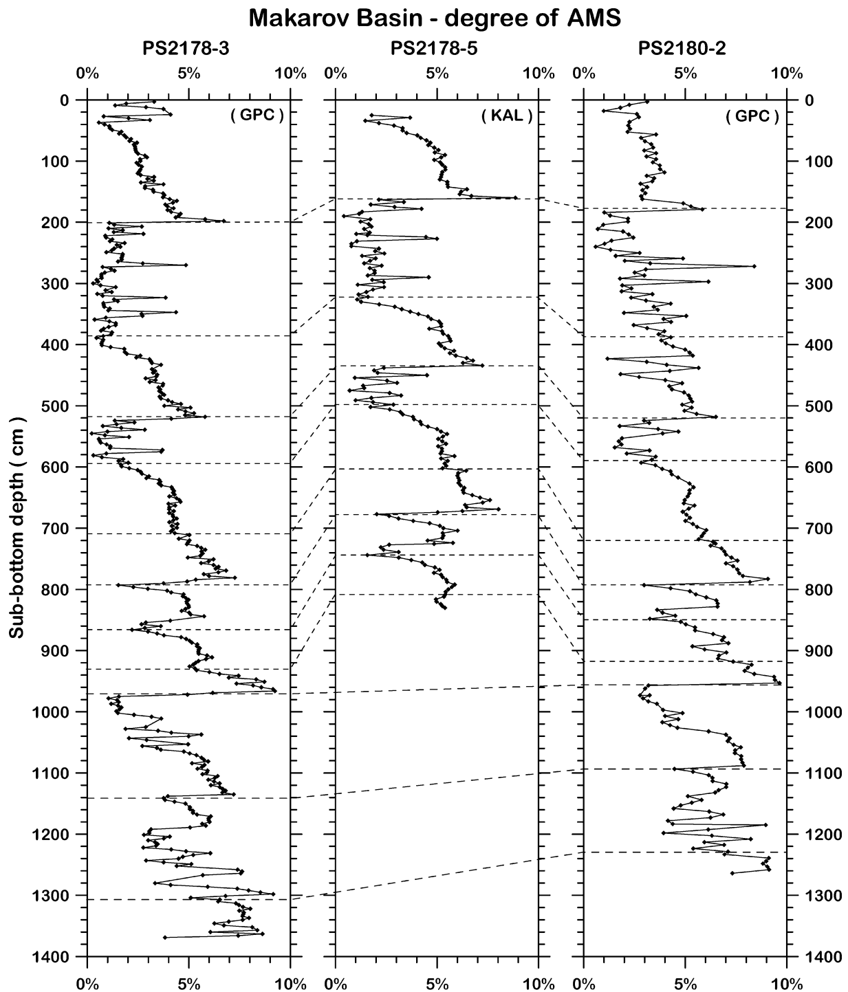
Figure 7. Degree of AMS for the three cores from the Makarov Basin. Dashed lines indicate correlation of the three cores based on the results shown in the figure and on palaeo- and rock magnetic results (Nowaczyk et al. 2001). GPC—giant piston corer, KAL—Kastenlot corer.
