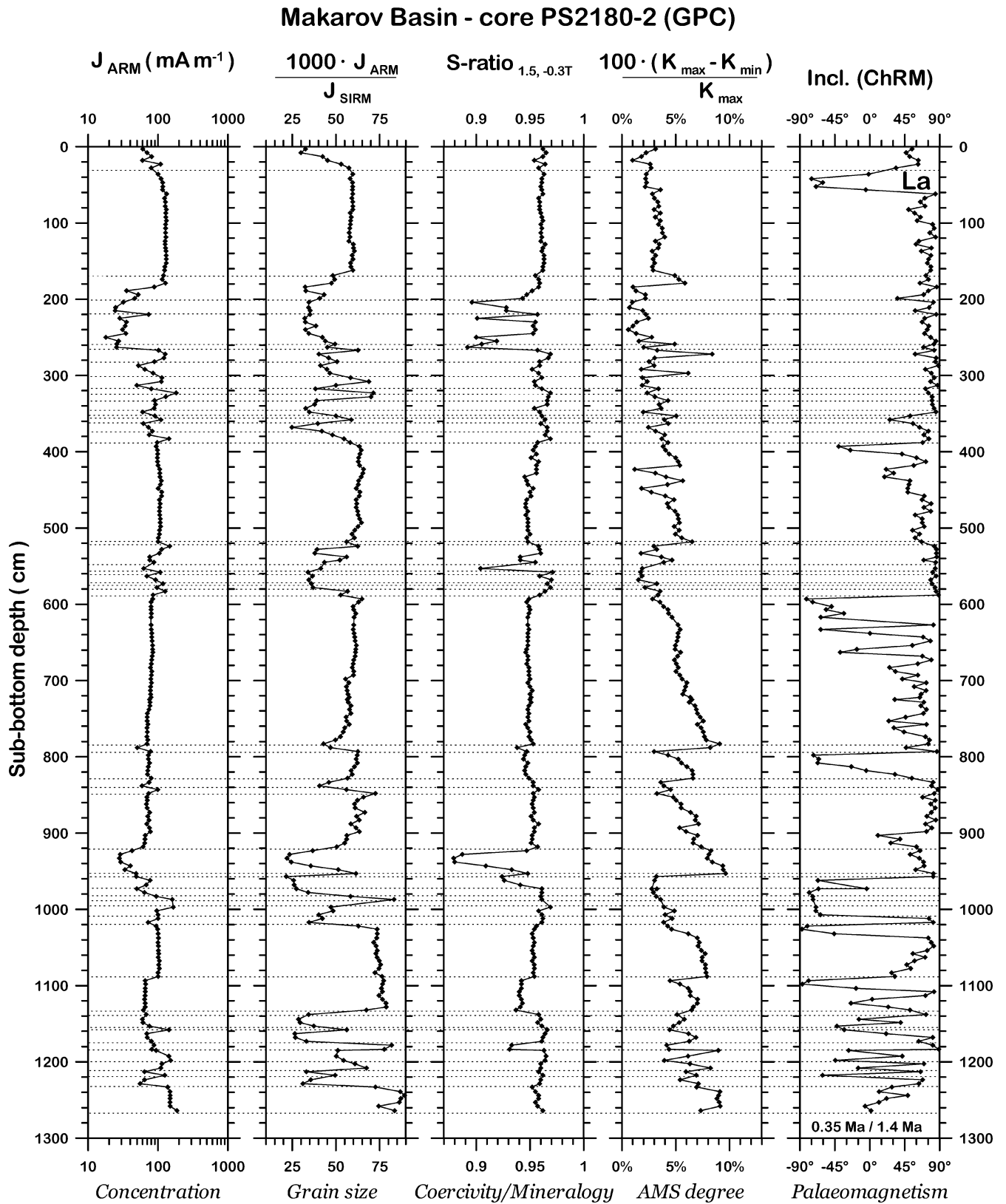
Figure 2. (b) Basic rock and palaeomagnetic data from core PS2180-2. Horizontal dashed lines indicate lithological boundaries visible within the core. Two different age models are discussed for this core (Nowaczyk et al. 2001). La—Laschamp excursion (~40 ka).
