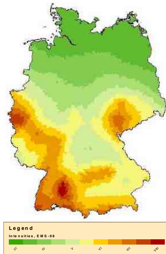
Figure 3. Seismic hazard distribution (for non-exceedance probability of 90 % in 50 years)
