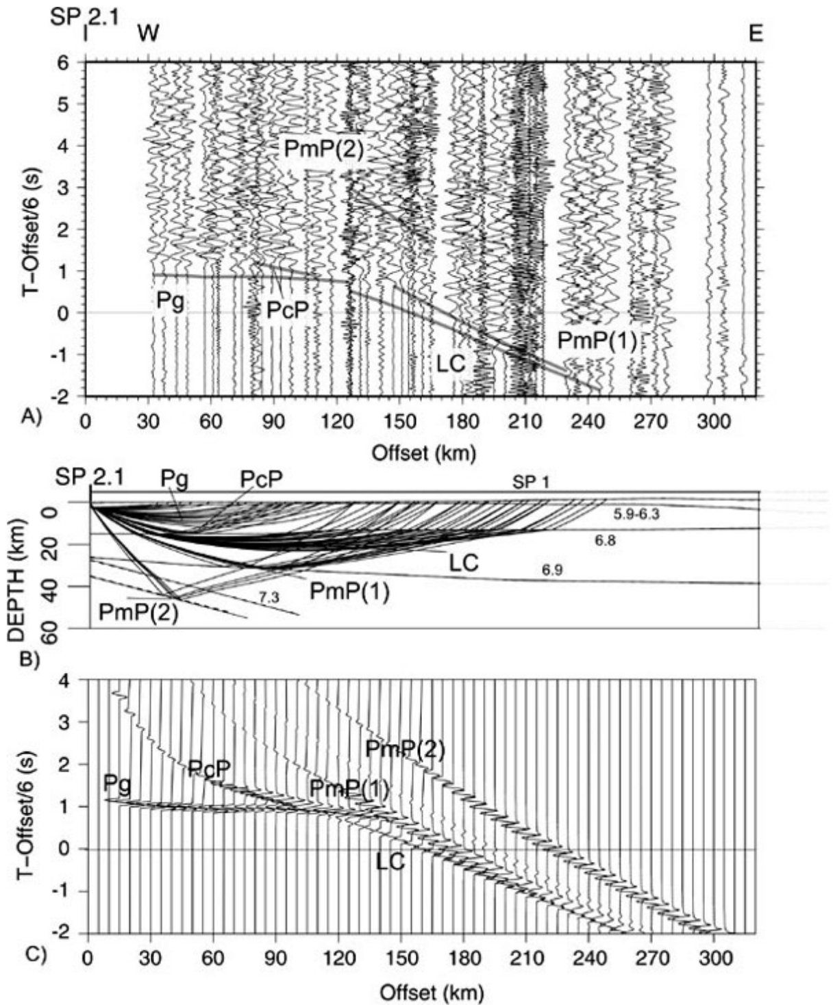
FIG. 2. A ): shot section from the shotpoint 2.1 (Pacific Ocean). The data have been bandpass-filtered 2-12 Hz and reduced with 6 km/s. Grey lines denote the modeled traveltimes of the phases which had been picked in the section; B ): ray-diagram of the correlated phases. Numbers in the ray-diagram indicate P-wave velocities in km/s; C ): ray-theoretical seismogram based on the final velocity model.
