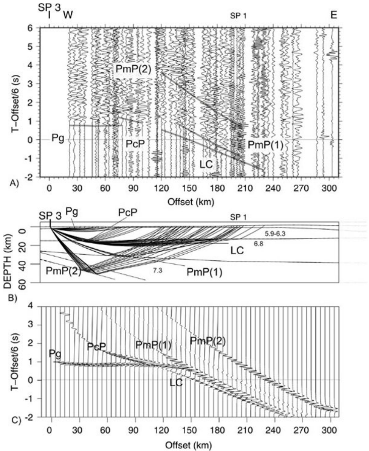
FIG. 3. A)- Shot section from the shotpoint 3 (Pacific Ocean). The data has been bandpass-filtered 2-12 Hz and reduced with 6 km/s. Grey lines denote the modeled traveltimes of the phases which had been picked in the section; B)- ray-diagram of the correlated phases. Numbers in the ray-diagram indicate P-wave velocities in km/s; C)- ray-theoretical seismogram based on the final velocity model.
