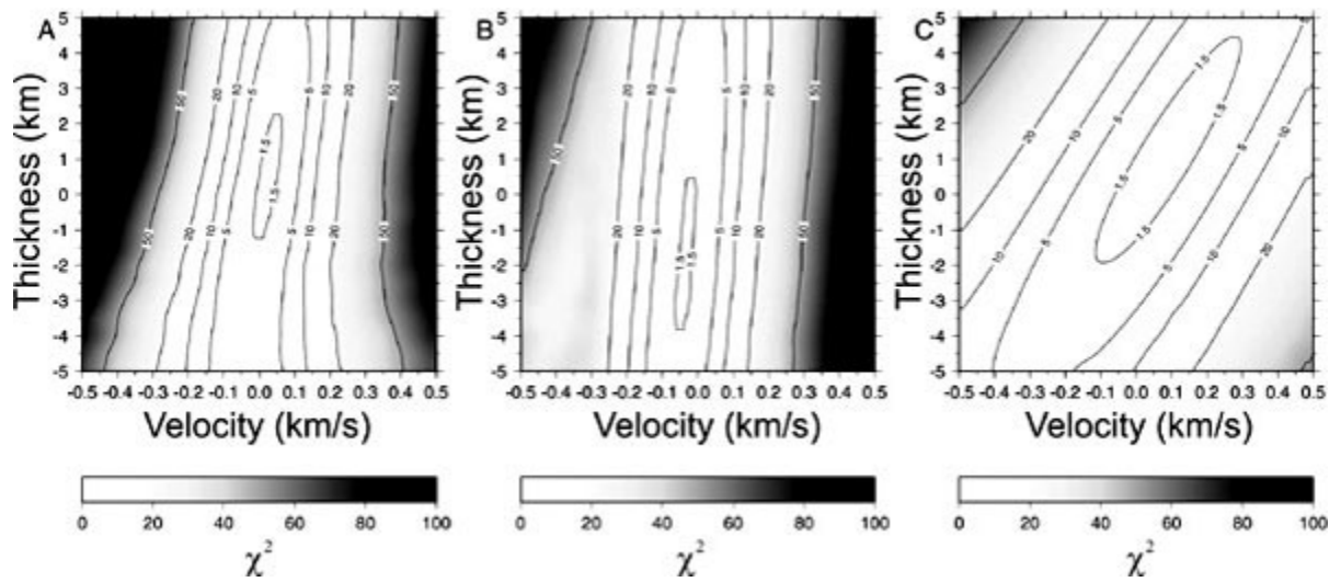
FIG. 5. 1-D perturbation analysis of upper continental crust A ; lower continental crust B , and below the lower continental crust C . The contour plots show the normalized mean-squared travelttime error in dependence on velocity and thickness perturbation of the respective layers. Due to the presence of refracted and reflected phases for upper and lower crust the trade-off is very small ( A and B ); contrary to the part of the model between lower continental crust and oceanic Moho, which is passed by reflected phases only ( C ).
