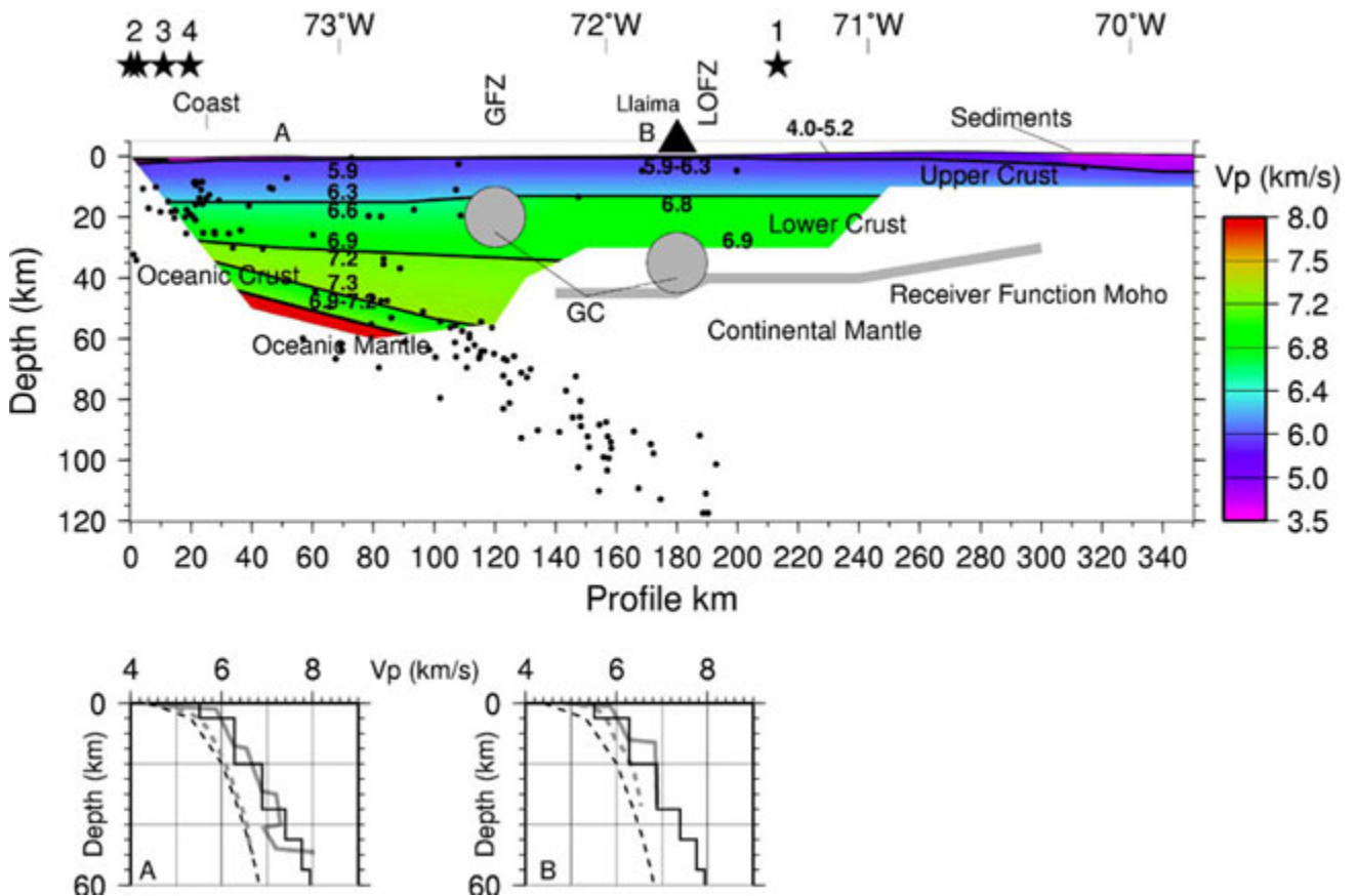
FIG. 2. P-wave velocity model as derived from iterative traveltimes modeling. The velocity model is represented by color coding and values given near the layer boundaries (thick black lines). Black dots indicate the earthquake hypocenters located from the ISSA passive seismological experiment (Bohm et al. , 2002). The hypocenters have been projected perpendicularly onto the model plane. Only events south of 37°S are shown. The position of the receiver function Moho is according to X. Yuan (oral communication, 2001). Grey circular patches at 120 km and 180 km indicate locations of good electrical conductors (GC) after Brasse and Soyer (2001). The diagrams below the section show velocity-depth functions for representative locations along the profile in the fore-arc (A) and the magmatic arc (B). Thick grey line: interval velocity of the model from seismic refraction; thin black line: 1-D velocity model from passive seismology; grey dashed line: average velocity of the model from seismic refraction; black dashed line: average velocities of the 1-D velocity model from passive seismology. GFZ - Gastre Fault Zone; LOFZ - Liquiñe-Ofqui Fault Zone.
