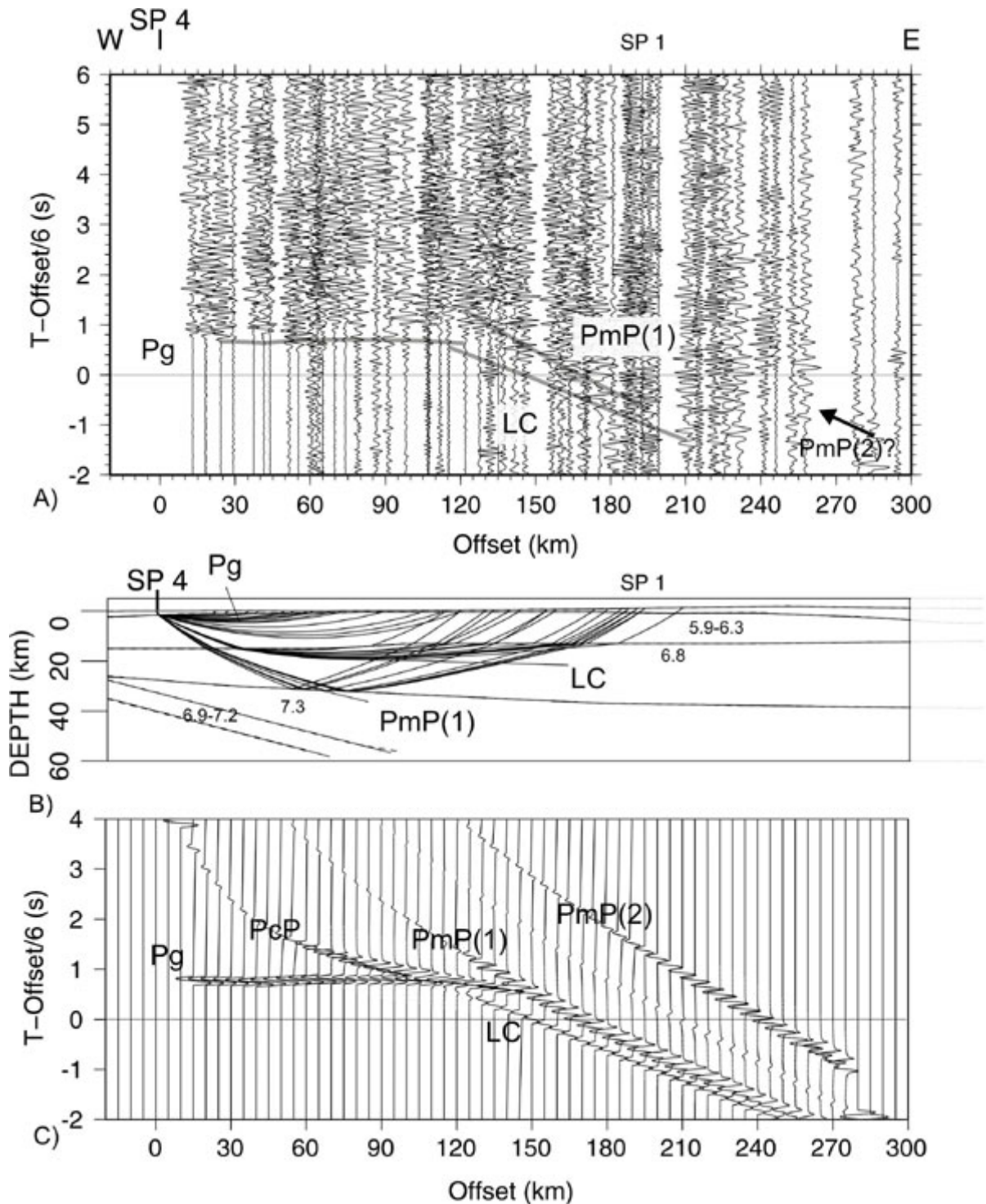
FIG. 4. A)- Shot section from the shotpoint 4 (Pacific Ocean). The data have been bandpass-filtered 2-12 Hz and
