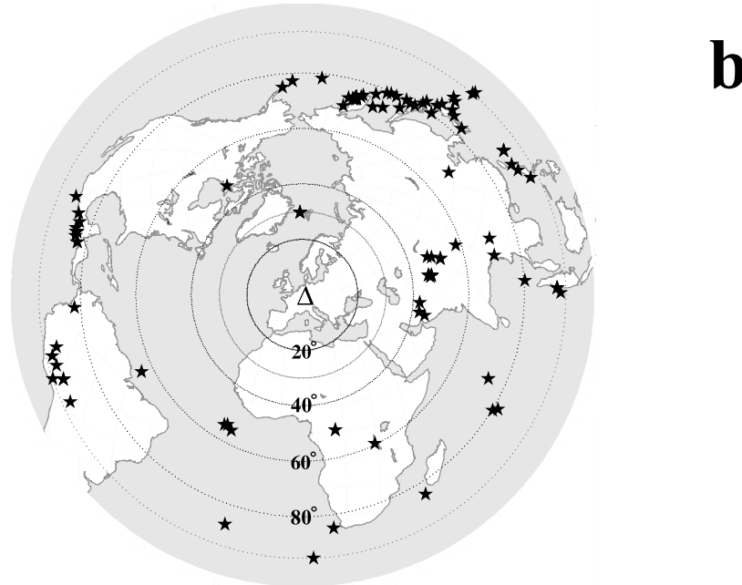
Figure 1. (a) Distribution of the 242 stations of the Eifel network (1997 November to 1998 June), including the permanent stations. The centre of the network is at the West Eifel. (b) Epicentral-equidistant map centred on the Eifel with the 96 teleseismic events used ( m_b > 5.2 , 30–95 degree).
