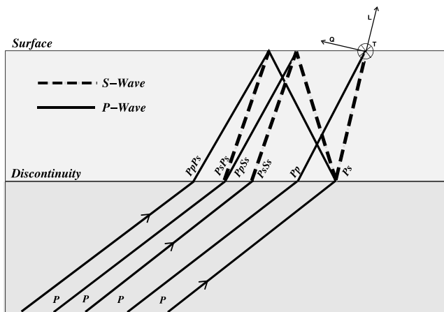
Figure 2. Sketch showing the ray path geometry used. The direct P wave, the converted Ps wave and multiples, for example, crustal multiples if the discontinuity is the Moho, are observed at the seismometer. Rotation to ray coordinates L , Q , T divides the energy into P , SV and SH energy, respectively.
