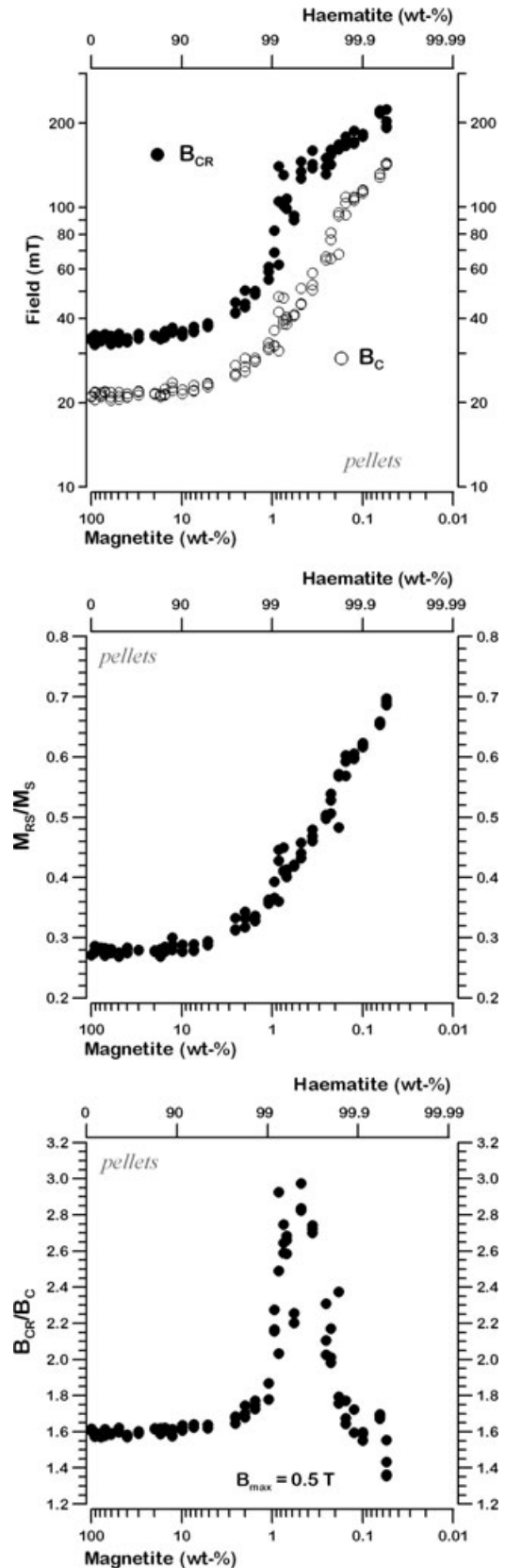
Figure 5. Relationship between the coercivity of remanence ( B_{CR} ) and coercive force ( B_C ), the hysteresis ratios saturation remanent magnetization ( M_{RS} ) over saturation magnetization ( M_S ) and B_{CR}/B_C , and the haematite/magnetite content. Determinations were carried out on small (5–60 mg) pellets.
