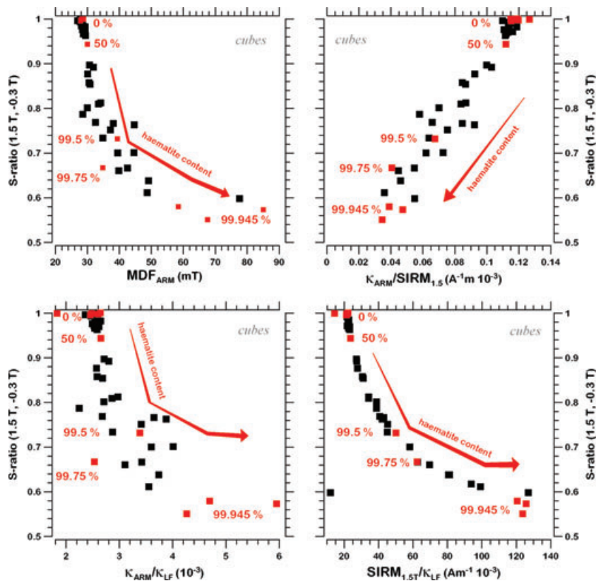
Figure 11. Bi-plots of different rock magnetic parameters and interparametre ratios illustrating the influence of variable haematite content. Numbers denote the haematite content of the samples in wt-% (red text).
