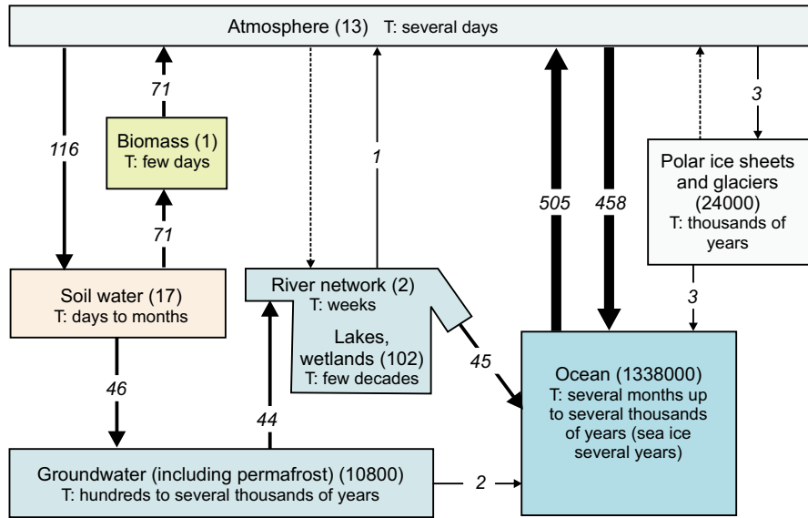
Figure 2. Storages in the global hydrological cycle. Storage volumes ( 1000 \text{ km}^3 , in brackets), fluxes ( 1000 \text{ km}^3/\text{year} , in italics ) and order of magnitude of mean water residence times (T) (after WBGU, 1997)
