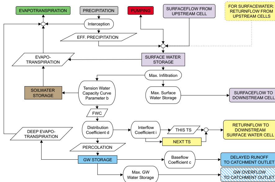
Figure 5. Flow chart of the SHM water balance model (Riegger et al., 2001)
