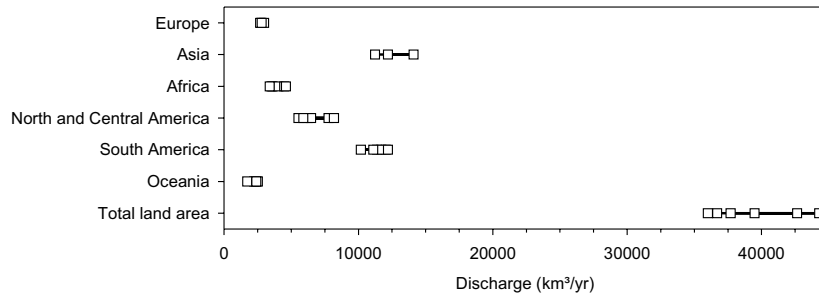
Figure 3. Long-term average annual continental discharge into oceans (estimations of six observation-based and model-based studies compared in Döll et al. 2003)
