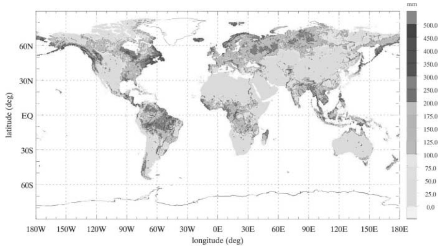
Figure 4. Average seasonal changes (changes between the months of maximum and minimum storage) of the total continental water storage (composed of the storage components snow, soil water, groundwater, river, lakes and wetlands), simulated on a 0.5 global grid with the model WGHM (Döll et al., 2003), period 1961-1995.
