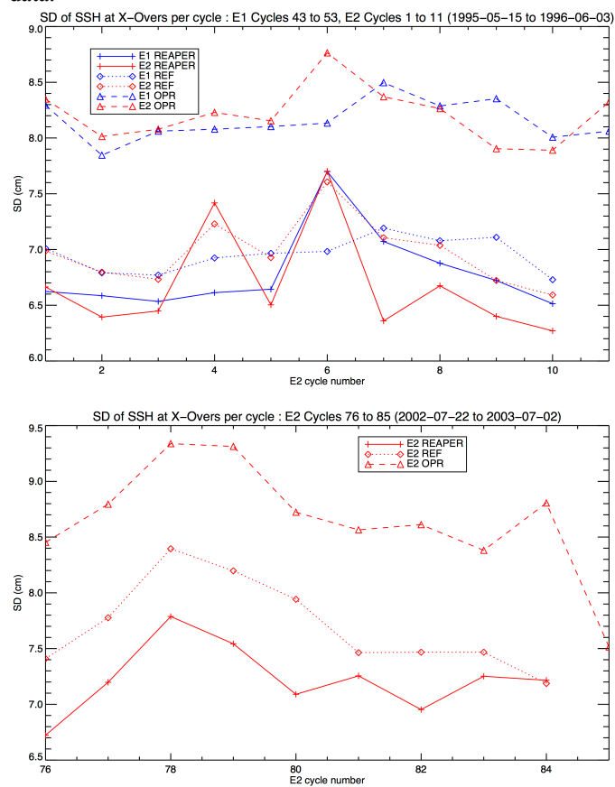
Fig. 3. Temporal evolution of the standard deviation of SSH differences at crossovers for latitudes below 50^\circ , bathymetry greater than 1000 m and low oceanic variability areas. The statistic is derived for historical OPR, updated OPR (REF), and REAPER data, and is tabulated in Table I and Table II.
