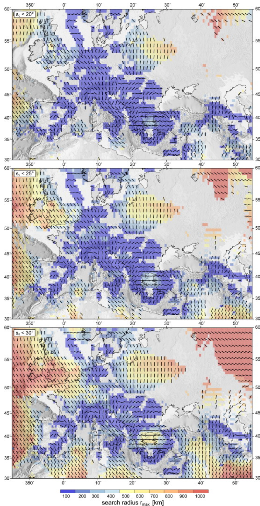
Fig. 5. Smoothed stress map of Europe for three different values of s_0 ; same legend as in Fig. 3A. In most areas of central Europe and the Mediterranean short wavelength of the stress pattern is prevailing, indicating that regional to local stress sources contribute significantly to the S_H orientation. Only in Great Britain, Ireland, offshore west and east of the Tornquist-Teisseyre Zone, that marks the border to the East European craton, the stress pattern displays longer wave-length. In contrast to California (Fig. 4) an increase of s_0 results in a gradual and smooth change of the wave-lengths of the stress pattern. Again, the S_H orientation is almost unaffected by the change of s_0 .
