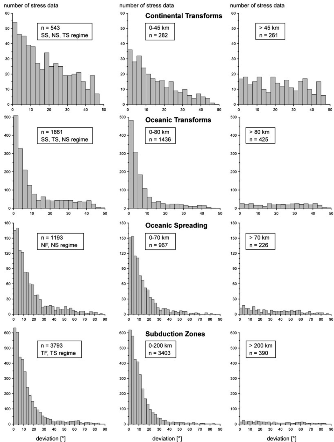
Fig. 2. Histogram of the lesser of the two deviations between the nodal plane azimuths of single focal mechanism solutions and the plate boundary azimuth. First column gives the deviation distribution of all stress data records deduced single focal mechanism solutions with the appropriate tectonic regime (SS = strike-slip, TS = transpression, NS = transtension, TF = thrust faulting, NF = normal faulting). Second column shows the deviation distribution for the datasets within the critical distance d_{crit} that resulted from the statistical analysis of the deviation distribution and the third column the deviation distribution for datasets beyond the critical distance. Rows show the deviation distribution for the different plate boundary types.
