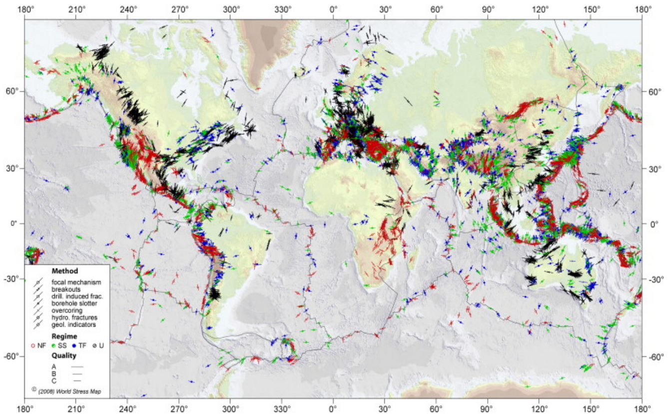
Figure 1. Global stress map based on the WSM database release 2008 using the 11,346 stress data records with of A–C quality, but excluding all Possible plate Boundary Events (PBE) (Heidbach et al., 2008, 2009). Lines represent orientations of maximum horizontal compressional stress S_H , line length is proportional to quality. Colours indicate stress regimes with red for normal faulting (NF), green for strike-slip faulting (SS), blue for thrust faulting (TF), and black for unknown regime (U). Plate boundaries are taken from the global model PB2002 of Bird (2003). Topography is based on the ETOPO1 data from the National Geophysical Data Center (NGDC) including bathymetry data from Smith and Sandwell (1997).
