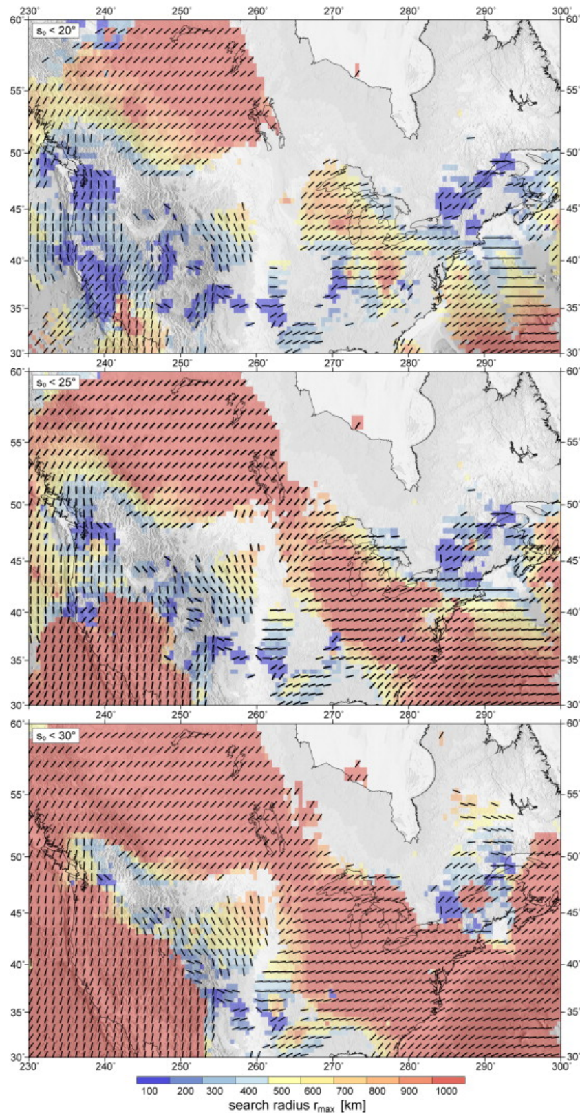
Fig. 4. Smoothed stress map of North America for three different values of s_0 ; same legend as in Fig. 3A. For all three results the overall pattern of the wave-length remains. The Basin and Range area and the NW coast exhibits short wave-length of their stress pattern. In California the high variability of data density leads to a flip of the colours from blue to red when s_0 is increased. Note that the change of the \hat{S}_H orientation with changing s_0 is insignificant.
