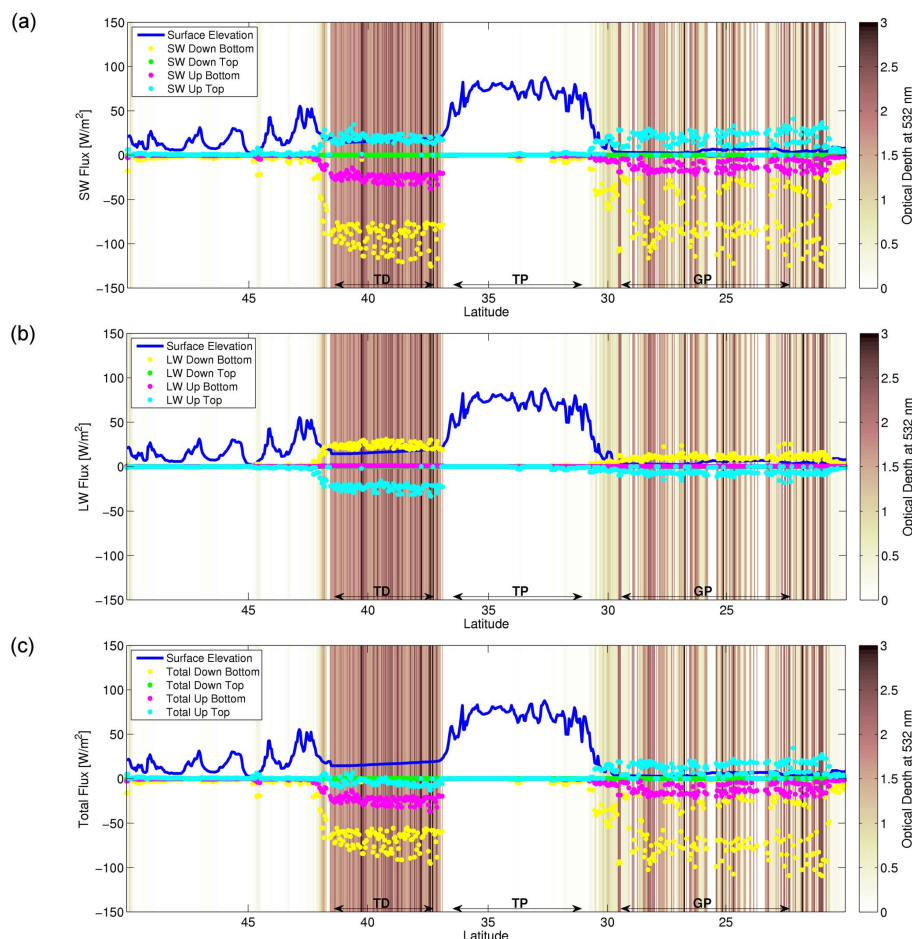
Fig. 5. Anomalies in (a) SW, (b) LW, and (c) Total (SW+LW) fluxes induced by aerosols at the top (50 km a.m.s.l.) and bottom (0 km a.m.s.l.) of the modeled atmosphere in both upward and downward directions. The background shading indicates the AOD at 532 nm as measured by CALIPSO. MODIS surface albedo values and CALIPSO aerosol distributions are used as input. Approximate extensions of the TD, TP, and GP regions are marked on the x-axis.
