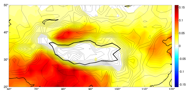
Fig. 10. Vertically averaged total heating rate anomalies due to aerosols between 0 and 8 km a.m.s.l. in K/day. Simulation with MODIS surface albedo. The thick lines indicate coasts and the Tibetan Plateau.
