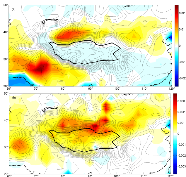
Fig. 12. Effect of albedo variations on aerosol forcing ( \Delta_{\text{alb}} ) in vertically averaged total heating rates between (a) 0 and 5 km and (b) 5 and 8 km a.s.l. in K/day. Note the different scalings of the colorbars, each time adjusted to the respective extreme value. The thick lines indicate coasts and the Tibetan Plateau.
