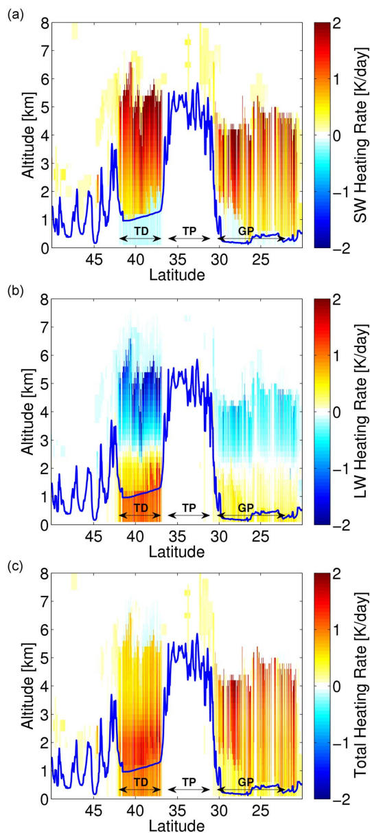
Fig. 6. Anomalies in (a) SW, (b) LW, and (c) Total (SW+LW) heating rates induced by aerosols throughout the vertical extent of the atmosphere in K/day. MODIS surface albedo values and CALIPSO aerosol distributions are used as input.
