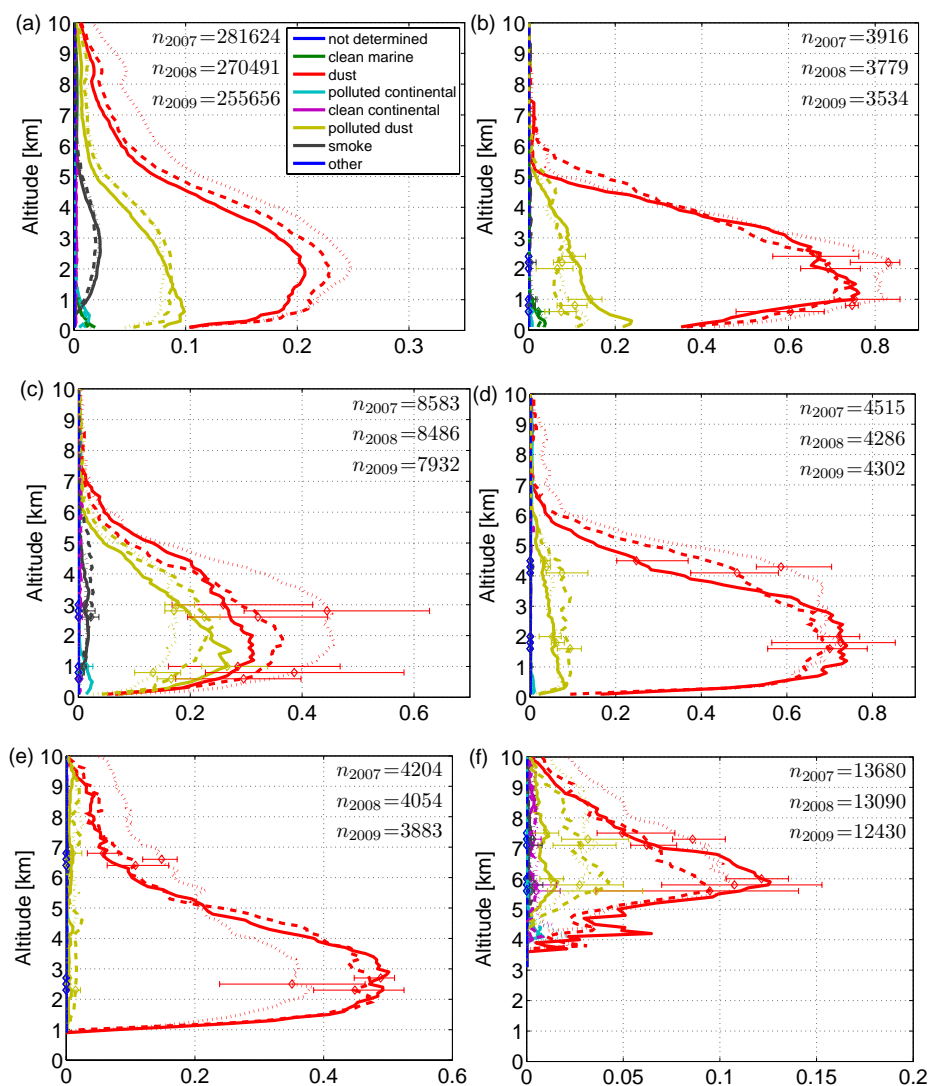
Fig. 2. Vertical distribution of the frequency of occurrence of the different aerosol types in (a) the entire region of interest, (b) the Arabian Sea, (c) the Ganges Plains, (d) the Indus Plains, (e) the Taklamakan Desert, and (f) the Tibetan Plateau. Note the different scalings of the respective x-axis. Data displayed separately for MAM 2007 (solid lines), 2008 (dotted lines), and 2009 (dashed lines). The numbers n_x indicate the total number of sample profiles that was considered for each averaged profile. The error bars indicate the geographical variability within the subregions.
