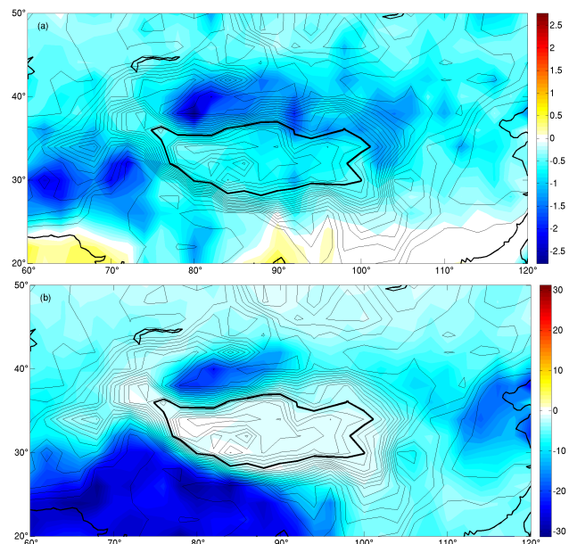
Fig. 8. Downward SW fluxes anomalies due to aerosols at (a) 5 km and (b) 0 km a.m.s.l. in \text{W/m}^2 . Simulation with MODIS surface albedo. Note the different scalings of the colorbars, each time adjusted to the respective extreme value. The thick lines indicate coasts and the Tibetan Plateau.
