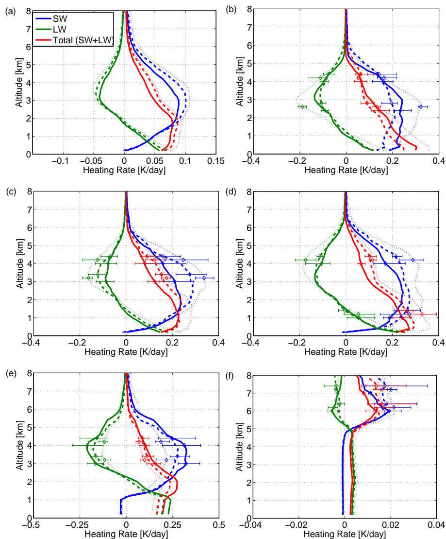
Fig. 11. Vertical distribution of the heating rates in K/day due to SW radiation (blue lines), LW radiation (green lines), and total radiation (red lines) in (a) the entire region of interest, (b) the Arabian Sea, (c) the Ganges Plains, (d) the Indus Plains, (e) the Taklamakan Desert, and (f) the Tibetan Plateau. Simulation with MODIS surface albedo. Note the different scalings of the respective x-axis. Data displayed separately for MAM 2007 (solid lines), 2008 (dotted lines), and 2009 (dashed lines).
