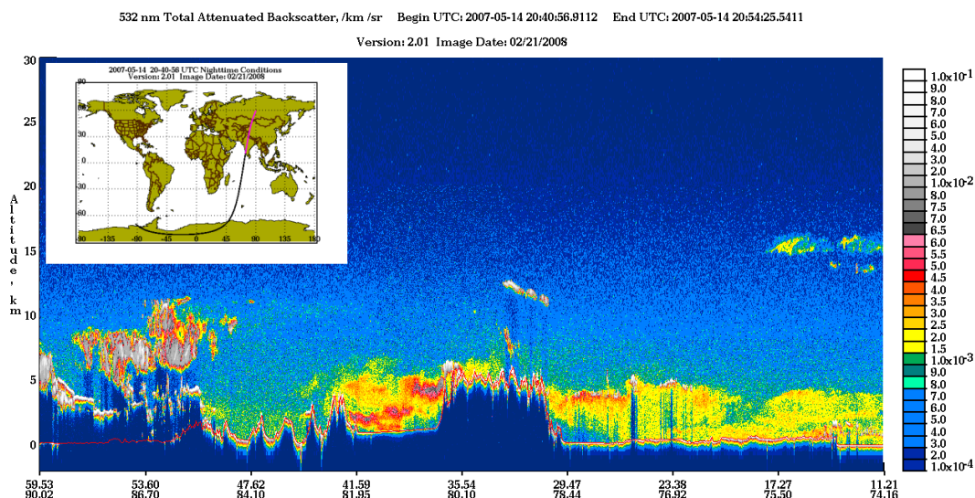
Fig. 4. CALIPSO backscatter signal for the case study of 14 May 2007. Vertically resolved total attenuated backscatter along the track. The TP (between approximately 30^{\circ} N and 35^{\circ} N, geographical coordinates are shown on the x-axis) is enclosed by aerosol layers, both from the southern and from the northern sides. Grey colour corresponds to clouds, yellow to red colours correspond to aerosol layers. Top-left corner: a map of the CALIPSO track used for the case study. The Indian subcontinent, the Himalaya and the Taklamakan Desert are covered. Image from http://www-calipso.larc.nasa.gov/ .
