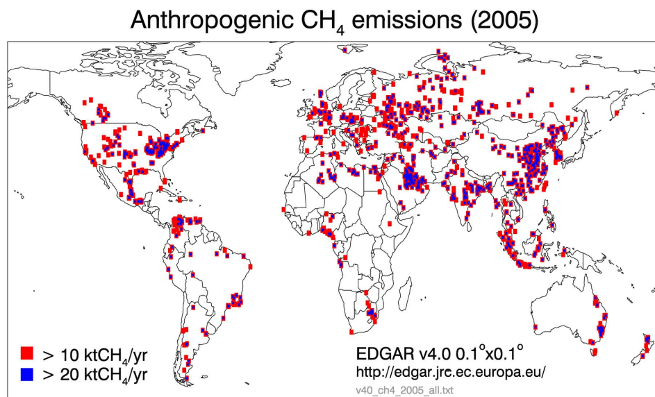
Fig. 15. Spatial distribution of strong localized anthropogenic methane sources according to the EDGAR data base (year 2005, gridded 0.1^\circ \times 0.1^\circ ). Shown are the locations of methane sources, which emit more than 10 \text{ ktCH}_4/\text{yr} (red boxes) and more than 20 \text{ ktCH}_4/\text{yr} (blue boxes). (Source: EC-JRC/PBL, EDGAR version 4.0, http://edgar.jrc.ec.europa.eu/ , 2009).
