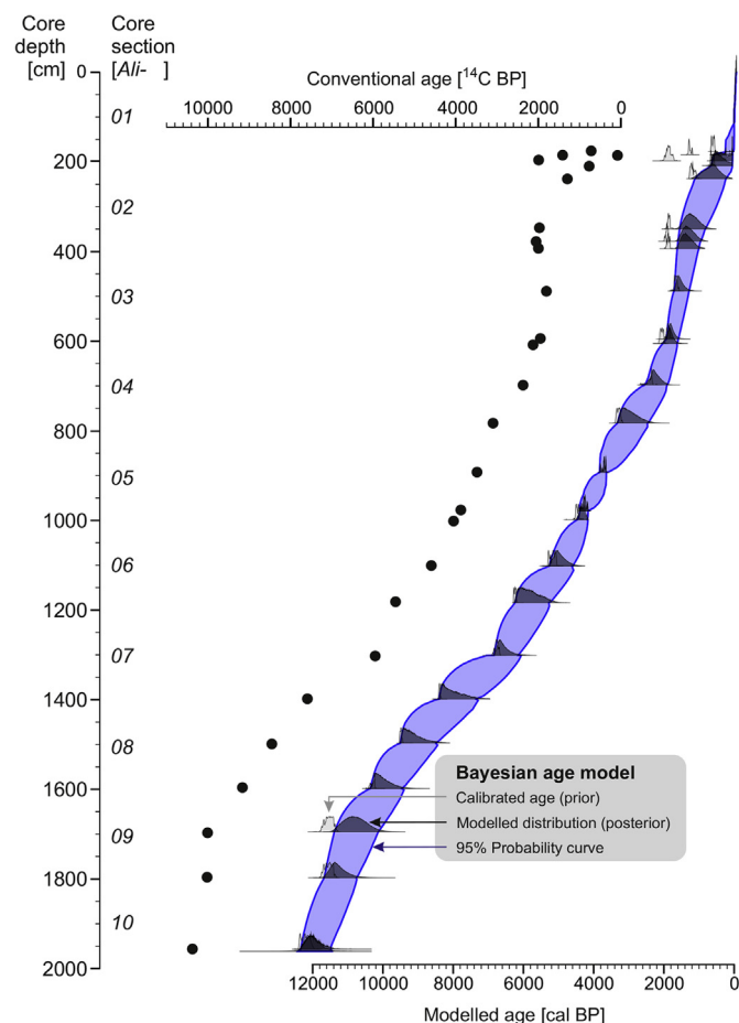
Fig. 3. Bayesian age model of the Sidi Ali core (Fletcher et al., 2017): the black dots show conventional ^{14}\text{C} ages [BP]. The light greyish curves show ^{14}\text{C} calibrated ages (prior). The dark greyish curves show modelled age distributions (posterior). The light purple area show the 95% probability distribution. Calibration (2 sigma) of the conventional radiocarbon ages was performed using intcal13.14c . (For interpretation of the references to colour in this figure legend, the reader is referred to the web version of this article.)
