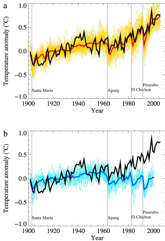
Figure 27. Global mean temperature anomalies, as observed (black line) and as modeled by (a) 58 simulations from 14 different models with both anthropogenic and natural forcings and (b) simulations from 5 models with natural forcings only. The individual simulations are shown in color, with bold curves of the same color indicating the ensemble mean. The observed and simulated time series in Figure 27a are expressed as anomalies relative to the 1901–1950 mean. The simulations in Figure 27b are expressed as anomalies relative to the corresponding model simulation that also includes anthropogenic forcing. Only models whose control simulations have a trend of less than 0.2^{\circ}\text{C century}^{-1} are included [from IPCC, 2007, Figure 9.5; after Stott et al. , 2006].
