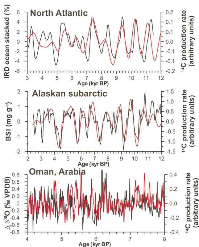
Figure 19. Comparison between the 14 C production rate (red curve in each plot) and (top) North Atlantic ice-rafted debris (IRD) [Bond et al., 2001], (middle) biogenic silica (BSi) from Arolik Lake in the Alaskan subarctic [Hu et al., 2003], and (bottom) detrended stalagmite δ 18 O record from southern Oman [Fleitmann et al., 2003]. Minima in solar activity (higher 14 C production rates) coincide with greater extent in sea ice in the North Atlantic (positive IRD values), wetter and colder conditions in the Alaskan subarctic (more negative BSi values), and reduced monsoon precipitation in southern Oman (more positive δ 18 O values).
