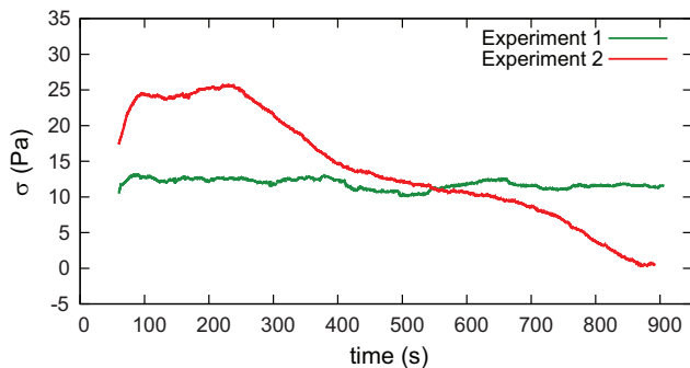
Fig. 8. Convergence parallel normal stress recorded in the back of the overriding plate in Experiments 1 and 2. In Experiment 1, the recorded compressive stress is due to the flexural rigidity of the plate which resists bending. In Experiment 2, the stress at the beginning of the experiment is due to the combined effects the flexural rigidity and high interplate friction. However, during Experiment 2, the compressive stress decreases because the subducted slab becomes longer and its pull becomes stronger.
