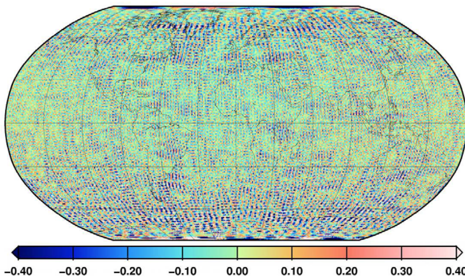
Fig. 22 Geoid height differences [m] between ITG-Grace2010s and GOCE (SPW) up to degree/order 180
