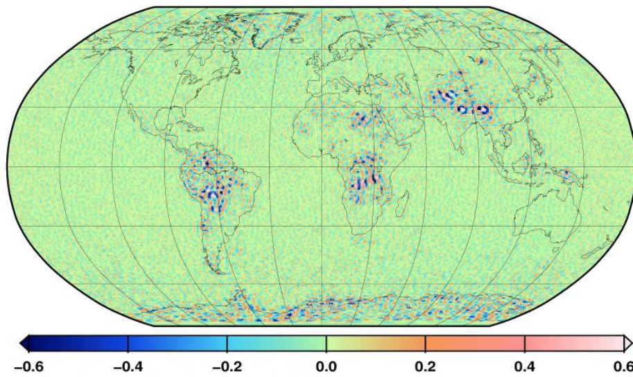
Fig. 20 Geoid height differences [m] between GOCE (DIR) and EGM2008 up to degree/order 240
