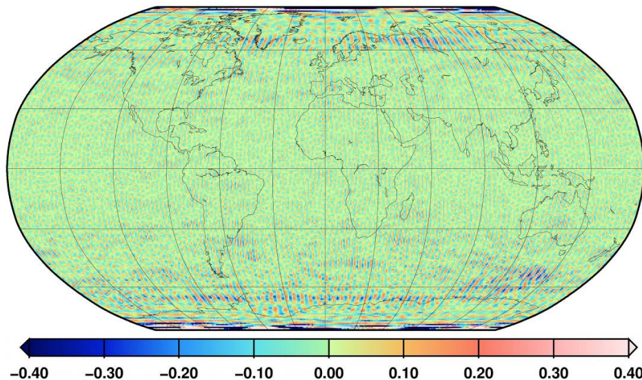
Fig. 23 Geoid height differences [m] between ITG-Grace2010s and GOCE (TIM) for the spherical harmonic degree range 80 to 160
