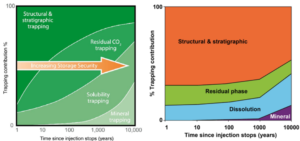
Fig. 2. Left) Diagram showing the concept of increasing amount of immobile CO 2 and thereby increased security of the storage facility with regard to the responsible mechanisms [5]. Right) Trapping-mechanism/time diagram based on data from simulations of the processes of mineral reaction and dissolution [7].
