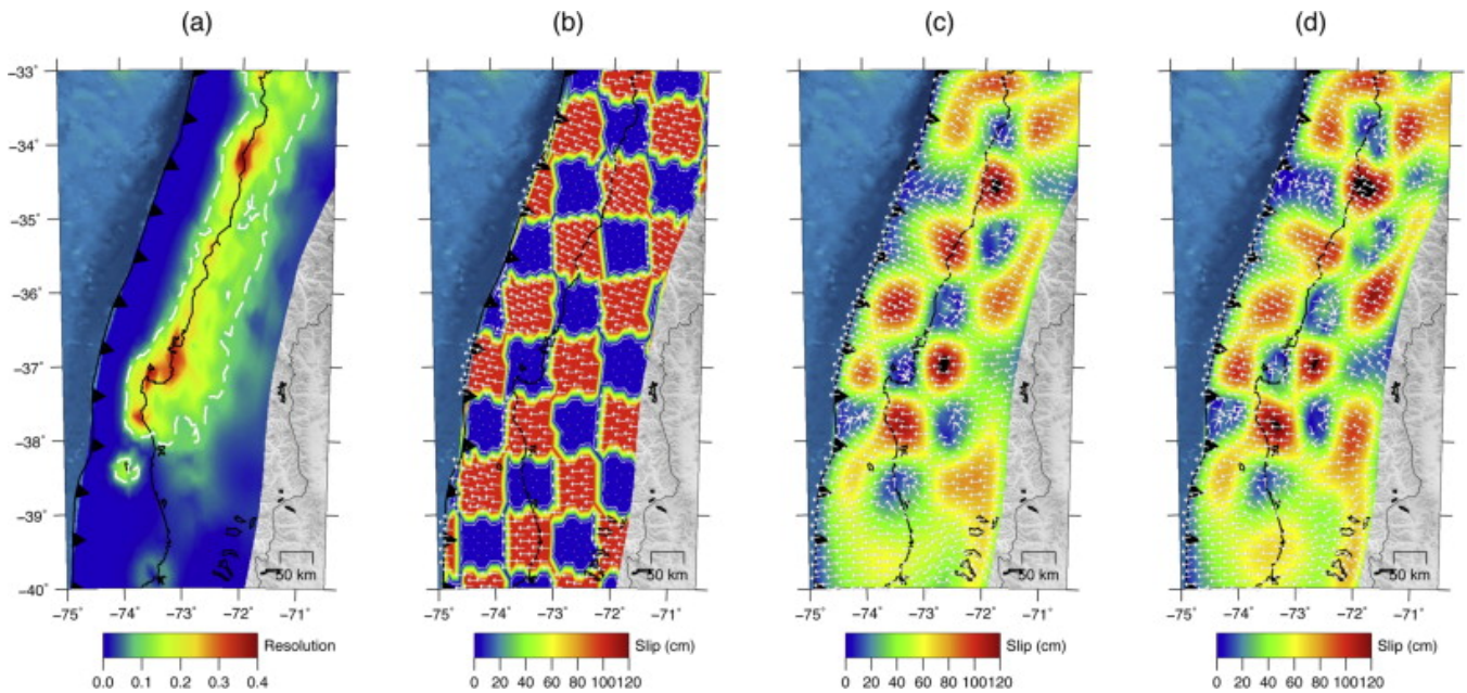
Figure 3. (a) The diagonal of the model resolution matrix, averaged for both up-dip and along-strike model parameters, and averaged over all the inversions that are summed to produce the model. Model resolution matrix, R , is equal to (G^T G)^{-1} G^T G , where G is the matrix of Green's functions relating the dislocations in the elastic halfspace to the surface displacements (Menke, 1989). Higher values indicate better model resolution. The white dashed line encloses the region of the interface with superior resolution (resolution > 0.1 ). (b) The input slip for the checkerboard test. Unit slip is implemented up-dip. (c) The inverted slip for the checkerboard test, using the synthetic displacements (without noise) 60 most commonly available cGPS stations. (d) The inverted slip for the checkerboard test, using the synthetic displacements (with noise) 60 most commonly available cGPS stations. Random uniformly distributed noise is added to each synthetic displacement, with the maximum noise being \pm 20\% of the maximum displacement.
