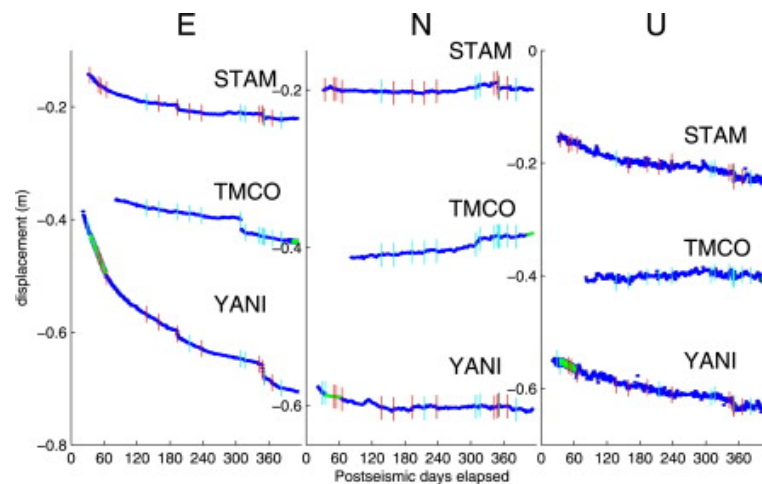
Figure 2. East, North, and Vertical components of the continuous GPS data for 3 stations. Blue time series points correspond to real data, and green points correspond to linearly interpolated data. Interpolated data has been given an error 3 times that of the average, so that it is weighted less in model. Vertical red lines indicate plate interface aftershocks with M_w \geq 5.5 (from catalogue of Agurto et al., 2012 ) which have occurred within a lateral radius of 1^\circ , and vertical cyan lines indicate earthquakes that have occurred further away. Aftershocks are often seen to line up with jumps and subsequent accelerations in the time series.
