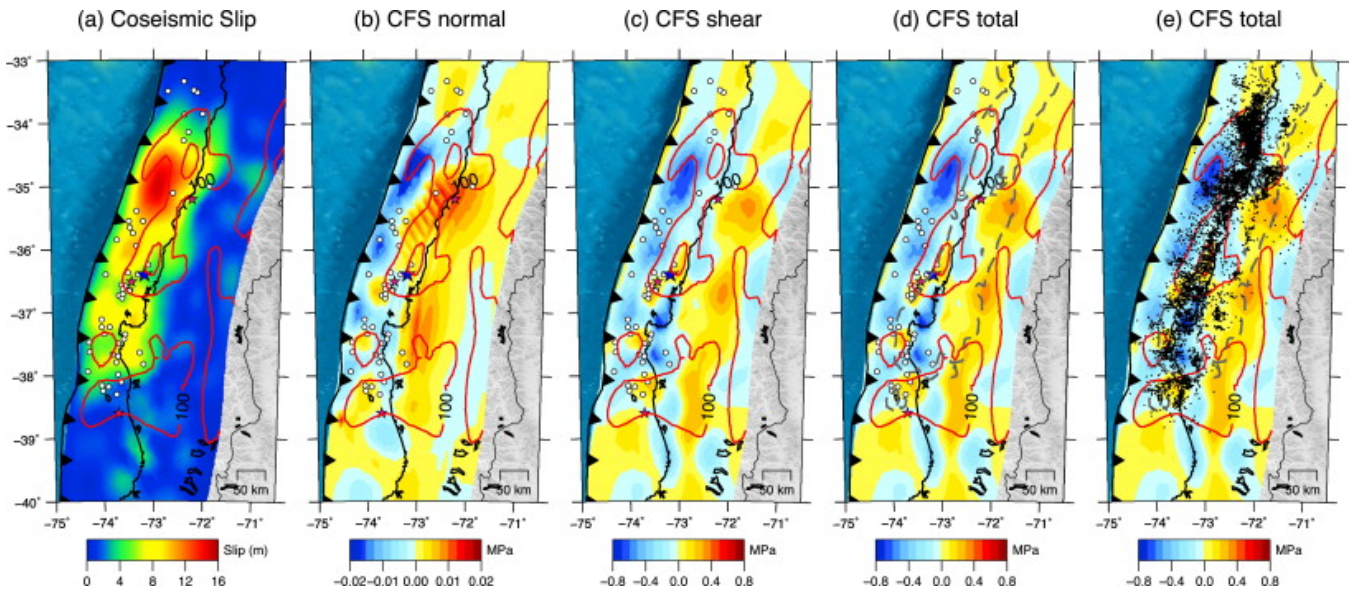
Figure 6. (a) Co-seismic slip. White circles are the plate interface thrust events larger than M_w = 5.5 , pink stars are the largest aftershocks on the plate interface (from north to south M_w = 7.2, 6.8, 7.1 ), and the blue star is the epicentre of the mainshock (hypocentre from Vigny et al. , 2011). All other epicentres from Agurto et al. , 2012). Red contours represent 100 cm and 200 cm of afterslip (in any direction). (b) Normal component of the \Delta CFS calculation assuming a coefficient of friction \mu = 0.1 . Positive indicates a change in stress bringing the interface closer to failure. The circles, stars, and red contours indicate the same things stated for panel (a). (c) Shear component (in up-dip direction) of the \Delta CFS calculation. Positive indicates a change in stress bringing the interface closer to failure. The circles, stars, and red contours indicate the same things stated for panels (a)–(b). (d) Total \Delta CFS . Positive indicates a change in stress bringing the interface closer to failure. The circles, stars, and red contours indicate the same things stated for panels (a)–(c). The grey dashed line encloses the region of the interface with superior resolution (resolution > 0.1 ). (e) Total \Delta CFS . Black dots represent the plate interface seismicity (events which are \pm 5 km from the plate interface as defined by Tassara and Echaurren (2012)). Seismicity from the catalogue of Lange et al. (2012). The red contours indicate the same things stated for panels (a)–(d). The grey dashed line encloses the region of the interface with superior resolution (resolution > 0.1 ).
