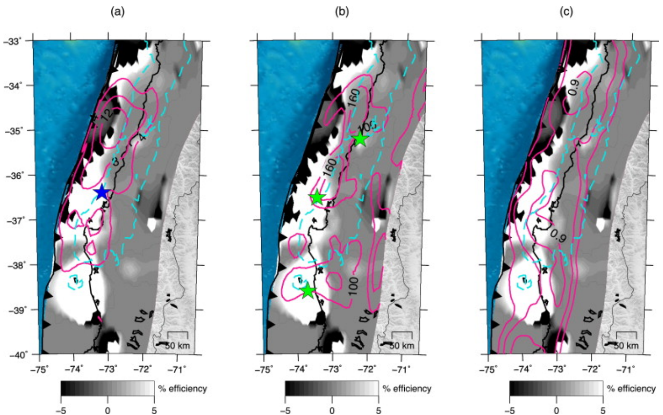
Figure 7. (a) Post-seismic Seismic Efficiency (PSE) with magenta contours of co-seismic slip (4, 8, and 12 m). Blue star is the mainshock hypocentre (Vigny et al., 2011). The blue dashed line encloses the region of the interface with superior resolution (resolution > 0.1). (b) PSE with magenta contours of afterslip (100 and 160 cm). Green stars are the largest aftershocks on the plate interface (pink stars in Fig. 6). The large aftershock at 35.2°S happens over one year later – it is not included in the calculation of PSE. The blue dashed line encloses the region of the interface with superior resolution (resolution > 0.1). (c) PSE with contours of interseismic locking degree (contour intervals: 0.3, 0.6, and 0.9). The blue dashed line encloses the region of the interface with superior resolution (resolution > 0.1).
