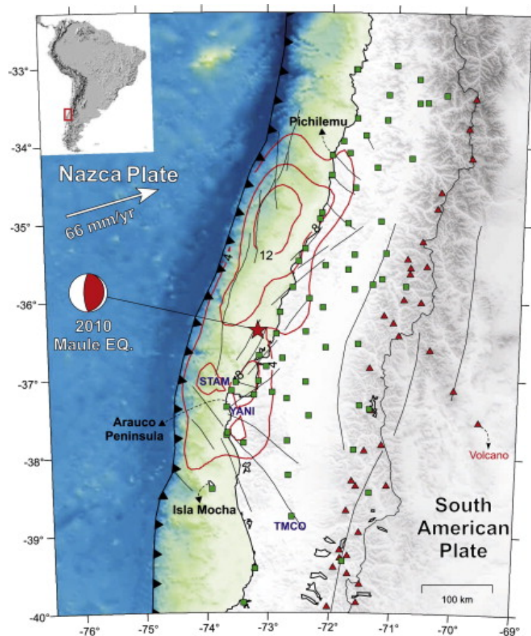
Figure 1. Tectonic setting for the Maule 2010 subduction earthquake. Green squares indicate locations of continuous GPS stations. Co-seismic slip contours of 4 m, 8 m, and 12 m are plotted in red. Mainshock hypocentre is given by the red star (Vigny et al., 2011) and focal mechanism from the gCMT catalogue is shown. Crustal faults are indicated with black lines. Red triangles indicate Quaternary volcanoes.
