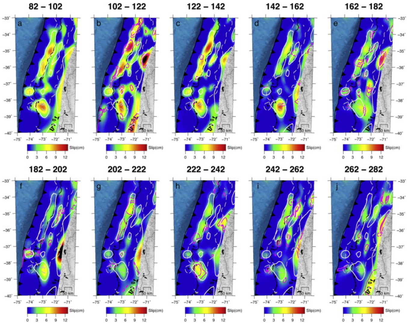
Figure 5. The panels (a)–(j) represent 20 day time windows of up-dip afterslip as averaged from the jackknife testing between days 82–282 of the post-seismic period. Pink contours indicate robustly identified pulses of afterslip, with the first contour representing the ratio (slip difference: standard deviation) of 1:1 and the second contour a ratio of 2:1. There are no contours on panel a because this is the first time window of the analysis. White contour represents the 25 cm contour of up-dip afterslip between post-seismic days 82–282. Light grey dashed contour encloses the region of the interface with superior resolution (resolution > 0.1).
