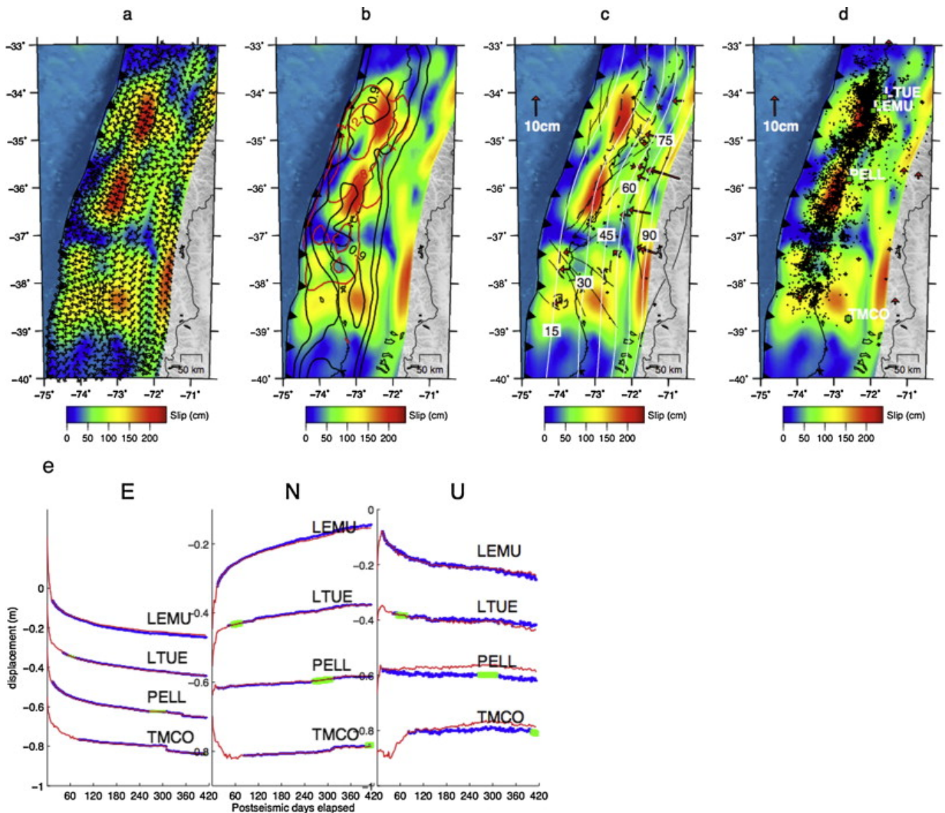
Figure 4. (a) Cumulative afterslip between February 27th 2010 (day of mainshock) and April 15th 2011. Arrows show direction of slip on the interface. (b) Afterslip model overlain with the red mainshock slip contours (4, 8, and 12 m) and the black interseismic locking degree contours (0.3, 0.6, and 0.9) (Moreno et al., 2010). (c) Afterslip model and the horizontal misfit vectors (misfit = data – prediction). Misfits are plotted rather than the data and prediction vectors because the data at certain stations are incomplete for the model duration. Misfit is calculated between the first and last days of available data. White lines represent depth contours of the plate interface, spaced in 15 km intervals (slab model: Tassara and Echaurren, 2012). Black dashed line encloses the region of the interface with superior resolution (resolution > 0.1). (d) Afterslip and the vertical misfit vectors. Black dots represent the aftershock seismicity from Lange et al. (2012). (e) Selected time-series of model predictions and data. Blue, green, and red points represent the data, interpolated data, and the model predictions respectively.
