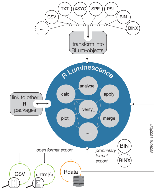
Figure 2. R ‘Luminescence’ package structure with indicated input/output interfaces. Once the raw measurement data have been transformed into an RLum-object, data can be passed without further transformation from one function to another within the package environment.
