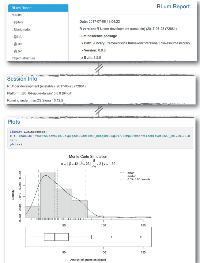
Figure 3. Screenshot of an HTML report produced using the function report_RLum() from the R package ‘Luminescence’. The output object used for the example was produced by the function calc_AliquotSize() . The output has been manually reduced for this figure.
