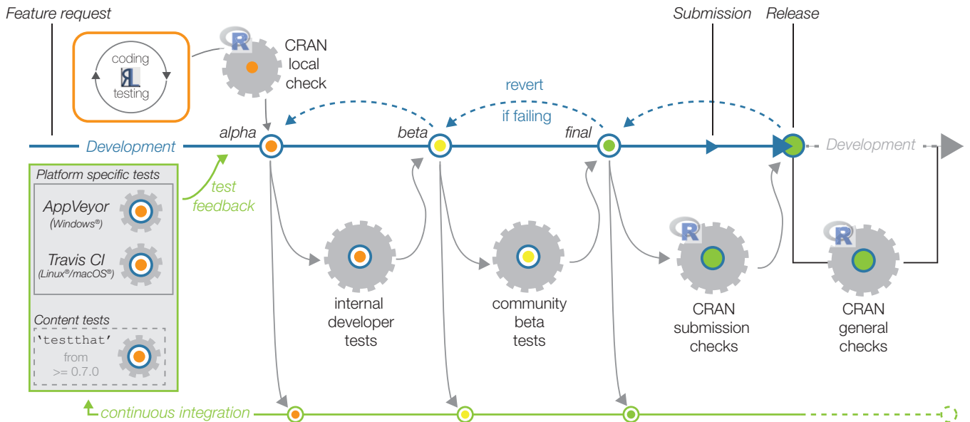
Figure 5. Development and testing process as implemented in the R package ‘Luminescence’. Once the development process has been initialised by a feature request (e.g., a new function), the new package version evolves over several development versions. Starting with an alpha version, stability and quality are improved until a final version, ready for submission to CRAN, is reached. The entire development process is supported by automatic platform and unit tests, which are run continuously.
