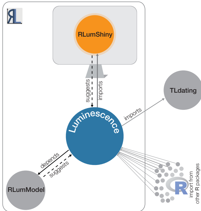
Figure 4. R package ‘Luminescence’ dependency sketch. For example: The package ‘RLumShiny’ is suggested by the package ‘Luminescence’ and therefore imported. Thus, the package ‘Luminescence’ can run without the package ‘RLumShiny’, but not the other way around.
