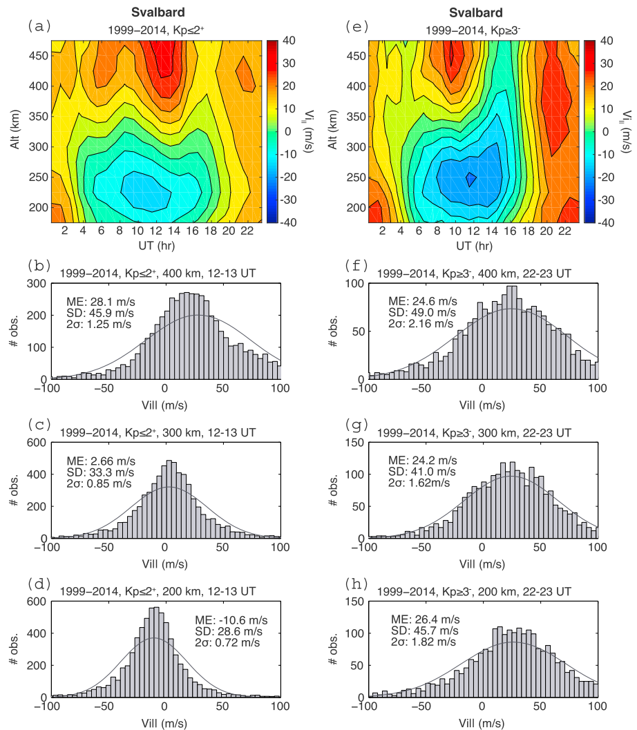
Figure 3. Same as Figure 2 except for Svalbard during 1999–2014. The average standard deviations are (a) 37.8 and (e) 44.5 m/s. The average 2\sigma errors are 1.09 and 1.96 m/s for Figures 3a and 3e, respectively.
