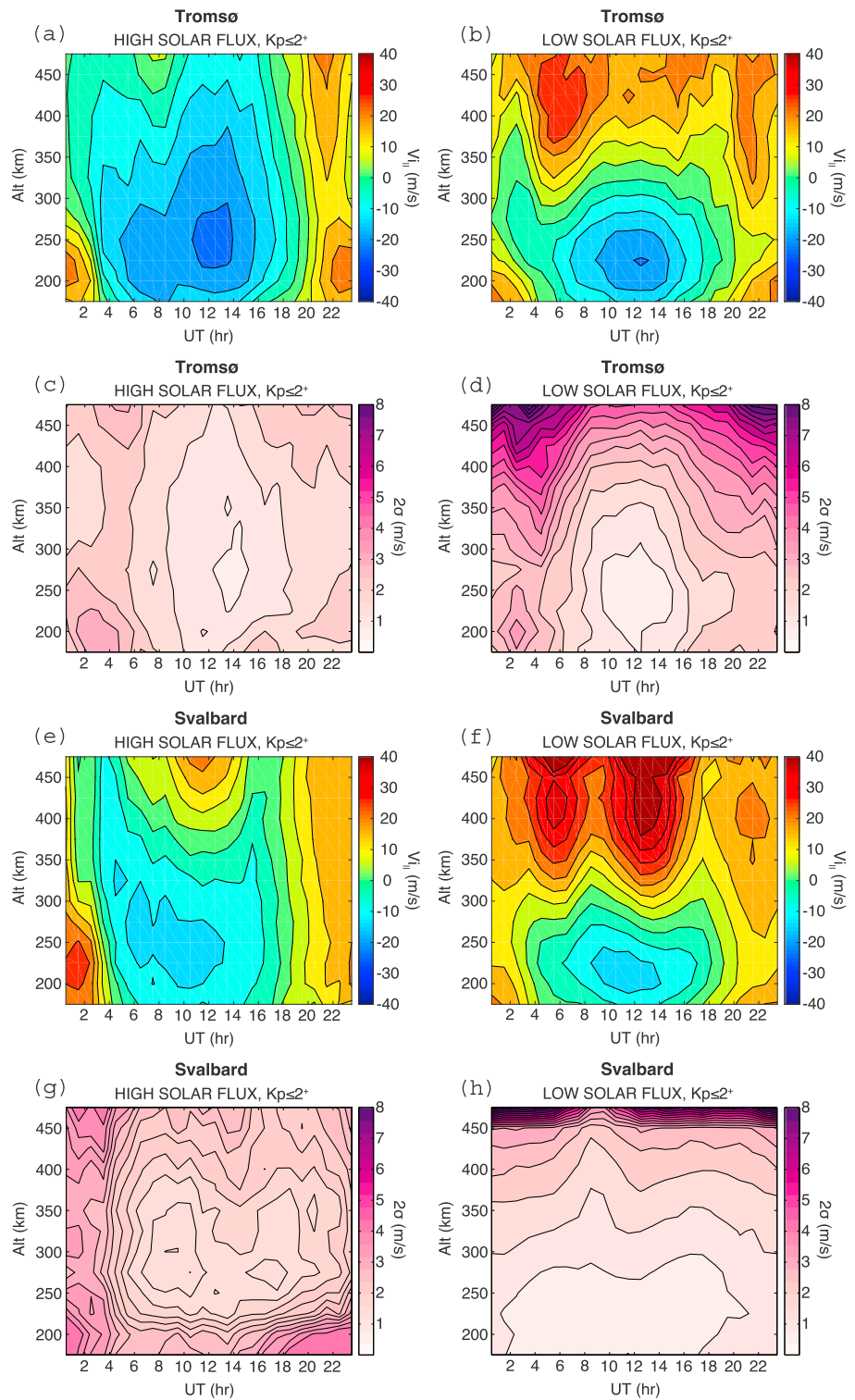
Figure 5. The dependence of the average field-aligned ion velocity (positive upward) on solar activity (a and b) for Tromsø and (e and f) for Svalbard. The 2\sigma errors are shown (c and d) for Tromsø and (g and h) for Svalbard. The average standard deviation is 21.7 and 35.5 m/s for Figures 5a and 5b, respectively, and 34.1 and 38.7 m/s for Figures 5e and 5f, respectively. The average 2\sigma error is 1.83 and 3.14 m/s for Figures 5a and 5b, respectively, and 2.44 and 2.02 for Figures 5e and 5f, respectively.
