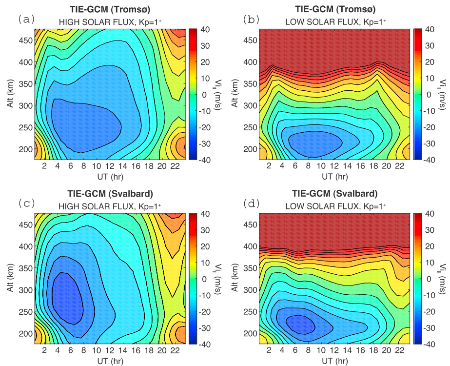
Figure 6. The dependence of the TIE-GCM field-aligned ion velocity (positive upward) on solar activity for (a and b) for Tromsø and (c and d) for Svalbard.
