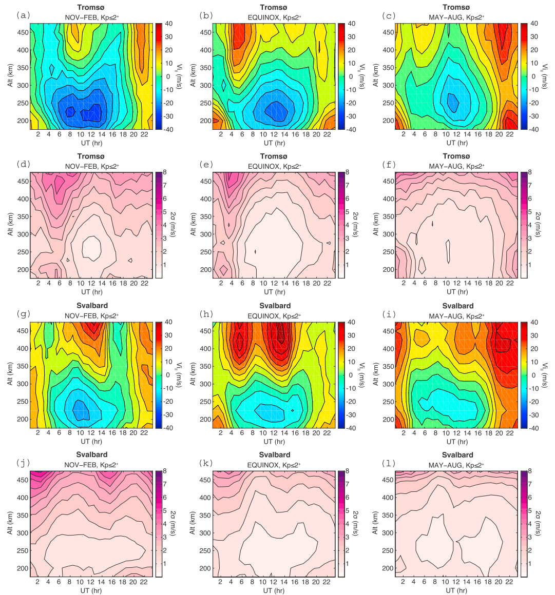
Figure 4. The dependence of the average field-aligned ion velocity (positive upward) on season for (a–c) for Tromsø and (g–i) for Svalbard. The 2\sigma errors are shown in (d–f) for Tromsø and in (j–l) for Svalbard. The average standard deviations are 33.2, 28.7, and 21.1 m/s for Figures 4a–4c, respectively, and 46.2, 35.0, and 27.1 m/s for Figures 4g–4i, respectively. The average 2\sigma errors are 2.37, 1.89, and 2.01 m/s for Figures 4a–4c, respectively, and 2.39, 1.61, and 1.48 m/s for Figures 4g–4i, respectively.
