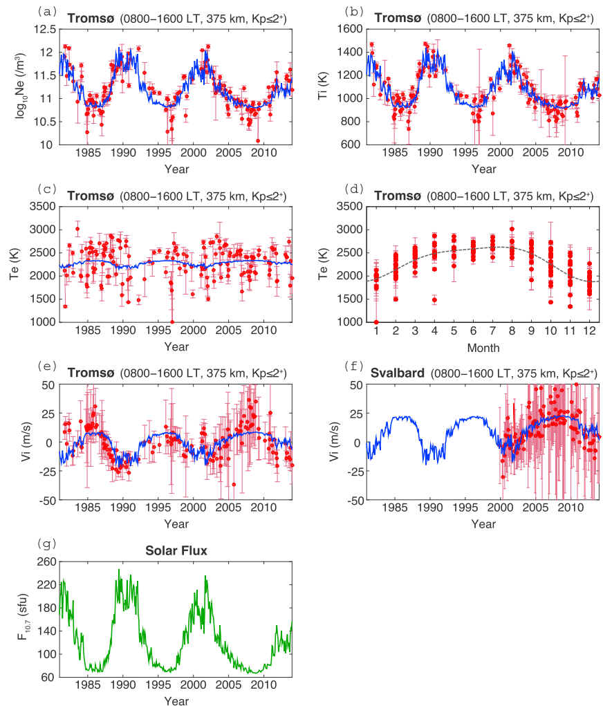
Figure 1. Time series of (a) plasma density ( N_e ), (b) ion temperature ( T_i ), (c) electron temperature ( T_e ), and (e) field-aligned ion velocity ( \mathbf{V}_{||} , positive upward) at 375 km, obtained from the EISCAT radar at Tromsø under geomagnetically quiet conditions ( K_p \leq 2^+ ) during 1981–2014. Shown are monthly averages of the daytime measurements (0800–1600 LT). The error bars represent the standard deviation, and the blue lines represent the least squares fit of the function C = a + bF_{10.7} to the corresponding ionospheric data (see text for details). (d) Seasonal variation of T_e , with the least squares fit of the function D = \sum_{k=0}^2 \{a_k \cos(kM/12) + b_k \sin(kM/12)\} (see text for details). (f) Same as Figure 1e except for Svalbard. (g) Monthly values of the F_{10.7} index.
