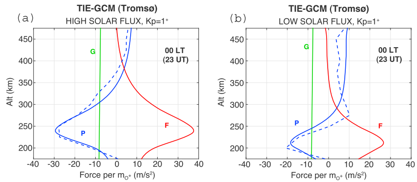
Figure 9. Same as Figure 7 except for 0000 LT.
