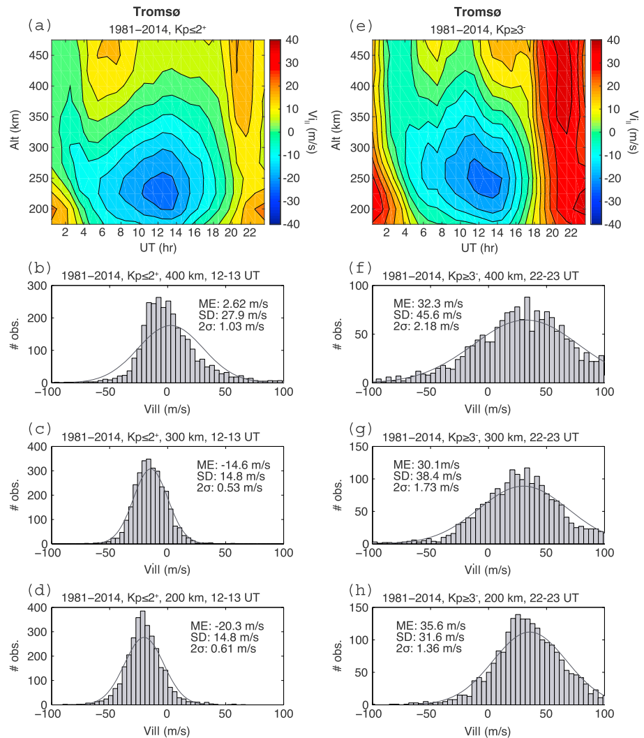
Figure 2. (a) The average field-aligned ion velocity (positive upward) at Tromsø during 1981–2014 as a function of UT and altitude for K_p \leq 2^+ . (b–d) The distribution of V_{||} (positive upward) between 12 and 13 UT for K_p \leq 2^+ at 400, 300, and 200 km. (e) Same as Figure 2a but for K_p \geq 3^- . (f–h) The distribution of V_{||} (positive upward) between 22 and 23 UT for K_p \geq 3^- at 400, 300, and 200 km. The average standard deviations are 29.7 and 34.7 m/s for Figures 2a and 2e, respectively. The average 2\sigma errors are 1.26 and 1.78 m/s for Figures 2a and 2e, respectively.
