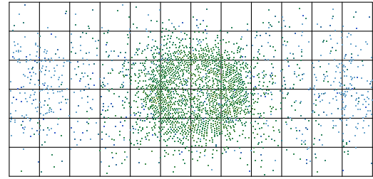
electron-like event
