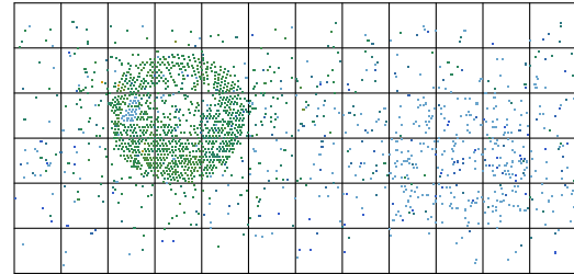
muon-like event
