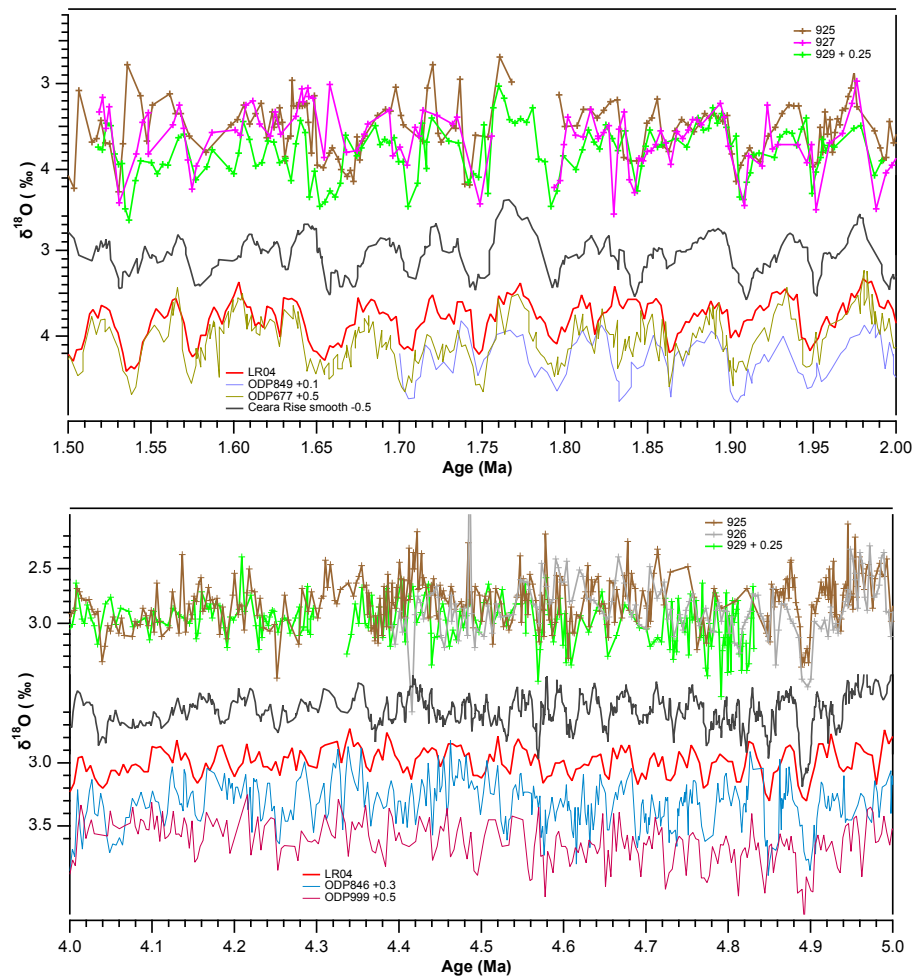
Figure 9. Detail from Fig. 8 comparing individual holes to one another and a smoothed composite to LR04 for the intervals 1.5 to 2.0 and 4.0 to 5.0 Ma. For better illustration we plotted the initial alignment target records of the LR04 stack. For the 1.5 to 2.0 Ma interval these are the records from ODP sites 677 and 849; for the interval 4.0 to 5.0 Ma these are the records from ODP sites 846 and 999. Some records have been shifted as indicated in the figure for better comparison of the data with each other. Note the differences between LR04 and the Ceara Rise average at 1.80–1.85 Ma, although the initial alignment targets are more similar to the Ceara Rise smooth. Also note the difference between 4.0 and 4.5 Ma. The Site 999 record is from a single hole and the splice of the Site 846 record might be erroneous. The age model for the Ceara Rise is very robust in this interval (see Fig. 10) pointing to potential inconsistencies in the age model construction of the Site 846 and Site 999 records.
