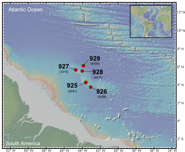
Figure 1. The location of ODP Leg 154 sites.
