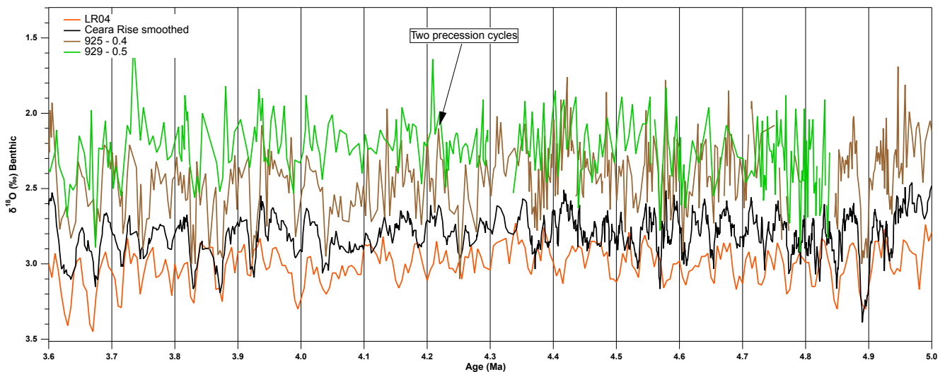
Figure 12. A comparison of LR04 and Ceara Rise (smooth) to Site 925 and Site 929 benthic isotope data. LR04 assignment of variability in the interval from 4.0 to 4.5 Ma to precession peaks may have resulted in the mismatch with the Ceara Rise stack.
