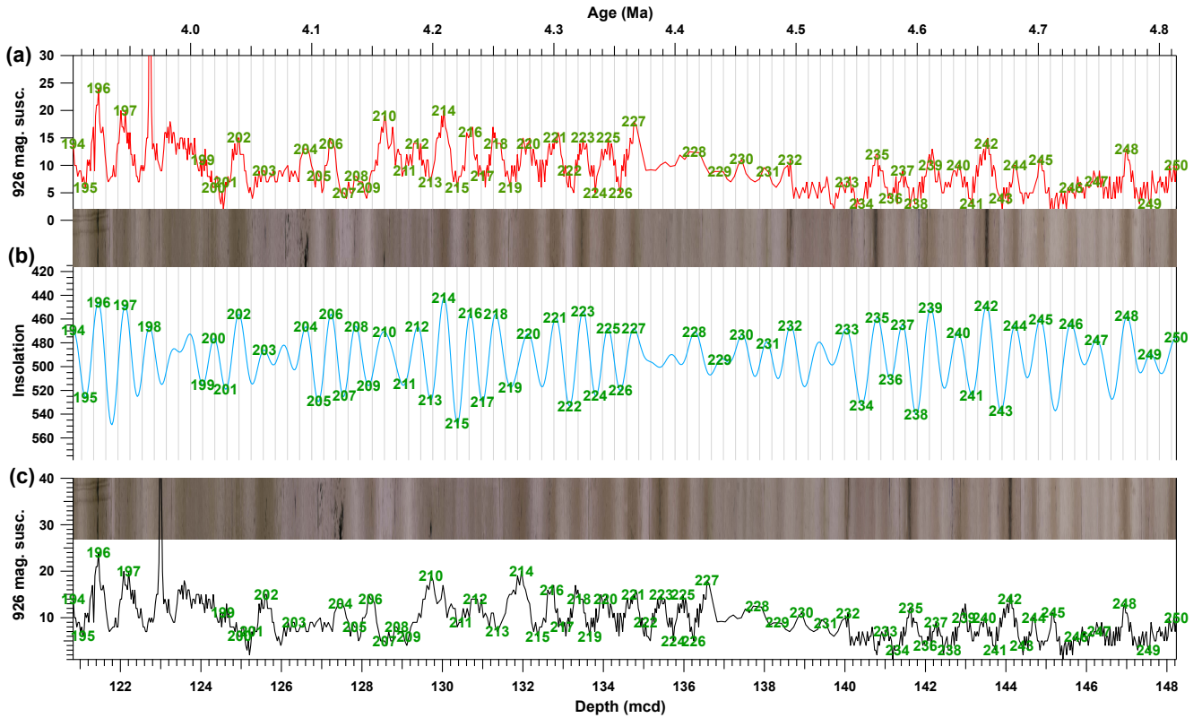
Figure 10. Detail from CODD tuning of Site 926 magnetic susceptibility and core images to insolation. Panel (c) is data versus depth, (b) shows insolation 65° N 21 June inverted, and (a) shows image and magnetic susceptibility versus tuned age. Green numbers mark position of tie points. Numbers identify tie points between the data and the insolation curve. Light/dark layering in the composite core image is tied to precession cycles prominent in the insolation curve.
