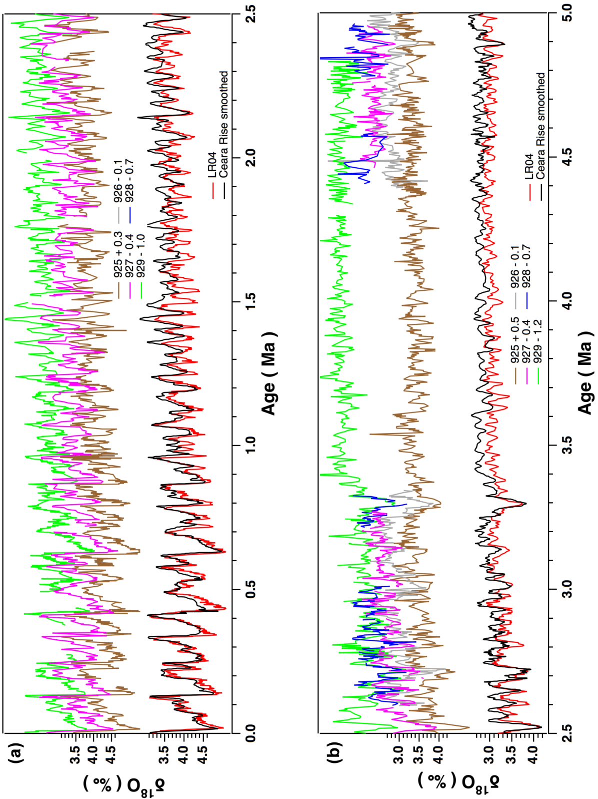
Figure 8. Benthic oxygen isotope data from all Ceara Rise sites compared with one another and a smoothed composite of all data compared to LR04. (a) 0 to 2.5 Ma; (b) 2.5 to 5 Ma. Note the \delta^{18}\text{O} scale change between (a) and (b). Individual site traces have been offset as indicated in the legend.
