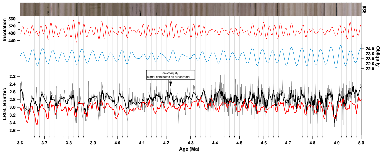
Figure 11. A comparison of LR04 (Red) to Ceara Rise (grey and black (smooth)) to obliquity and insolation from Laskar et al. (2004). Note that the interval 4.0 and 4.5 Ma exhibits poorly defined obliquity cycles leaving insolation dominated by precession.
