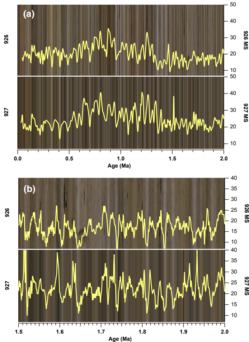
Figure 6. (a) Smoothed MS data and images plotted versus age from 0–2 Ma. (b) 1.5–2 Ma detail using non-smoothed data. Fine layers, on the order of 10 kyr, are correlated between sites 927 and 926.
