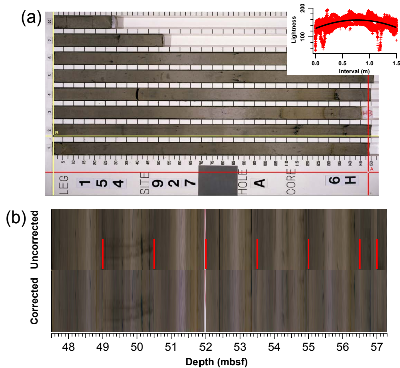
Figure 2. Creating a composite core image from a core table image. (a) Image loaded into IGOR. Red cursor moves horizontally to set bottom locations in pixels of each section. Yellow cursor moves horizontally and vertically to the lower left corner of each section before cutting. Inset – lengthwise lightness profiles for each of the cut sections and a best fit line used for the lighting correction. (b) Composite core image scaled to m.b.s.f. Vertical red lines indicate section breaks. Lower image has been corrected for uneven lighting in the core box photo.
