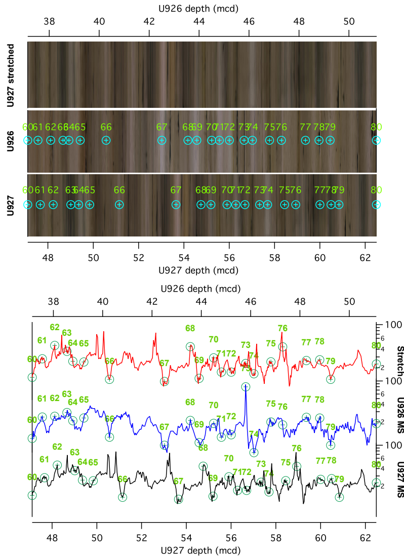
Figure 5. Spliced images and MS data from ODP sites 926 and 927. There have been small adjustments to the published splices for each site. Site 927 data and image are plotted versus the Site 927 depth scale on the bottom of each graph and versus the Site 926 depth scale at the top. Green numbers indicate tie points between the sites used to stretch the Site 927 image and data.
