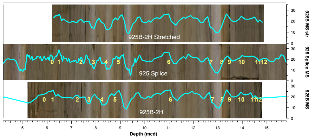
Figure 4. Core 925B-2H was not used for the Site 925 splice, and while there is good alignment between the core image and data and the spliced image and data at 13–14 m c.d., shallower portions of the core are not well aligned with the splice. Yellow numbers indicate tie points used to stretch the image and data so that they are in better agreement with the splice. Choice of tie points is cursor driven and stretching can be recalculated in real time.
