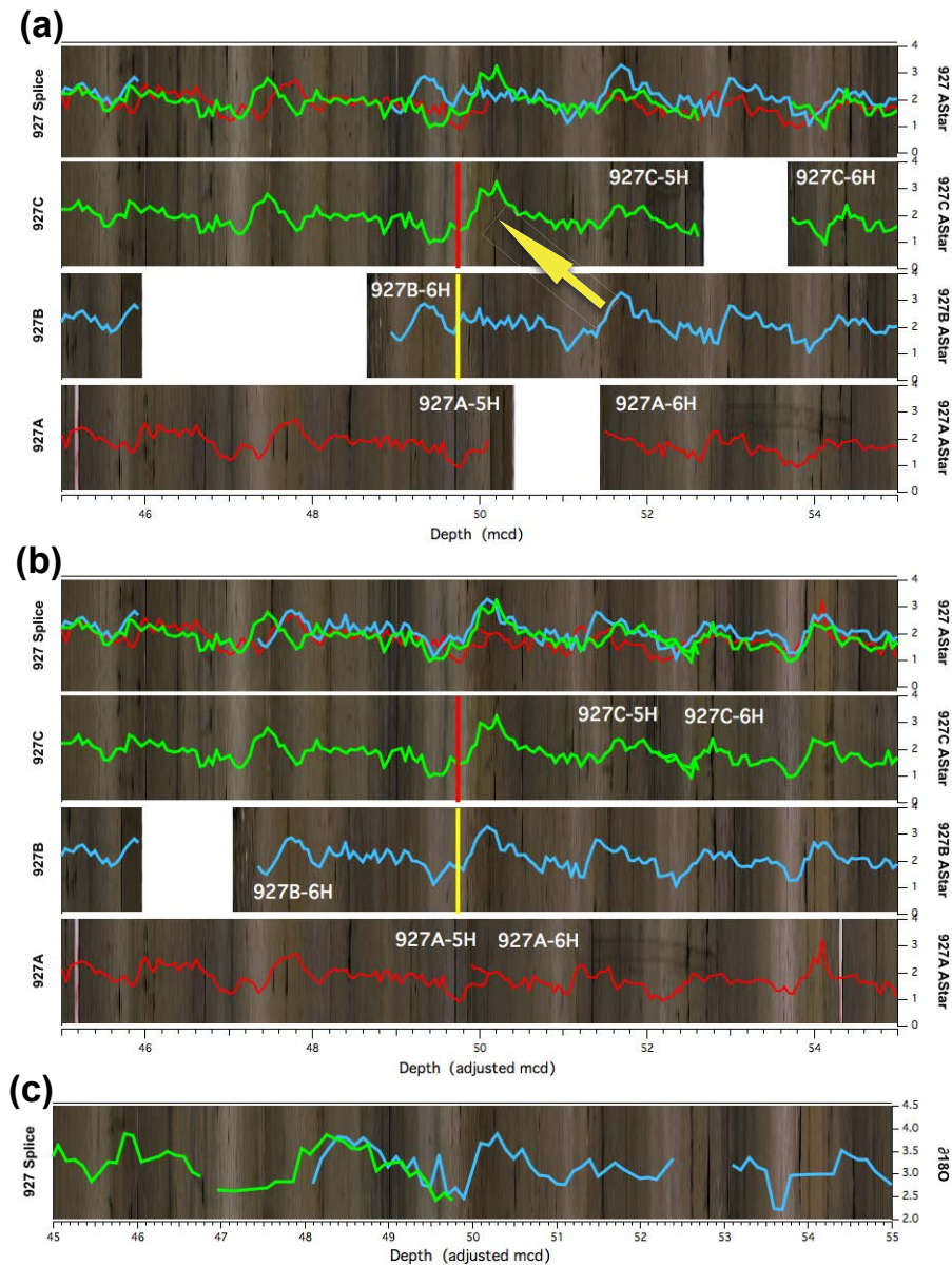
Figure 3. (a) Reflectance spectrophotometer (RSC) a^* data (LAB color model) and core images plotted against the published splice m.c.d. The yellow arrow indicates misaligned features. The yellow vertical line represents the top of a splice section and the vertical red line shows the bottom of the previous splice section. (b) The revised splice. The splice goes from Core 927C-05H to Core 927B-06H in both cases, but the offset for Core 927B-06H has been reduced by 1.6 m in the revised splice to account for the repeat sampling of a cycle. Note the poor agreement of the data between 49 and 51 m b.s.f. in the original splice. (c) Benthic \delta^{18}\text{O} revised. Samples were collected based on the original splice, resulting in data duplication between 48 and 50 m adjusted m.c.d.
