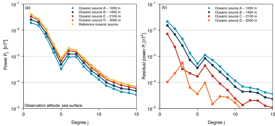
Figure 6. (a) Power spectra of the annual mean ocean-induced magnetic fields at sea surface. (b) Absolute differences between the power spectra of the scenario-wise ocean-induced magnetic fields and the reference.
