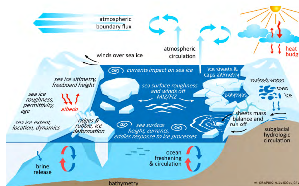
FIGURE 1. Sketch of different processes and interactions involving the cryosphere. G-TERN aims to improve understanding of the sea ice related processes and interactions at regional to climate scales, with focus on highly dynamic variations (ice production, deformation, melt), their driving forces and feedback mechanisms, including extreme events, ocean and atmospheric circulation. Other processes of the cryosphere related to sea ice snow cover and brine content, ice sheets and caps, hydrology and snow, biochemistry, and permafrost are secondary objectives of the G-TERN mission. Figure from G-TERN EE9 Proposal.
