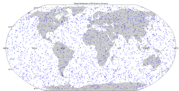
FIGURE 9. Example of geographical distribution of G-TERN RO profiles accumulated in 24 hours if all the twelve beams were devoted to capture GNSS occulting signals, enabling side-looking events. From this single receiving system it would be possible to acquire ~3000 RO profiles per day.
