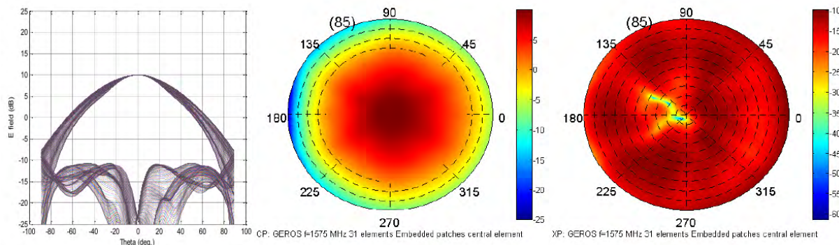
FIGURE 11. Embedded elementary radiator radiation pattern (central element; f = 1575 MHz).
