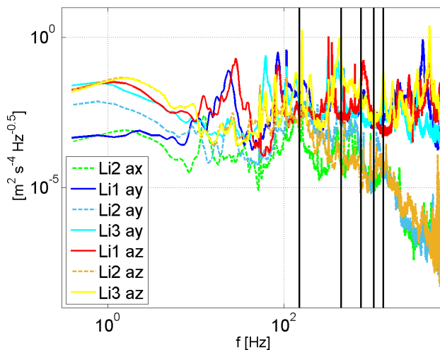
Figure 7. Acceleration spectra measured at the three humidity sensors Li1, Li2 and Li3 during the Do128 flight on 23 October 2015 for the same flight section as in Fig. 6. Blue and red indicate the accelerations of Li1 ( y and z respectively), cyan and yellow indicate the accelerations of Li3 ( y and z respectively), and the dashed lines in green, bright blue and other indicate the accelerations of Li2 ( x , y and z ). The vertical black bars indicate the critical frequencies of 150 Hz and odd harmonics 450 Hz, 750 Hz, 1050 Hz and 1350 Hz according to the manufacturer. The data were obtained during the part of the flight indicated in yellow in Fig. 3.
