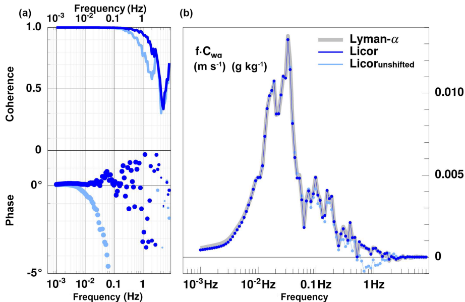
Figure 11. Phase shift and coherence spectra of the shifted (darker blue) and unshifted (light blue) signal of the LI-COR sensor on the Helipod (a) and cospectra of humidity from the different sensors and vertical wind speed multiplied by the frequency (b) on the Helipod flight. The area under the curves is proportional to the humidity fluxes. The flight part indicated in the time series in Fig. 5 in grey was used.
