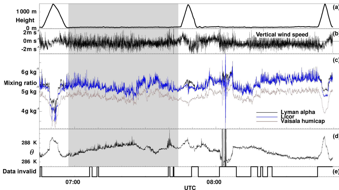
Figure 5. Overview of the flight with the Helipod on 14 August 2014. Panel (a) shows the height and (b) the vertical wind speed, indicating the strength of atmospheric turbulence. Panel (c) shows the time series of the mixing ratio measured by Lyman-alpha (black), Vaisala Humicap (purple) and the open-path Li3 (blue). Panel (d) represents the potential temperature. Panel (e) shows the parts of the flight with data that were excluded from the analysis for various reasons (e.g. impact of rain). For the spectral analysis, the part of the data shaded in grey was used, excluding segments indicated in the lowermost panel.
