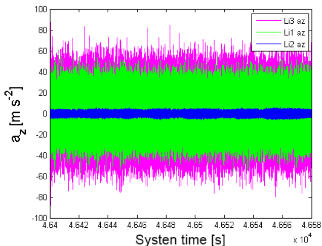
Figure 6. Time series of the accelerations in z direction of the three LI-COR sensors during a flight section of 3 min duration on 23 October 2013, illustrating the vibrations the LI-COR sensors were exposed to. The flight section took place above agricultural land at 220 m altitude. The acceleration measurements of this flight section are representative for other flight sections at different, but constant altitude. The acceleration measurements at the Li1 are shown in green, at the Li2 in blue and at the Li3 in magenta. The data were obtained during the part of the flight indicated in yellow in Fig. 3.
