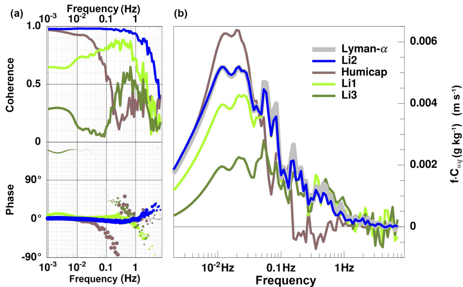
Figure 9. (a) Phase and coherence of the different LI-COR humidity sensors on the Do128 related to the Lyman-alpha sensor, with the same colour code as in Fig. 8. In the phase shift diagram, higher coherence is represented by larger dot size. (b) Cospectra of humidity from the different sensors and vertical wind speed on the Do128, multiplied by the frequency. The area under the curves is proportional to the humidity fluxes. The data are averaged over the data of the time series shaded in grey in Fig. 3.
