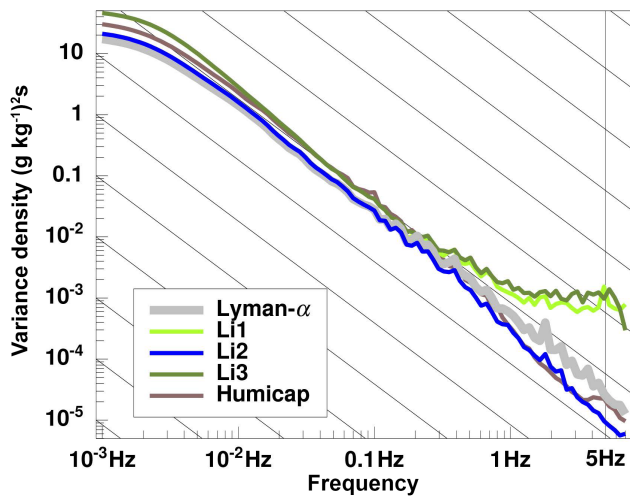
Figure 8. Power spectra (variance density) of the different humidity sensors on the Do128, Li1 in bright green, Li2 in blue, Li3 in olive, Lyman-alpha in grey and Humicap in purple. The spectra are averaged over the data of the time series shaded in grey in Fig. 3. The lines have a slope of -5/3 according to Kolmogorov theory.
