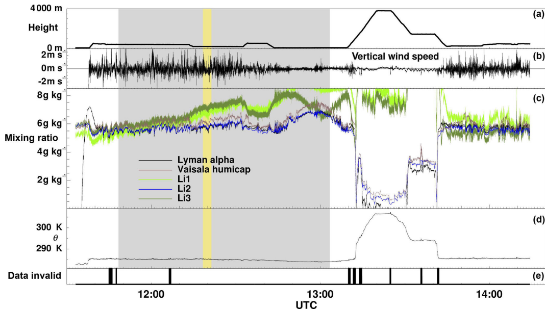
Figure 3. Overview of the flight with the Do128 on 23 October 2015. Panel (a) shows the height and (b) the vertical wind speed, indicating the strength of atmospheric turbulence. Panel (c) shows the time series of the mixing ratio measured by Lyman-alpha (black), Vaisala Humicap (purple), closed-path Li2 (blue), open-path Li1 at the nose boom (bright green) and closed-path Li3 on the cabin roof (olive). Panel (d) provides the potential temperature. Panel (e) shows the periods of invalid data, e.g. when radio communication disturbed the signals. For the spectral analysis, the part of the data shaded in grey was used, excluding segments with invalid data, e.g. disturbance from radio communication. The vibration data are analysed for the flight segment indicated in yellow.
