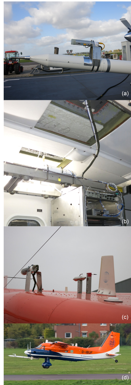
Figure 1. The three LI-COR sensors integrated into the Do128 during a humidity intercomparison flight: (a) LI7500A on the nose boom (Li1), (b) LI7200 in the cabin with an inlet near the LI-COR sensor on the roof (Li2), (c) LI7500 on the roof (Li3) and (d) the Do128 equipped with additional sensors during the flight (last photo courtesy of Uwe Bethke).
