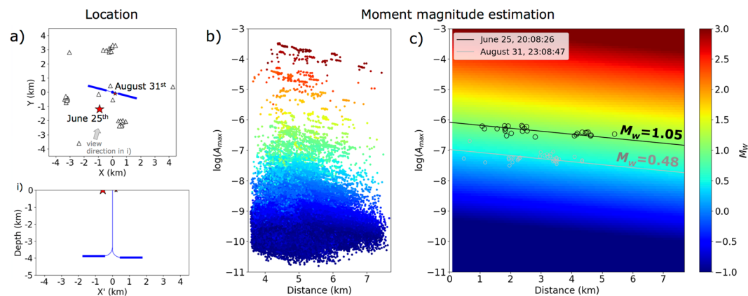
Figure 7. Location and moment magnitude ( M_w ) estimation for the two main weak events detected at the Wysin site (Method M6). (a) Map view (top) and depth section (down) displaying the located events (red stars). Stars are scaled according to the M_w estimation in (c) . Triangles show seismic stations. HF boreholes are indicated with blue lines. (b) Maximum amplitudes for each source and each station plotted against hypocentral distance for the complete synthetic catalogue generated in previous work 26 . (c) M_w estimation using a domain extrapolation defined from the microseismic synthetic catalogue in (b) . Black and gray dots show maximum amplitudes observed at all seismic stations for the two events displayed in (a) . Black and grey lines represent the M_w estimation for both events (see legend).
