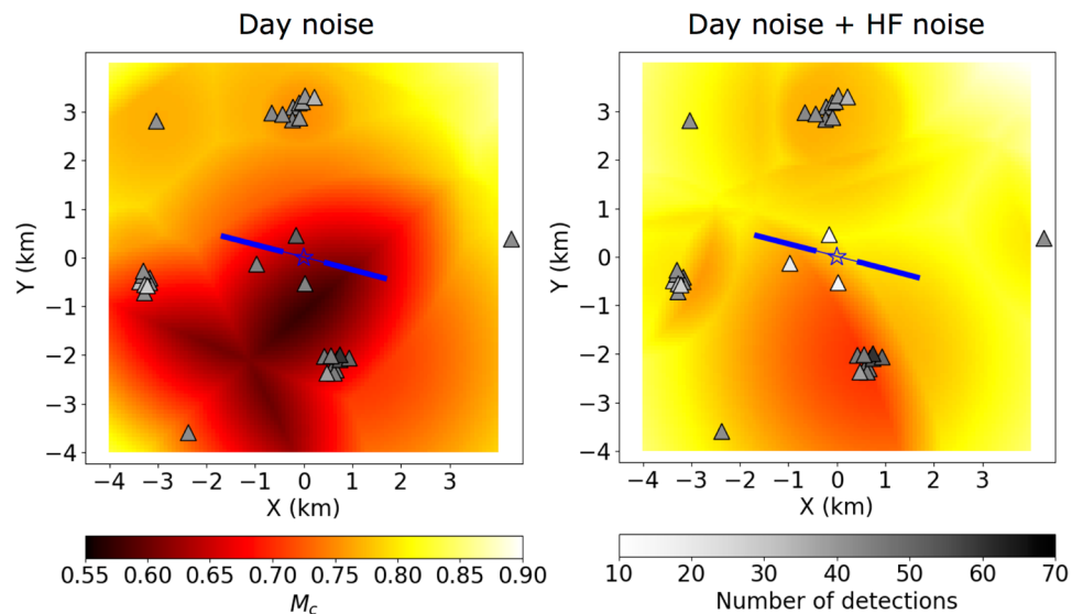
Figure 4. Spatial monitoring performance at Wysin site in terms of magnitude of completeness using an amplitude threshold approach estimated from noise recording before HF operations during day hours (left) and, in addition, considering the noise amplitude increase during the HF operations (right). Grey color scale identifies the number of synthetic events detected for each station (see technical details 26 ). Star shows the HF area (vertical drilling) and blue lines indicate the horizontal HF drillings.
