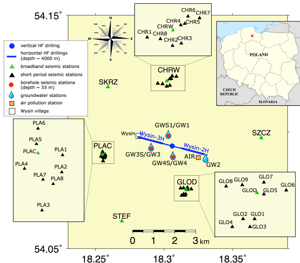
Figure 1. Map of seismic, air and groundwater monitoring at the Wysin site (Poland). The seismic monitoring includes broad-band stations (green triangles), small-scale arrays (inset boxes) composed by 8–9 short-period stations each (black triangles), and borehole stations (red circles). The air pollution station (orange square) is located at Stary Wiec village. Groundwater borehole monitoring stations are denoted by water drop symbols; some of them are located next to the borehole seismic stations. Wellhead (blue dot) and horizontal boreholes (blue lines) are shown. The inset map shows the hydraulic fracturing area (red square) in Poland. The map was created using the free software GMT Version 4.5.16 Released ( https://www.soest.hawaii.edu/gmt/ ) and finished with the free software LibreOffice Version 4.3.3.2 Released ( https://www.libreoffice.org ).
