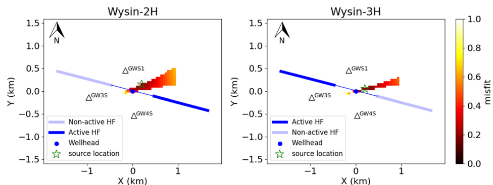
Figure 3. Location of SNAI (green open stars) through the modelling of amplitude decay during the HF stimulations at Wysin-2H (left) and Wysin-3H (right). Borehole stations are shown with black open triangles. We only assess the misfit in those grid points for which we observe the following amplitude relation: A_{\text{GWS1}} > A_{\text{GW4S}} > A_{\text{GW3S}} (Method M3).
