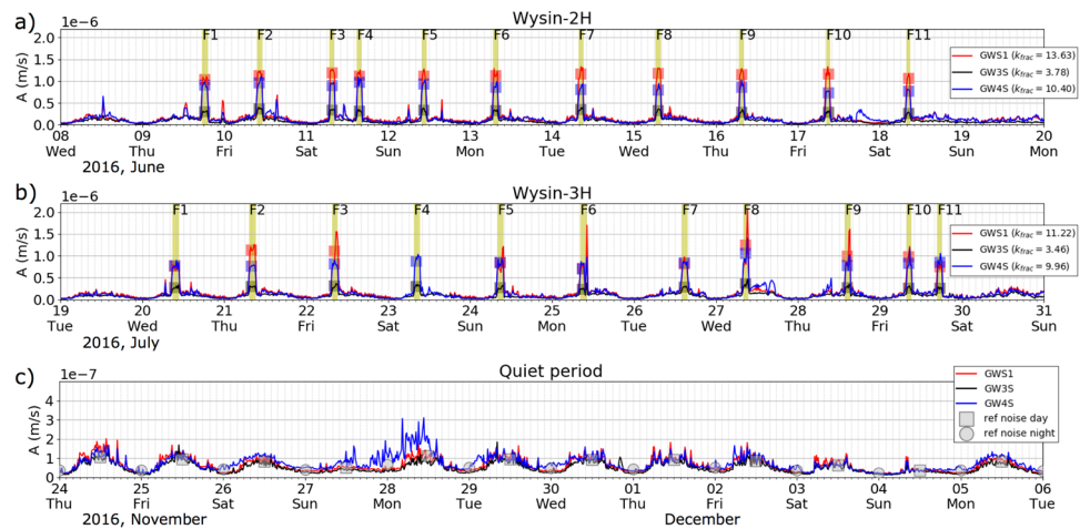
Figure 2. Average absolute amplitude of seismic signals is calculated every 15 min at borehole stations, applying a bandpass filter between 2 and 15 Hz. Three different time intervals of 12 days are considered: (a) HF stimulations at Wysin-2H, (b) HF stimulations at Wysin-3H and (c) quiet period after the end of all HF operations. Amplitude is normalized to velocity units removing the instrument response. Yellow bands indicate the SNAI duration associated with the frac stages (F1 to F11). Red, black and blue squares show the average amplitude during each frac stage for the borehole stations GWS1, GW3S and GW4S respectively. SNAI ratios ( k_{\text{frac}} ) for each sensor is shown in the legend (see Method M2). The average amplitudes according the diurnal variation between 6:00 and 18:00 h are shown for day hours (gray squares) and night hours (gray circles). Time marks are at 2-hr intervals.
