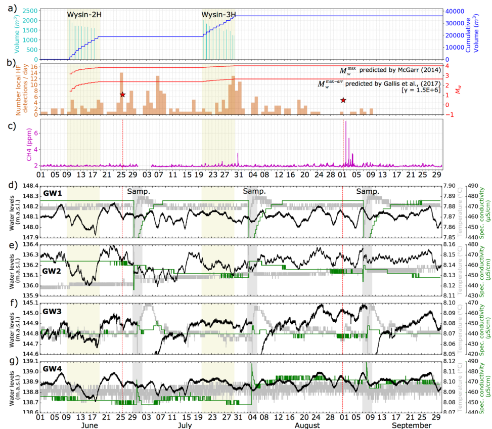
Figure 8. Correlation among fluid volumes injected, seismicity, air pollution and groundwater conditions for 4-month period involving different stages before, during and after the termination of HF stimulations. Yellow bands indicate the 10-days period for the HF stimulations at the Wysin-2H and Wysin-3H. Time marks are at 1-day intervals. (a) Fluid volumes injected in each frac stage and the cumulative volume. (b) Distribution of local HF detections per day (left axis) and the located events with M_w (red stars, right axis). The maximum magnitude 39,40 is also shown (red line). (c) Methane content ( CH_4 ) in ppm. (d–g) Water levels, temperature and specific conductivity (black, gray and green line, respectively) for each groundwater borehole. Note the same height is shown in y-axes for the water level (0.5 m), temperature (0.05 °C) and specific conductivity (50 \mu S/cm). Gray bands (so-called Samp.) indicate groundwater-sampling periods where any changes of the groundwater parameters result from groundwater sampling. Vertical red dashed lines in (c) to (g) indicate the time of the largest seismic events according the red stars in (b) .
