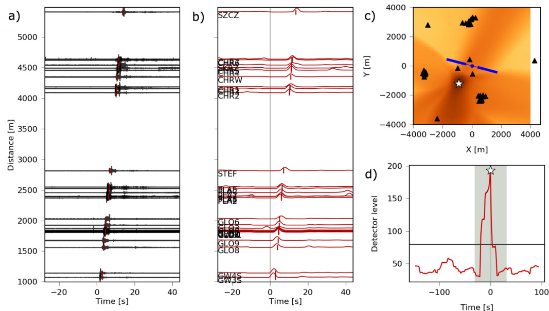
Figure 6. Hypocentral location on 2016 June 25 th , 20:08:26 UTC time (Method M5). (a) Waveforms sorted by hypocentral distance. (b) Characteristic function (normalized amplitude envelopes) for each trace. These are used for travel–time stacking corrected with S-wave speed (red lines). The markers indicate the (best fit) synthetic arrival time of the S-phase at each sensor. (c) Coherence (stack) map for the search region. Dark colors denote high coherence values. A white star marks the location of the detected event. Sensor locations are shown with black triangles. (d) Global detector level function in a processing time window from -20 to 20 s around the origin time of the detected event. The cutout time window used for the coherence map is shown in gray color. White star indicates the detection exceeding a detector level threshold of 80.
