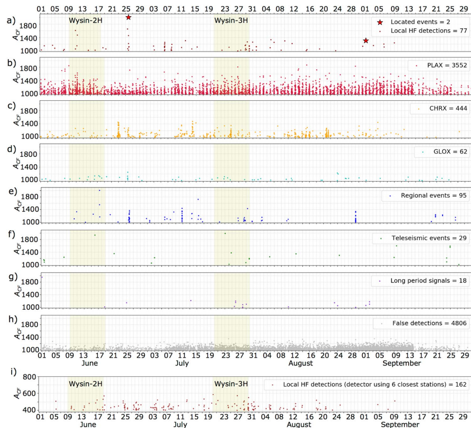
Figure 5. Detection and classification of seismic signals before, during and after the HF operations at the Wysin site. Each detection is identified by the time and the maximal coherence ( A_{cf} ) obtained from Lassie detector (Method M4). The dataset has been classified manually according different categories (see legend in each box). Yellow bands indicate the 10-days period for the HF stimulations in Wysin-2H and Wysin-3H. Time marks are at 1-day intervals.
