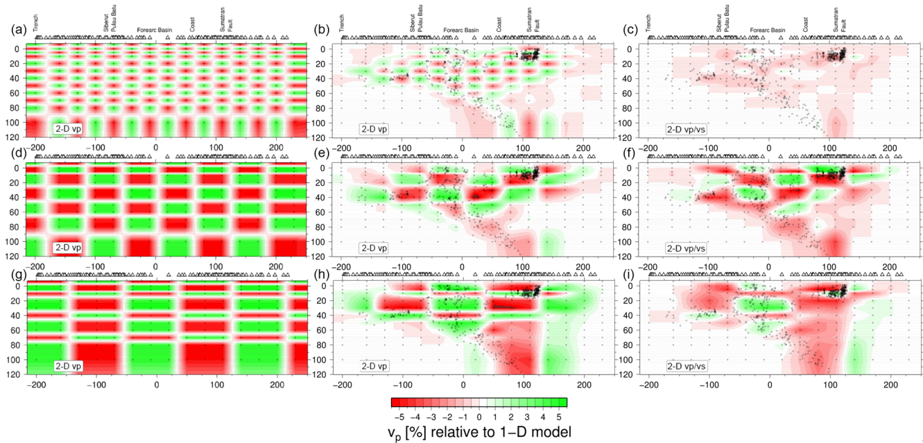
Figure 5. 2-D synthetic checkerboard models with 5 % velocity perturbation input anomalies ( a , d , g ), the inversion restoration for v_p ( b , e , h ) and v_p/v_s ( c , f , i ) models. Crosses represent nodes used in the inversion and the reconstructions are plotted with the resulting hypocenter locations (black points). We calculated different checkerboard inversions using 1 \times 1 and 2 \times 2 (shown in the rows from top to bottom) grid node model perturbations. Noise was added to the synthetic data depending on the quality of the arrivals.
