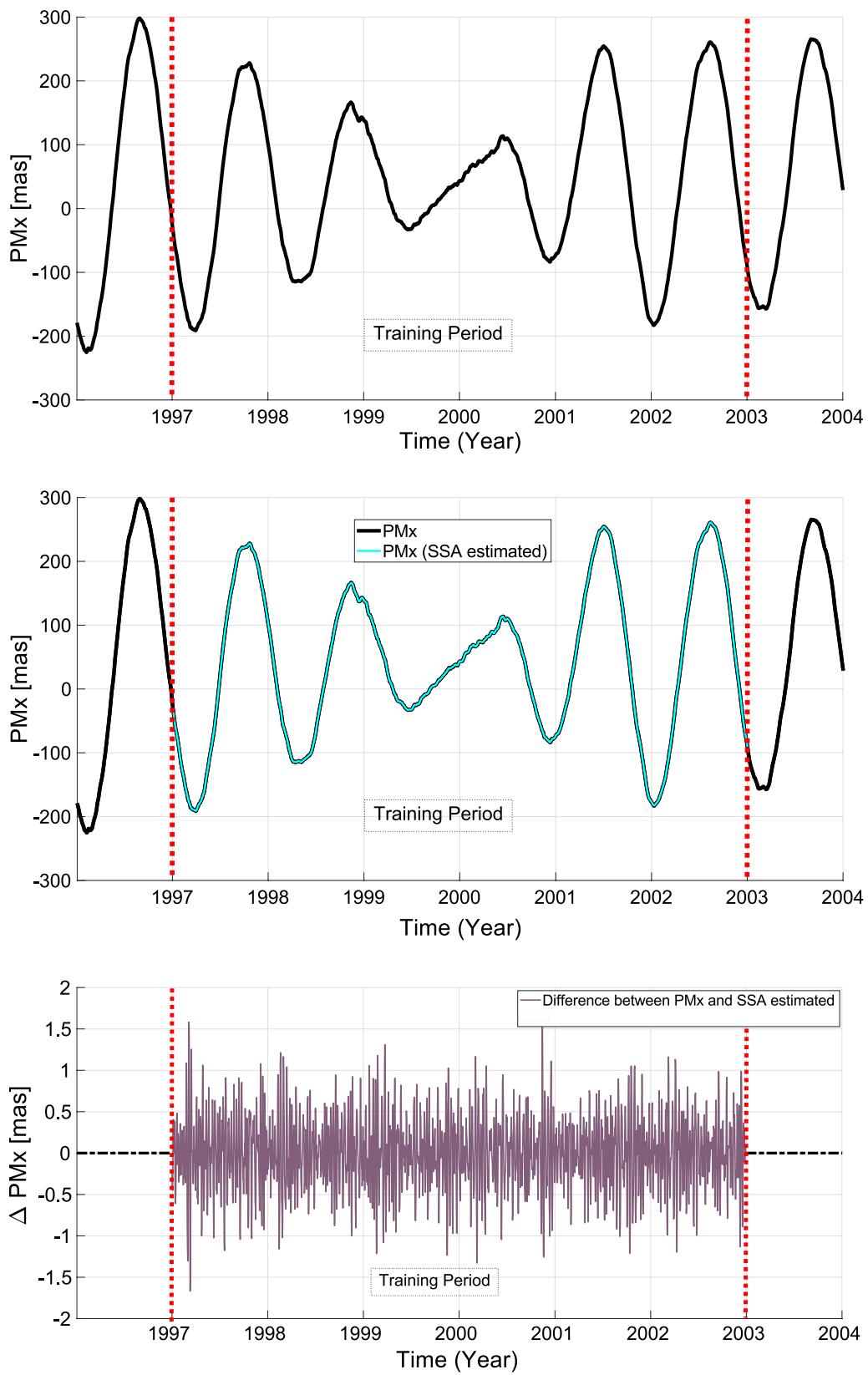
Fig. 8 The original time series (upper panel), the reconstructed time series (middle panel), and the difference between original and reconstructed time series (lower panel) for PM_x
