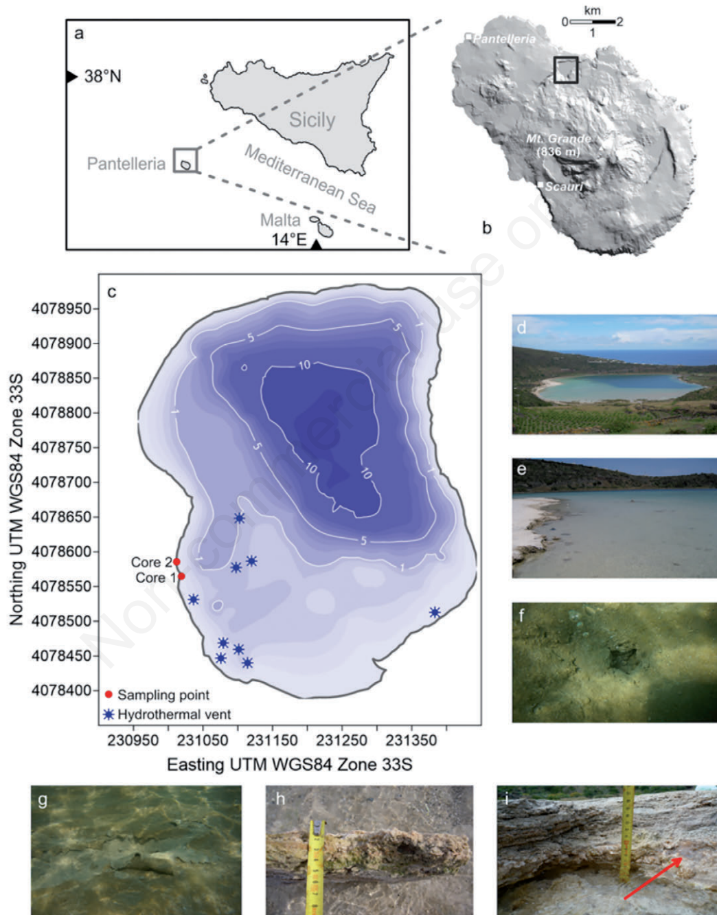
Fig. 1. Studied area: a) location of Pantelleria Island; b) location of Lake Specchio di Venere; c) bathymetric contour lines (m bl) and location of sampling points (red circles) and hydrothermal vents (blue stars); d) overview of Lake Specchio di Venere; e) view of the southwestern sector of the lake showing the carbonate bank (on the left in the picture); f) submerged hydrothermal vent emitting CO 2 bubbles; g) microbial mats wrapping the unconsolidated sediments of the lake floor; h) siliceous stromatolites; i) sampling point (core 1) showing the roughly laminated structure of the bank with associated silica gel deposit (red arrow).
