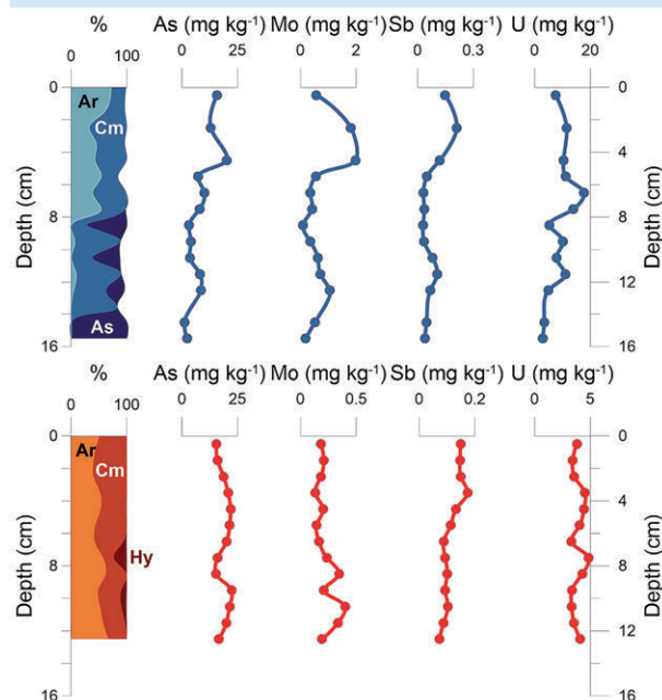
Fig. 5. Top: vertical variations of abundance (%) of aragonite (Ar), clay minerals (Cm) and amorphous silica (As) compared with As, Mo, Sb and U concentrations in core 1. Bottom: vertical variations of abundance (%) of aragonite (Ar), clay minerals (Cm) and hydromagnesite (Hy) compared with the same elements in core 2.
