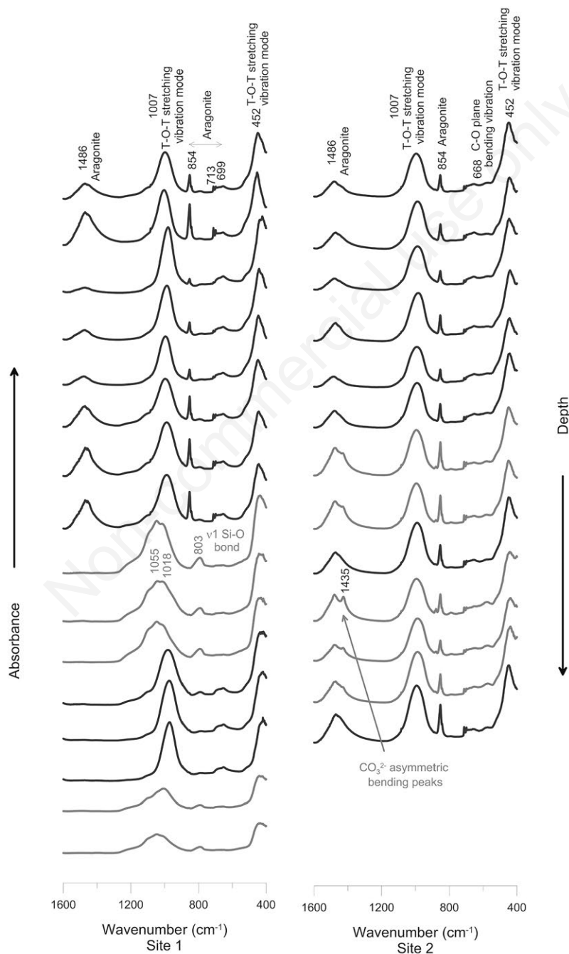
Fig. 2. FTIR spectra of core 1 and 2 in the low frequency region (400-1600 \text{cm}^{-1} ).
