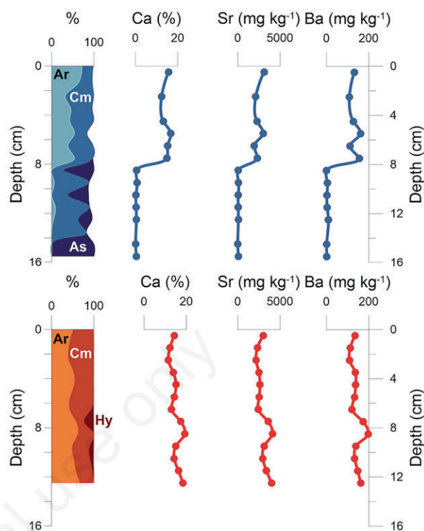
Fig. 4. Top: vertical variations of abundance (%) of aragonite (Ar), clay minerals (Cm) and amorphous silica (As) compared with Ca, Sr and Ba concentrations in core 1. Bottom: vertical variations of abundance (%) of aragonite (Ar), clay minerals (Cm) and hydromagnesite (Hy) compared with the same elements in core 2.
